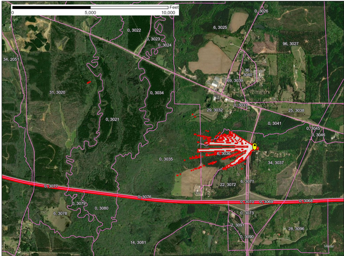
Figure 1 – Tremont, MS SAN -77.6 dB(mW/(m2 * MHz)) pfd contour
