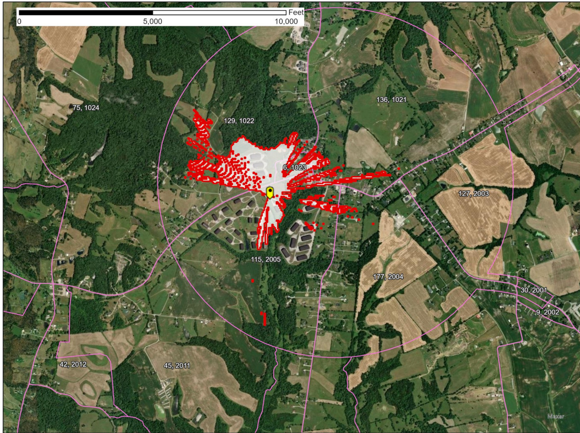
Figure 1 – Loretto, KY SAN -77.6 dB(mW/(m2 * MHz)) pfd contour
