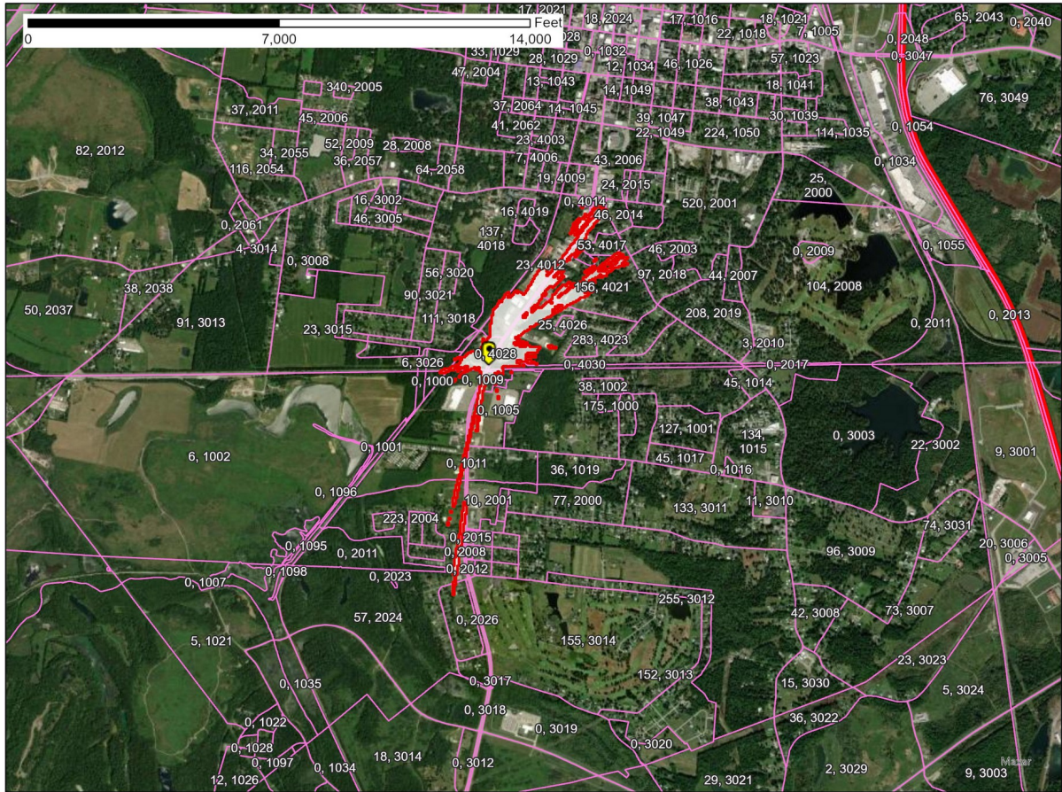
Figure 1 – Madisonville, KY SAN -77.6 dB(mW/(m2 * MHz)) pfd contour
