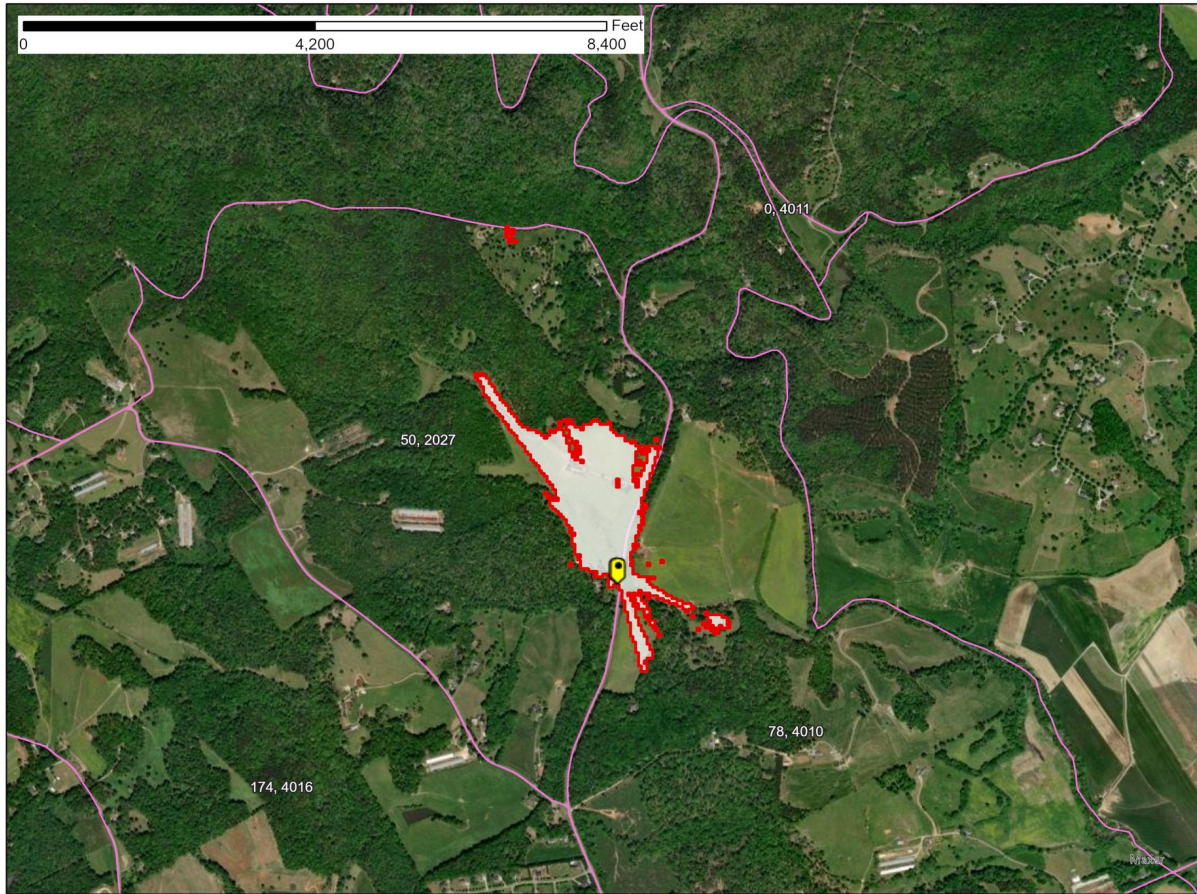
Figure 1 – Clarkesville, GA SAN -77.6 dB(mW/(m2 * MHz)) pfd contour
