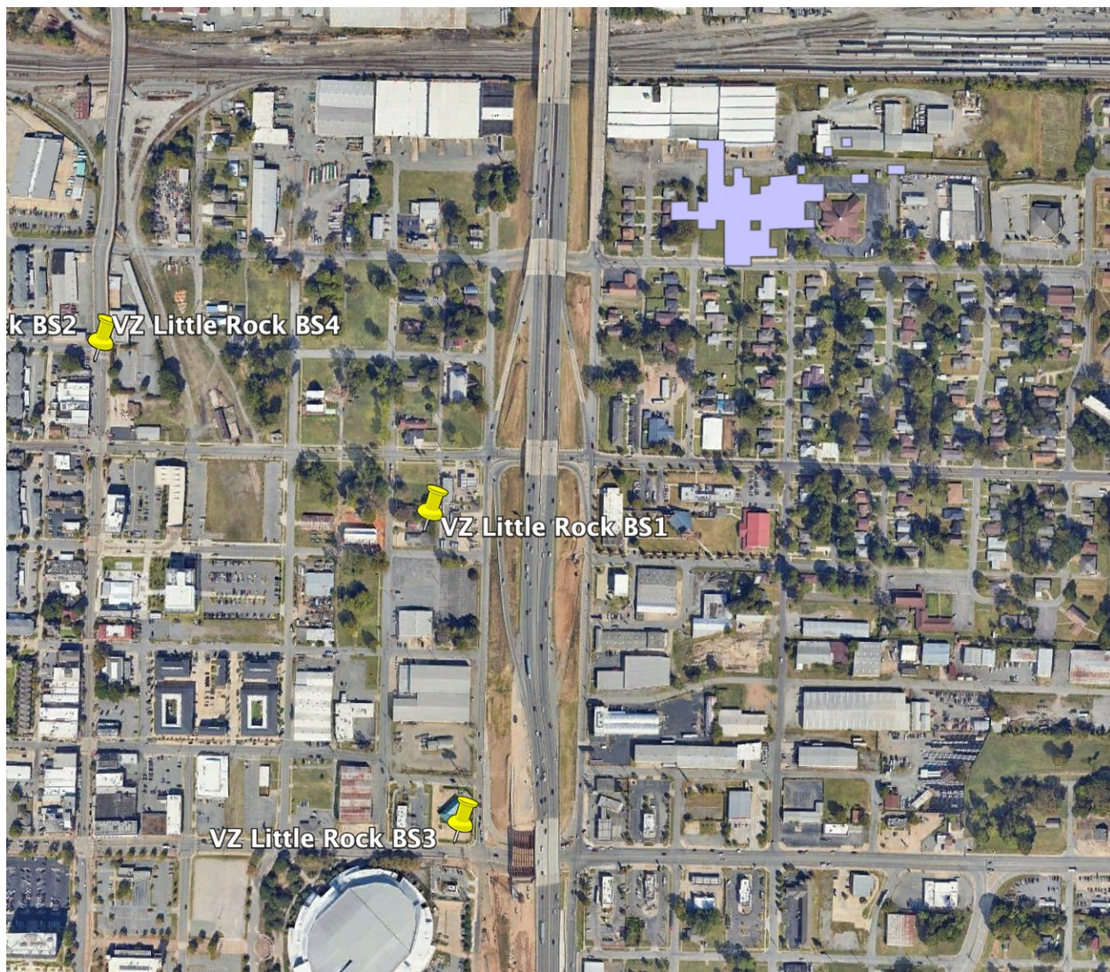
Figure 3 - North Little Rock, AR SAN -77.6 dB(mW/(m 2 * MHz)) pfd contour with Verizon BS in Yellow Pins
