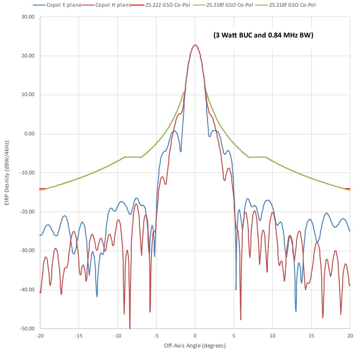
H90 Transmit Azimuth 14.25 GHz Copol EIRP
