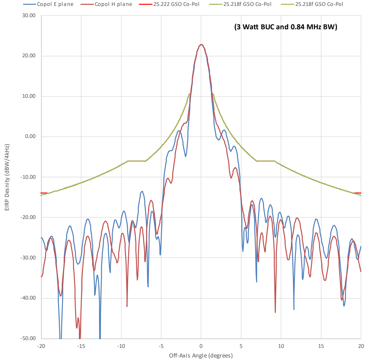
H90 Transmit Azimuth 14.50 GHz Copol EIRP
