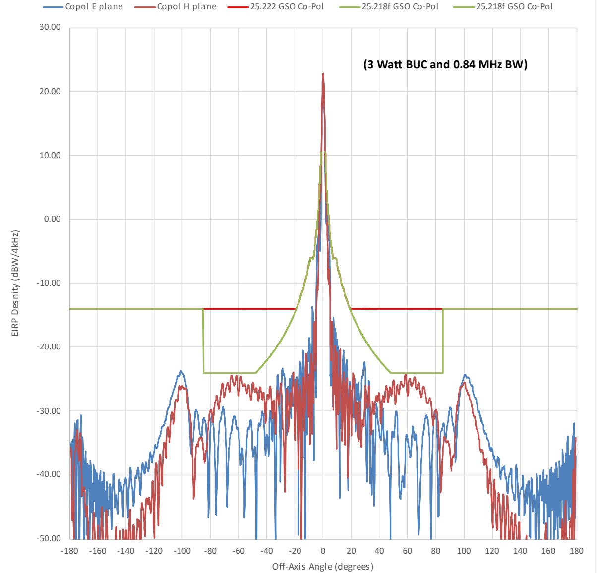
H90 Transmit Azimuth 14.50 GHz Copol EIRP
