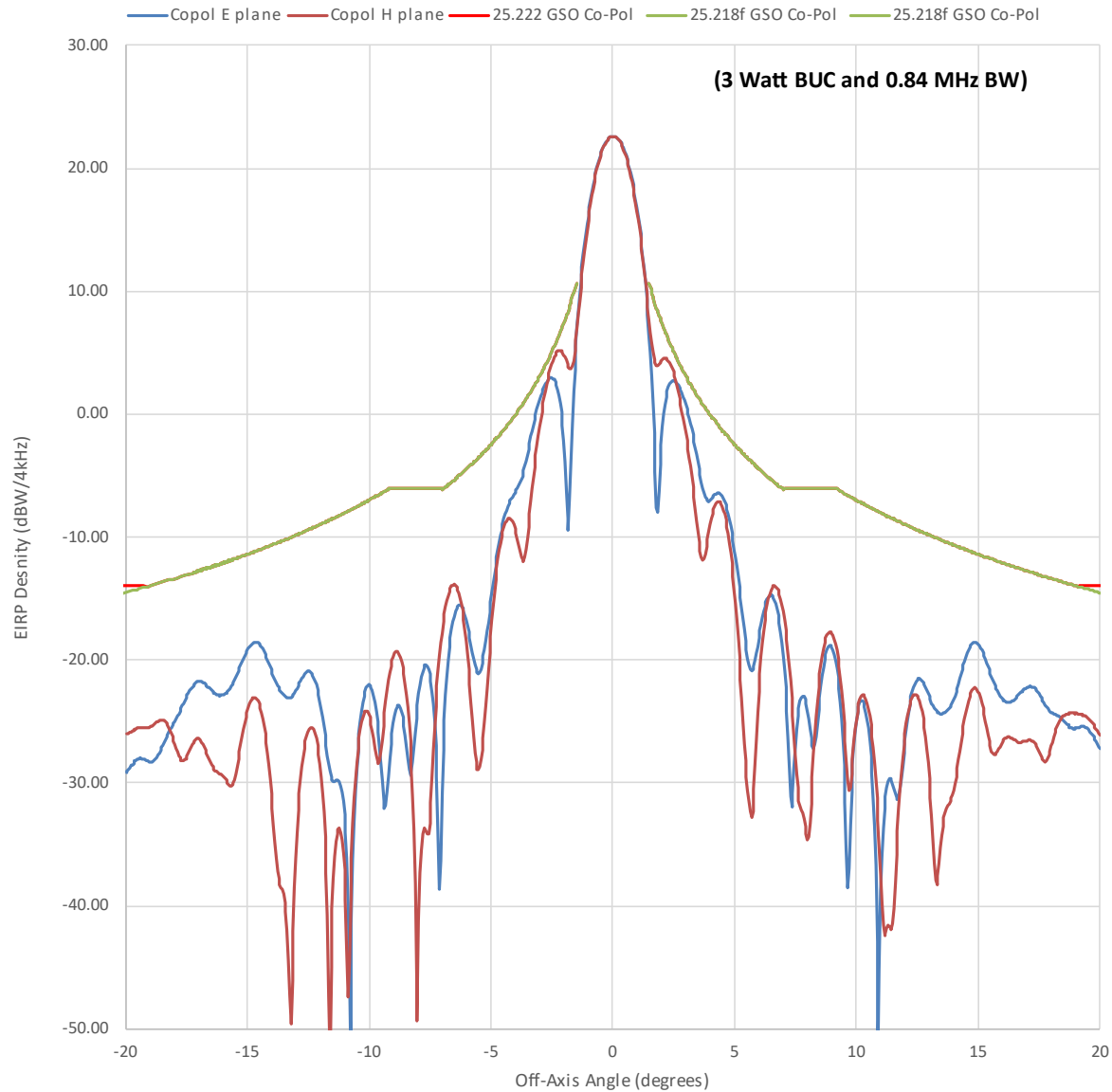
H90 Transmit Azimuth 14.00 GHz Copol EIRP
