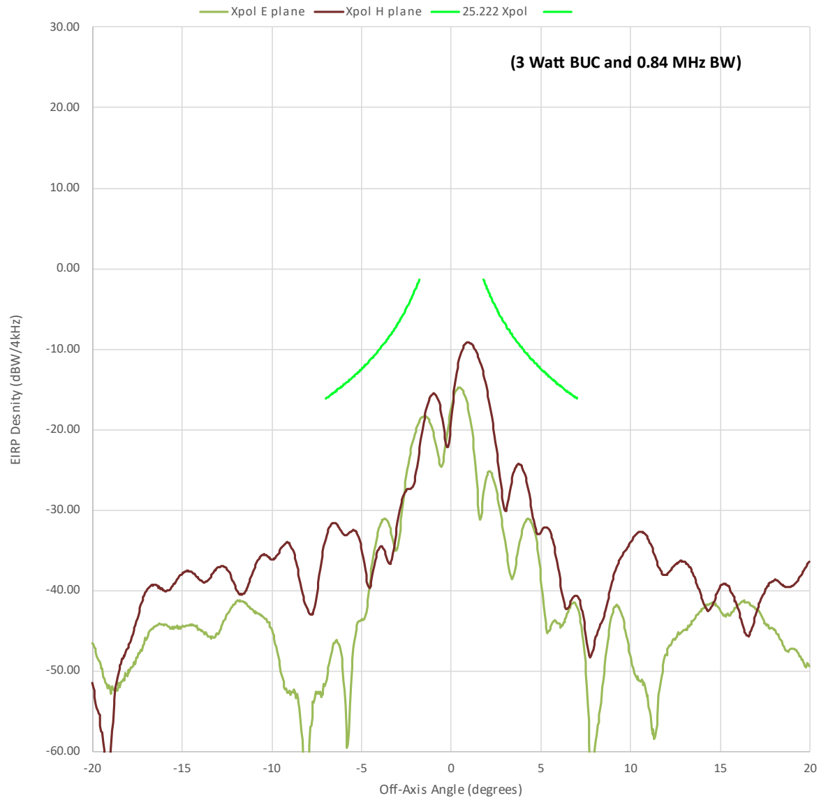
H90 Transmit Azimuth 14.25 GHz Xpol EIRP
