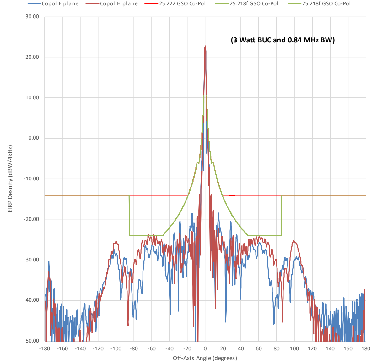
H90 Transmit Azimuth 14.00 GHz Copol EIRP
