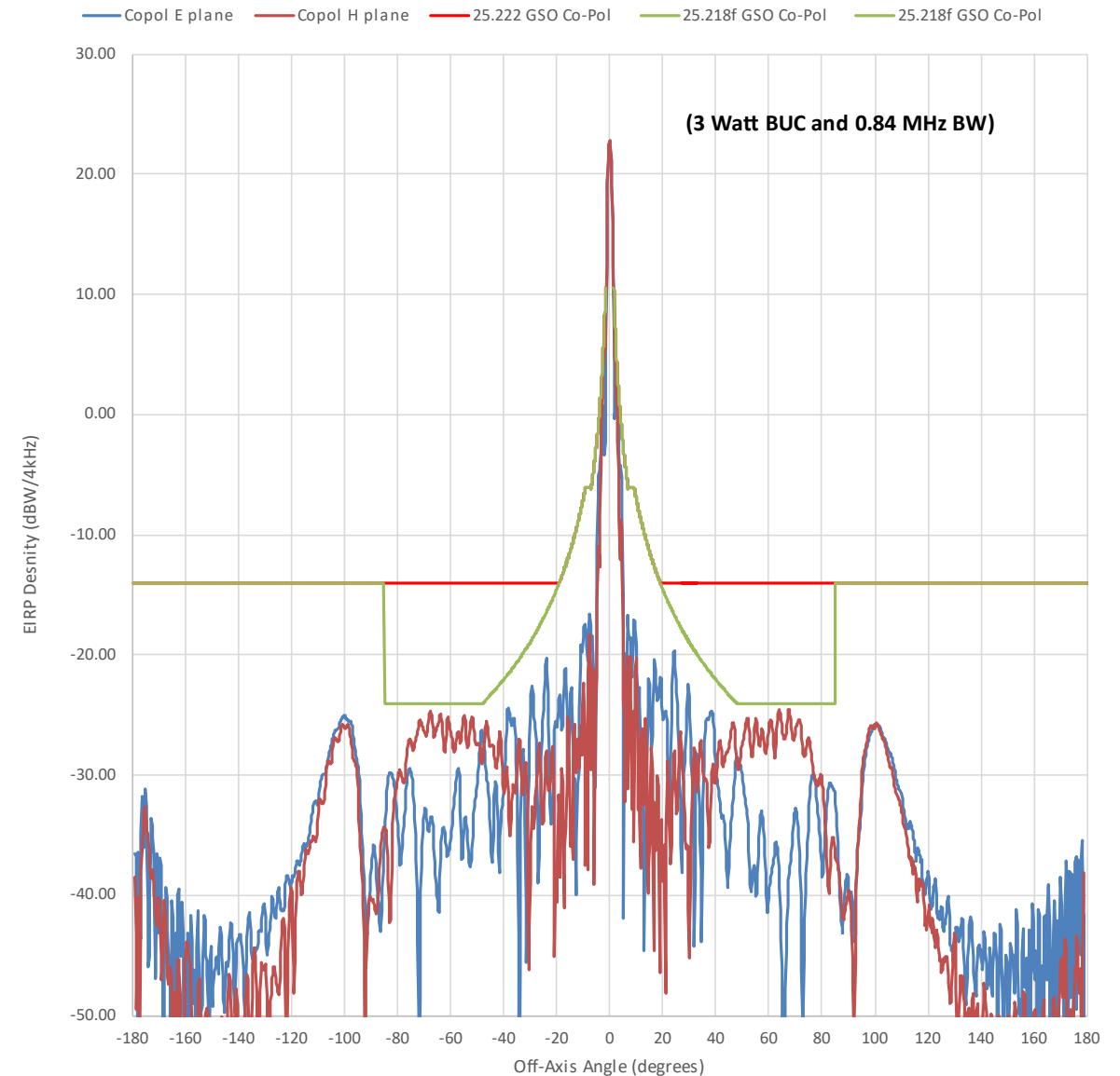
H90 Transmit Azimuth 14.25 GHz Copol EIRP
