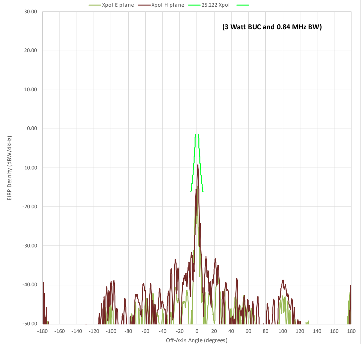
H90 Transmit Azimuth 14.25 GHz Xpol EIRP
