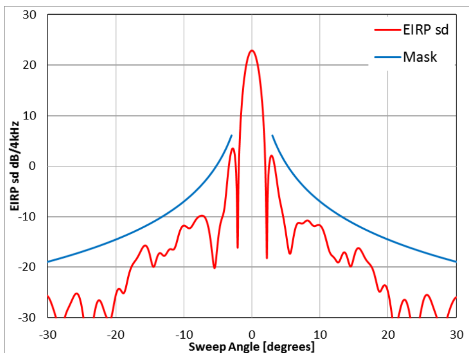
14.25GHz EIRP spectral density @ -18.08 dBW/4kHz Input power spectral density
