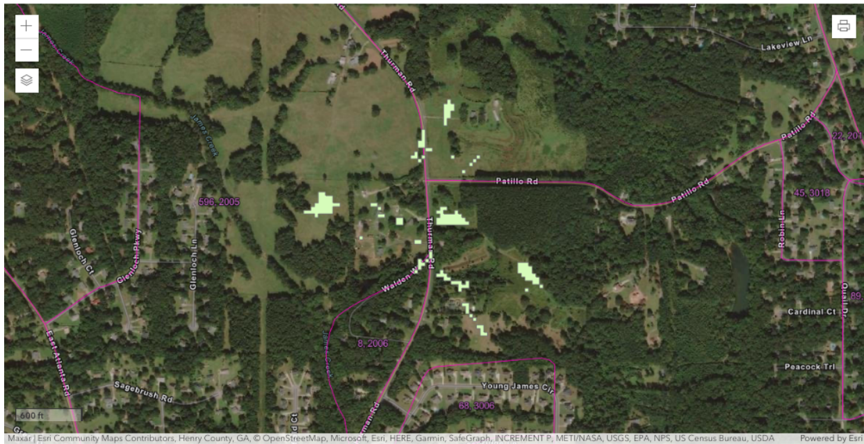
Figure 2 – E160131 earth station -77.6 dB(mW/(m 2 * MHz)) pfd contour
