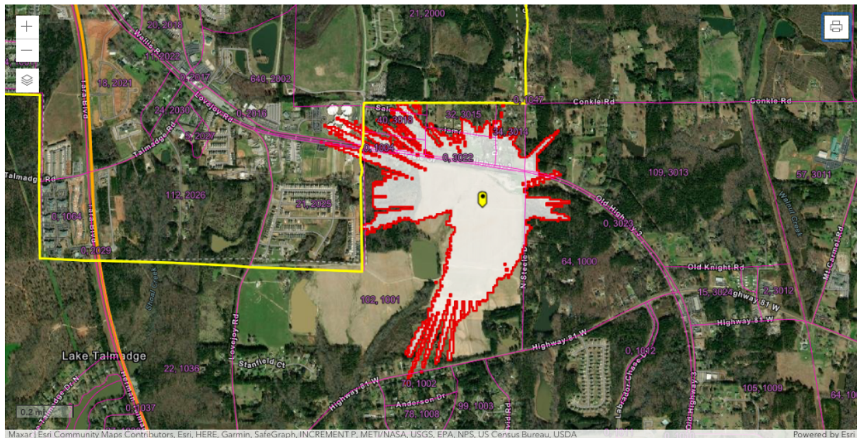
Figure 1 – Hampton, GA SAN -77.6 \text{ dB(mW/(m}^2 * \text{ MHz))} pfd contour
