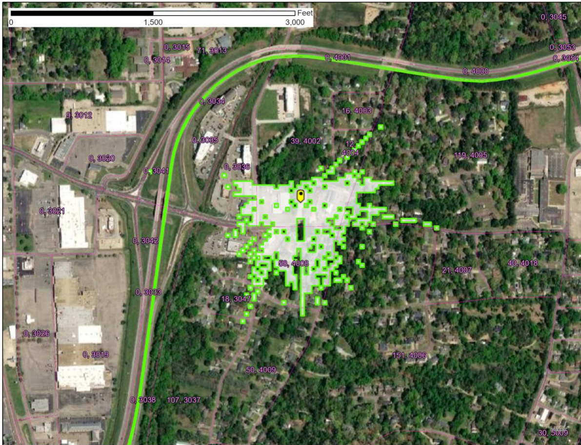
Figure 1 – Columbus, MS SAN -77.6 \text{ dB(mW/(m}^2 * \text{ MHz))} pfd contour
