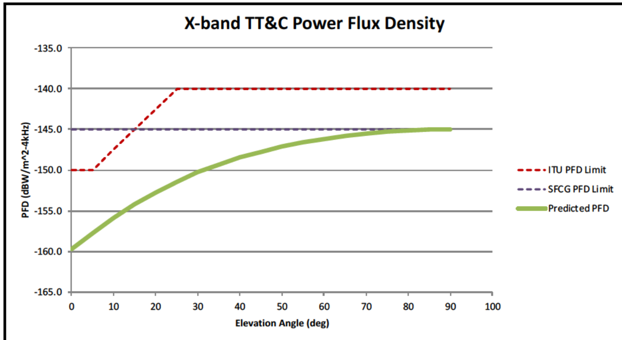
Figure VII.A-2. Capella X-Band TT&C downlink PFD at Earth's surface (worst-case altitude)
