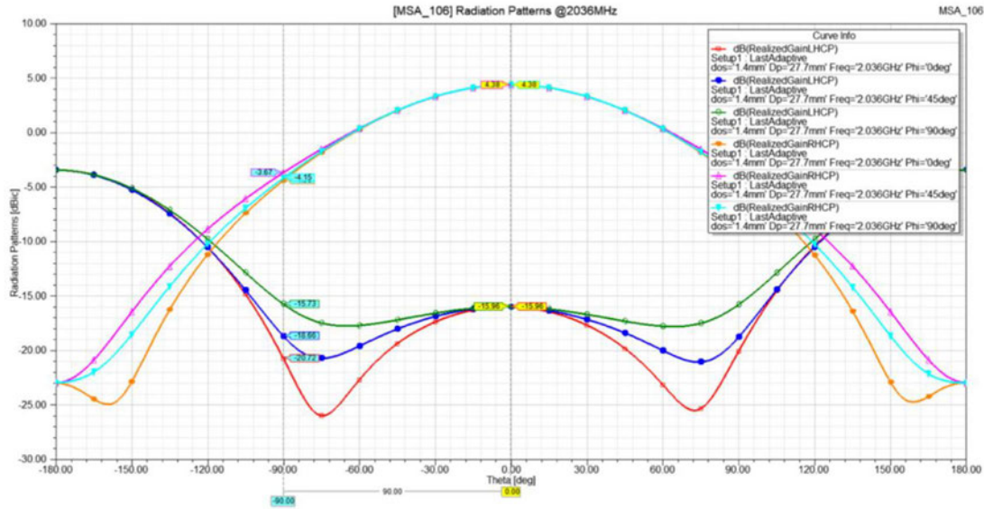
Figure V.C-1. Capella S-Band TT&C Uplink Gain Pattern
