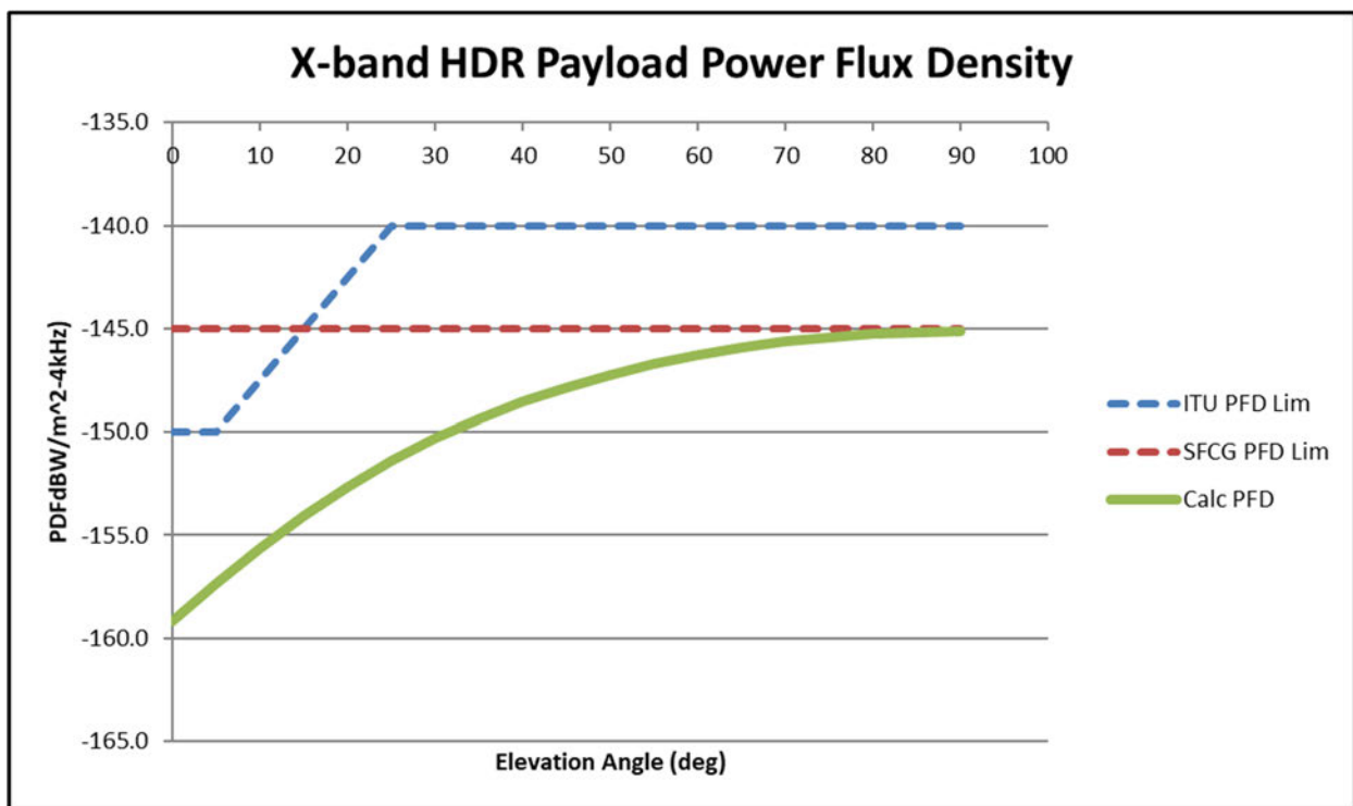
Figure VII.A-1. Capella X-Band payload downlink PFD at Earth’s surface (worst-case altitude)
