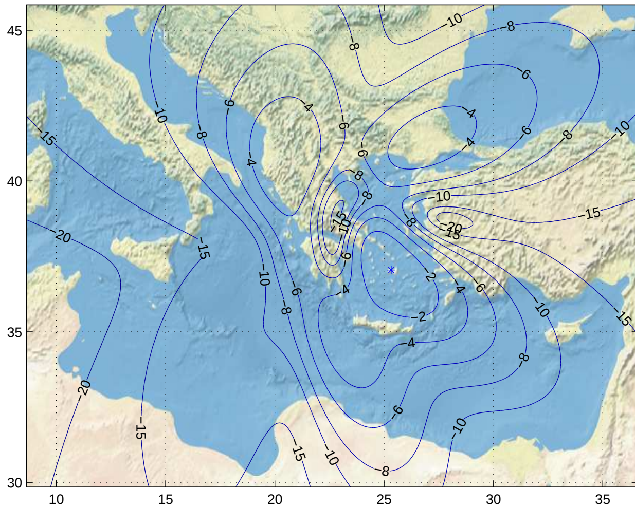
Gain Contours at 385km for ATH. Beam ID=URC, Polarization=h
