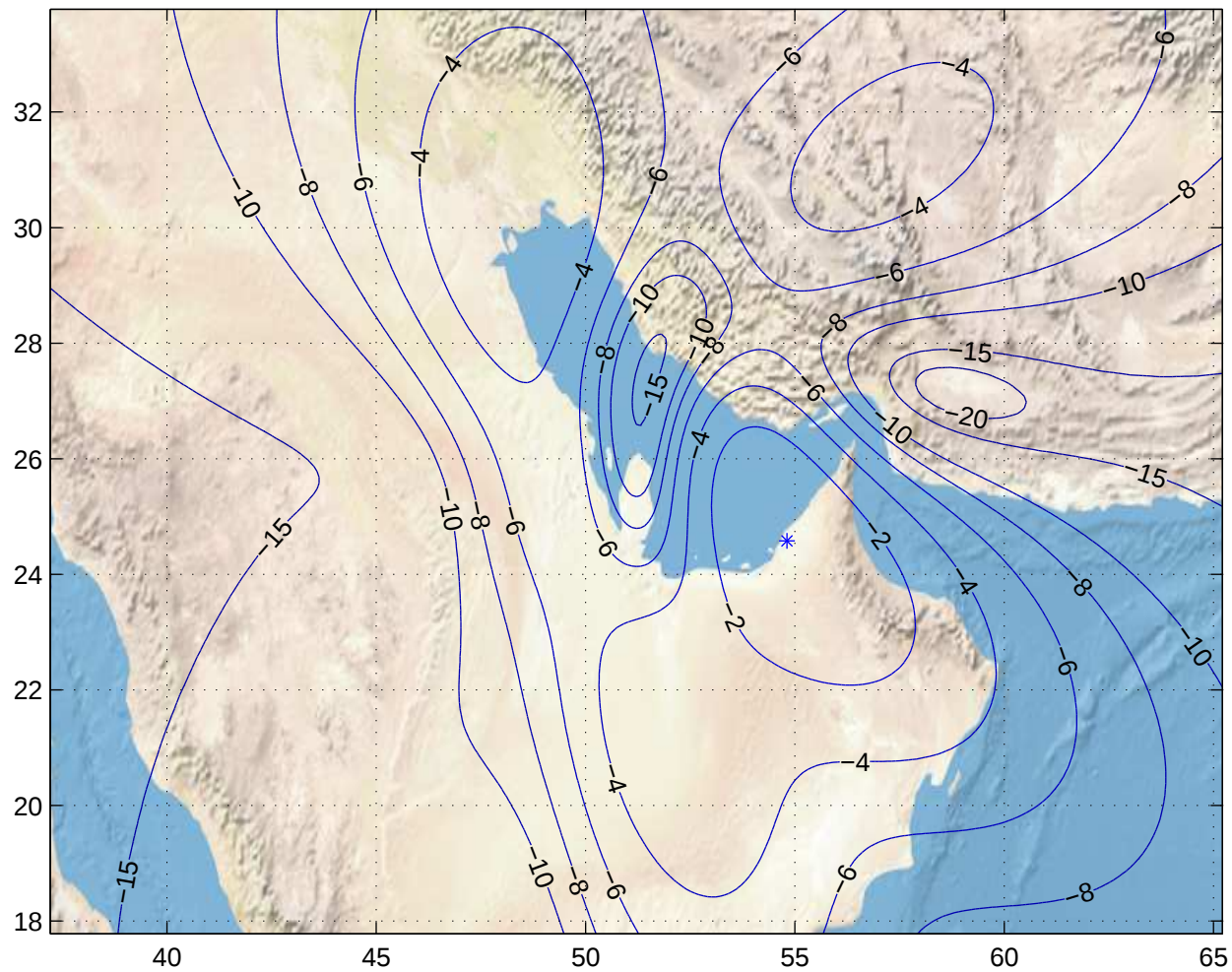
Gain Contours at 600km for DOH. Beam ID=URC, Polarization=h
