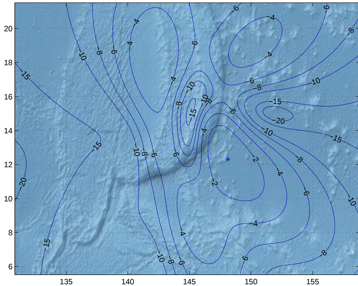
Gain Contours at 600km for GUM. Beam ID=URC, Polarization=h
