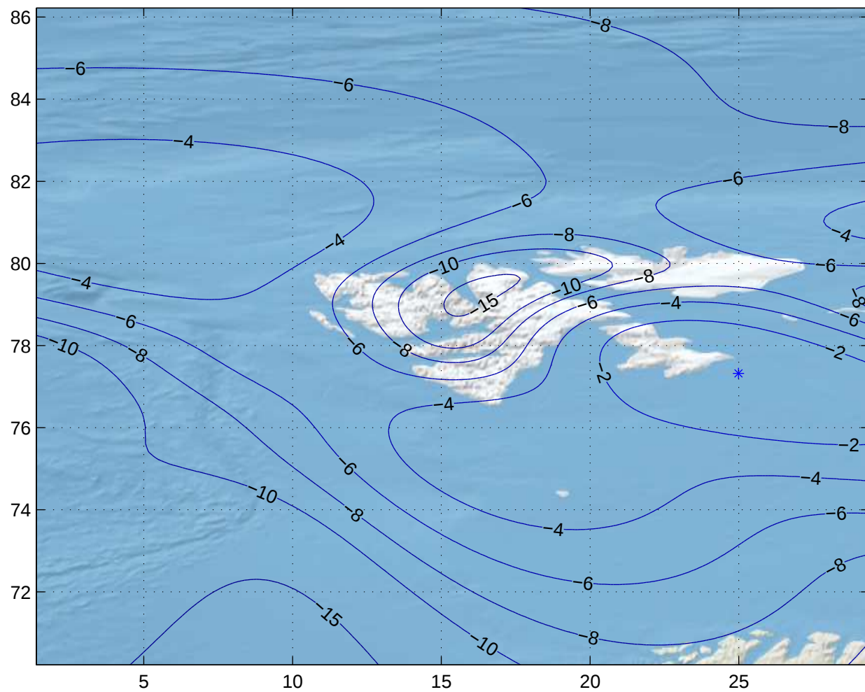
Gain Contours at 385km for LVR. Beam ID=URC, Polarization=h
