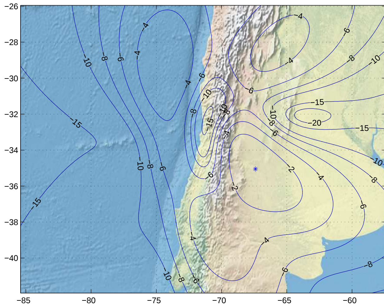
Gain Contours at 600km for SCL. Beam ID=URC, Polarization=h
