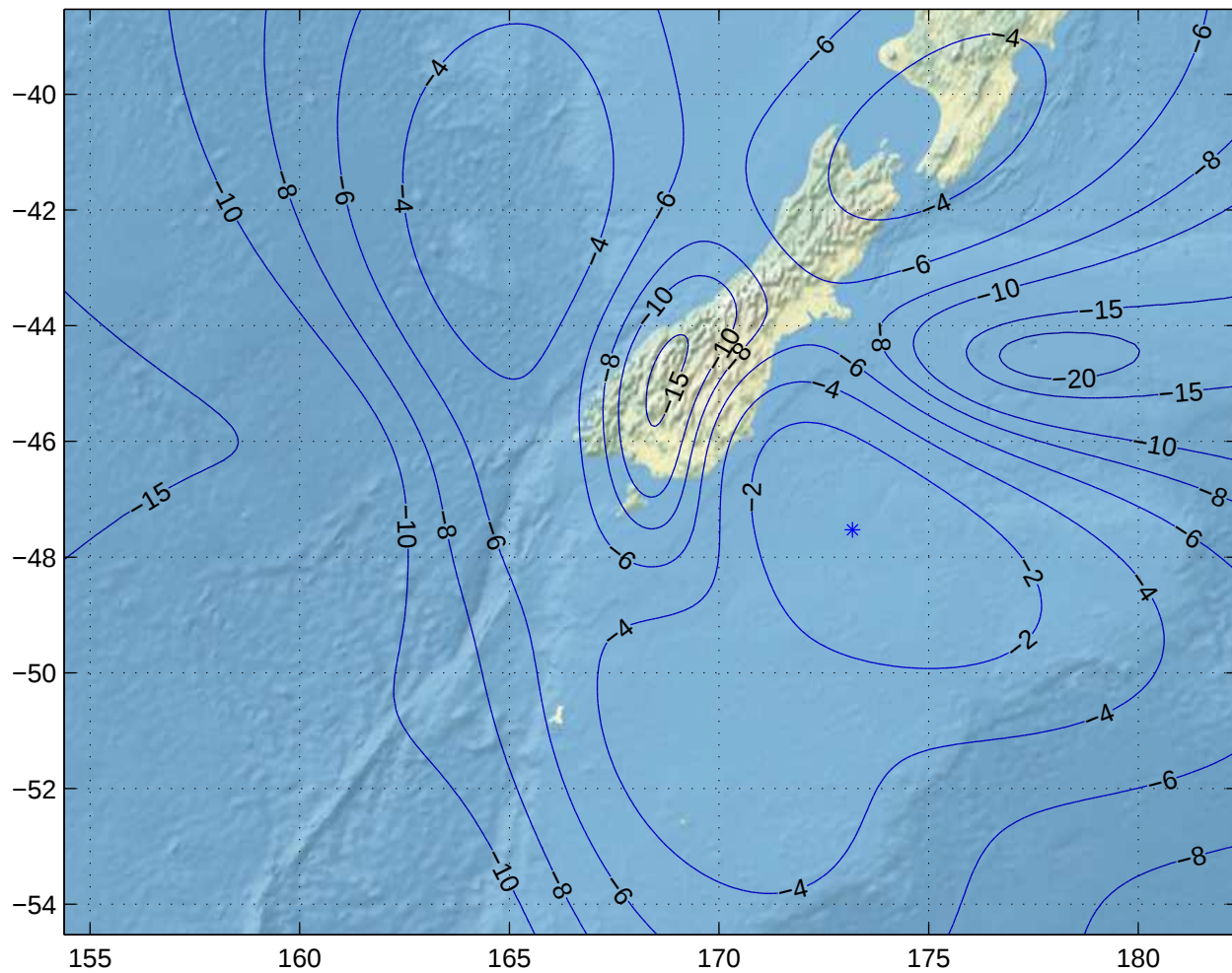
Gain Contours at 600km for IVC. Beam ID=URC, Polarization=h
