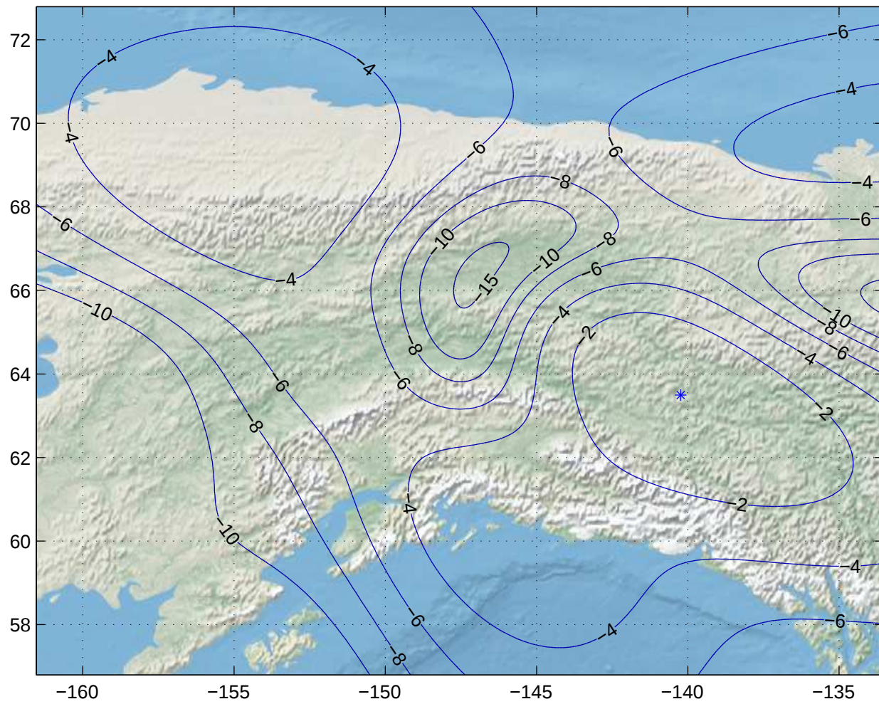
Gain Contours at 600km for FAI. Beam ID=URC, Polarization=h
