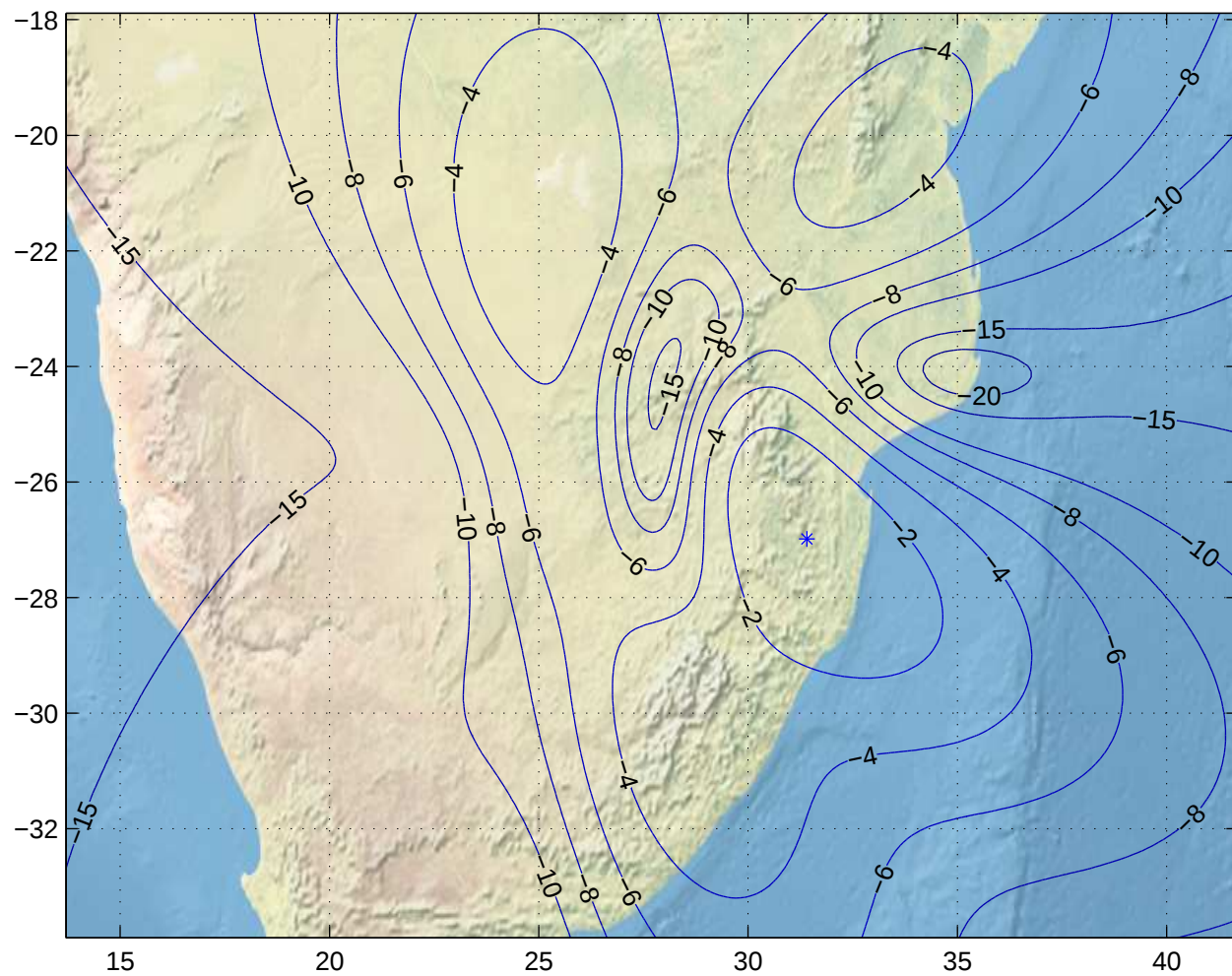
Gain Contours at 600km for JNB. Beam ID=URC, Polarization=h
