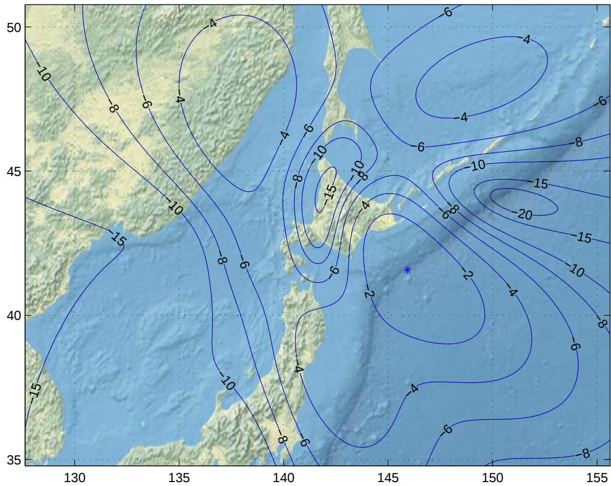
Gain Contours at 600km for CTS. Beam ID=URC, Polarization=h
