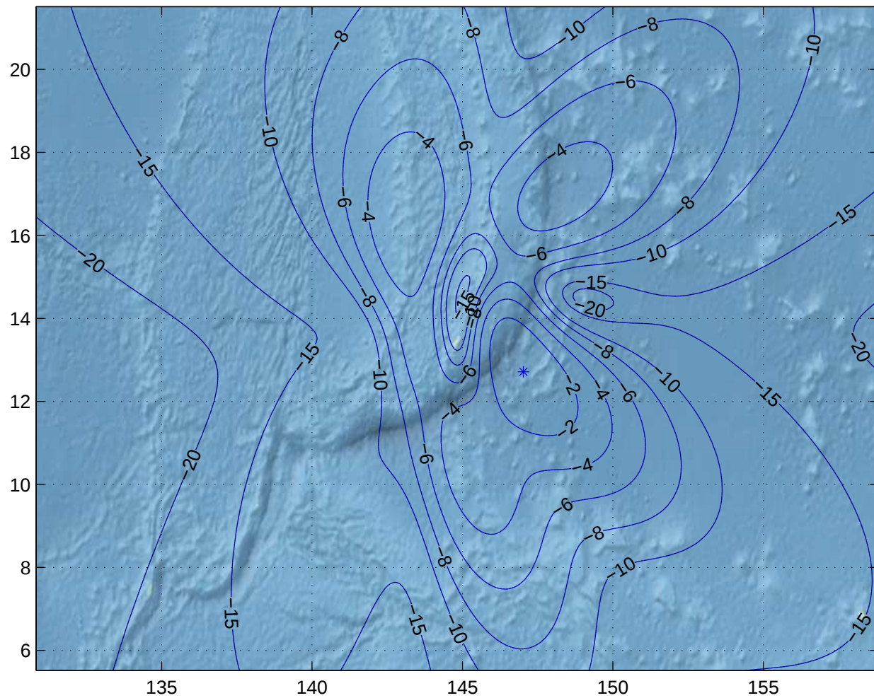
Gain Contours at 385km for GUM. Beam ID=URC, Polarization=h
