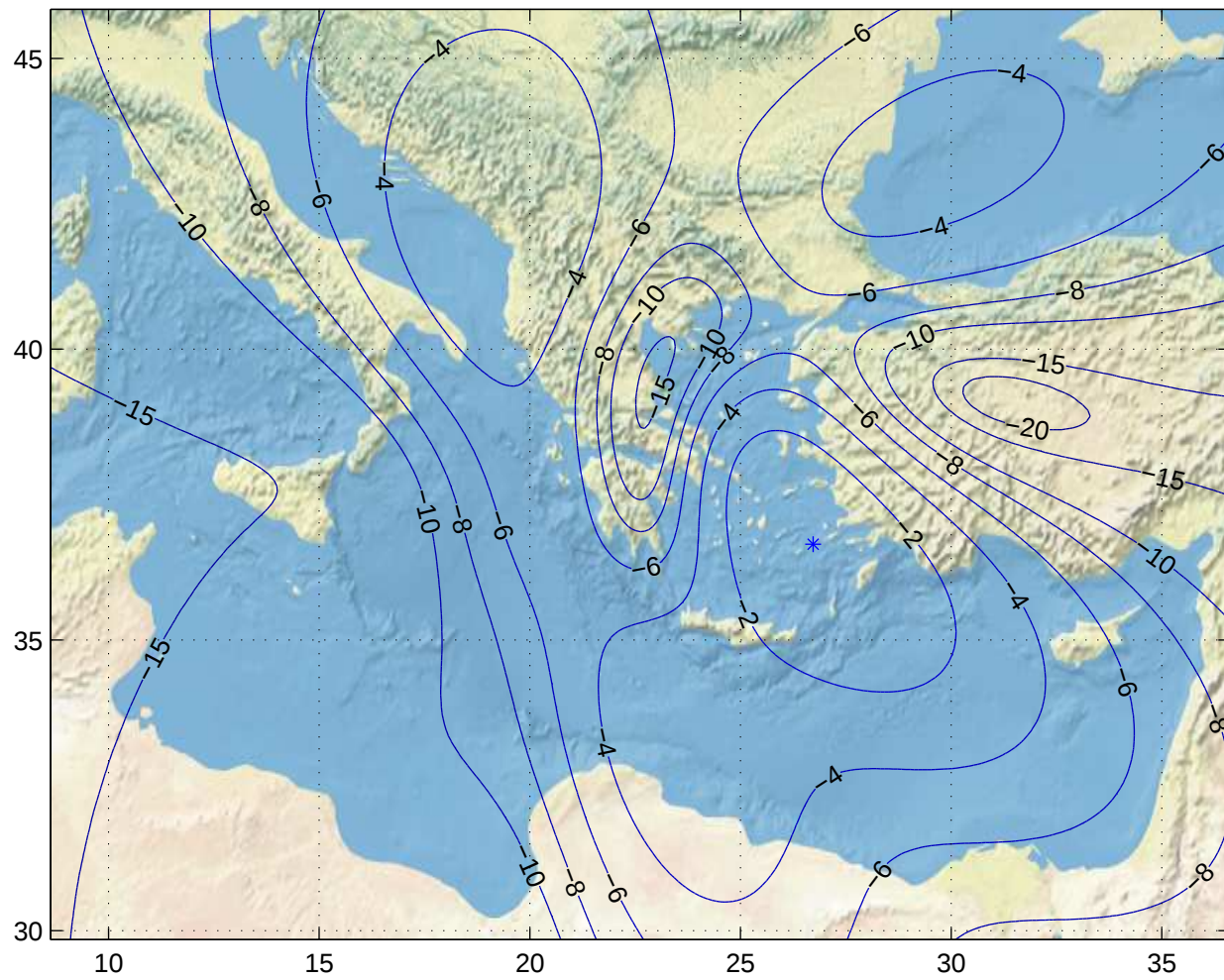
Gain Contours at 600km for ATH. Beam ID=URC, Polarization=h
