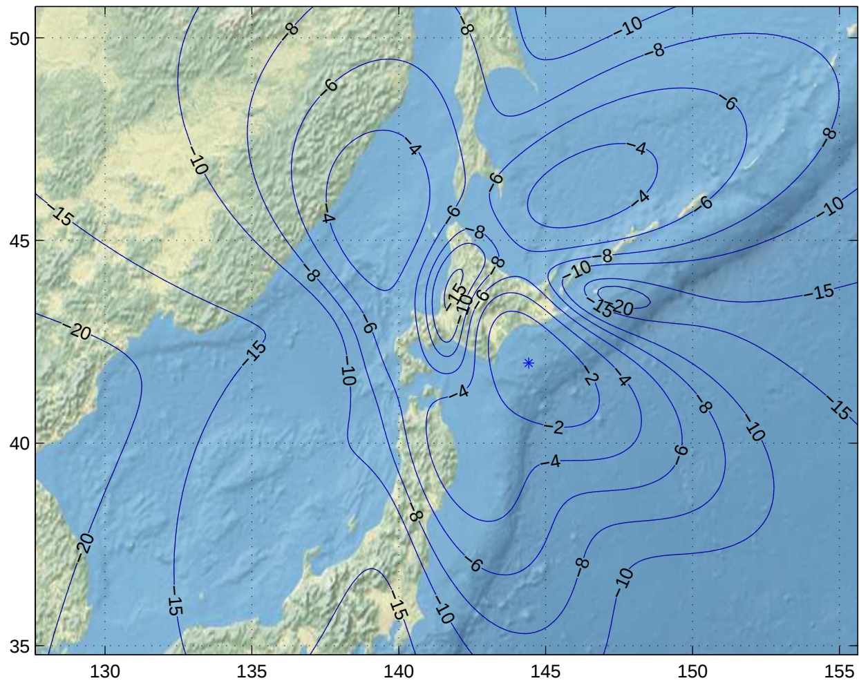
Gain Contours at 385km for CTS. Beam ID=URC, Polarization=h
