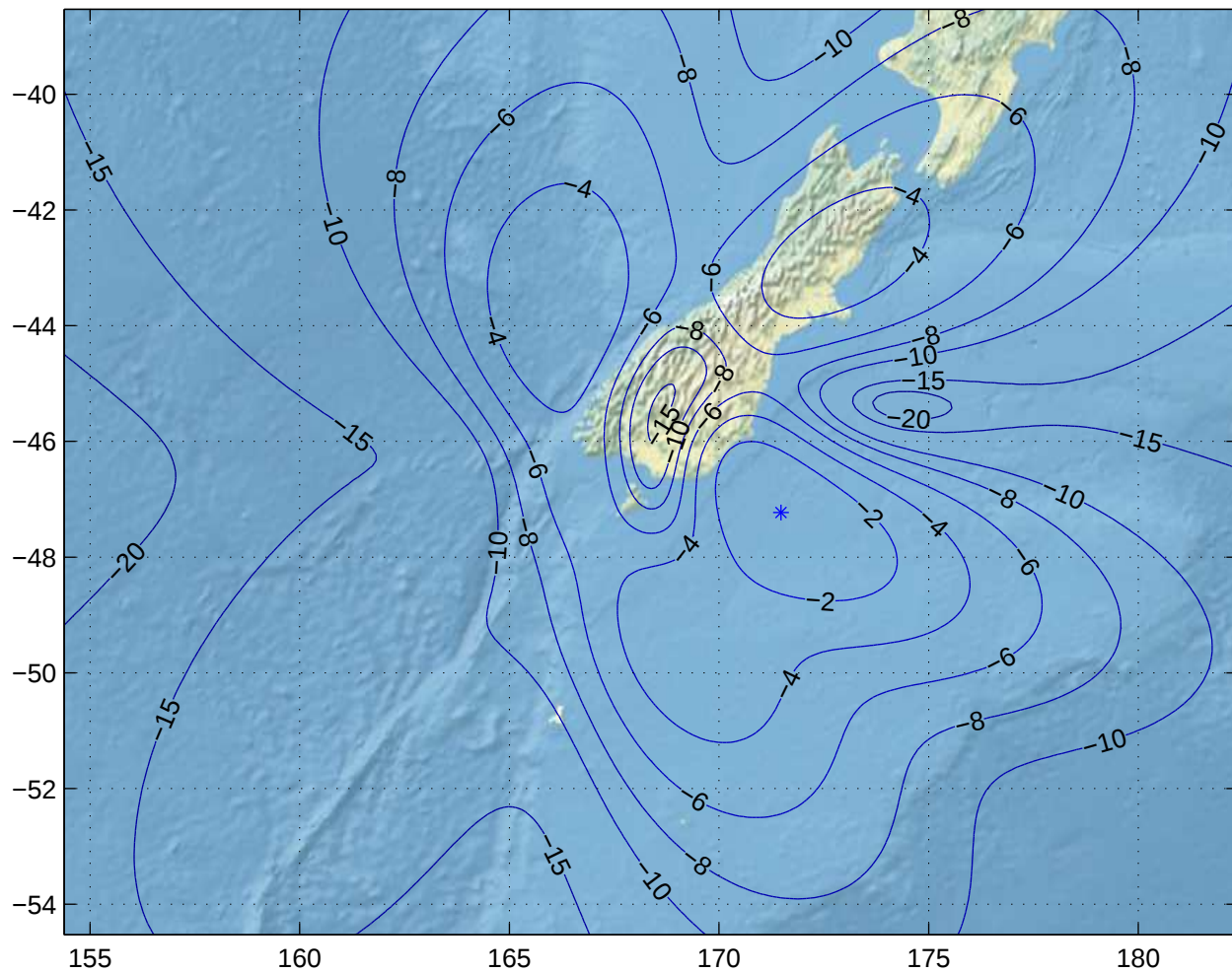
Gain Contours at 385km for IVC. Beam ID=URC, Polarization=h
