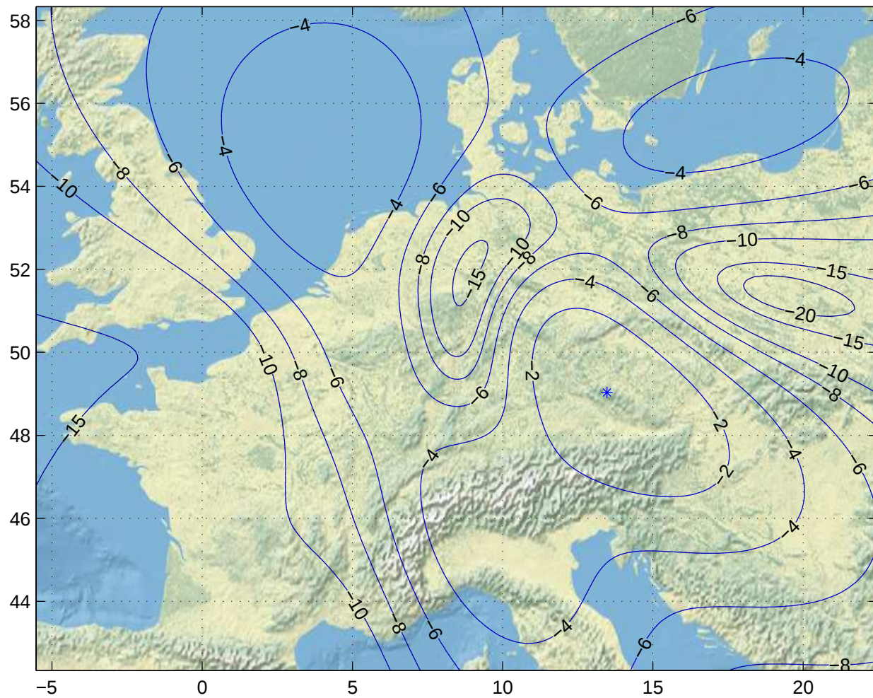
Gain Contours at 600km for FRA. Beam ID=URC, Polarization=h
