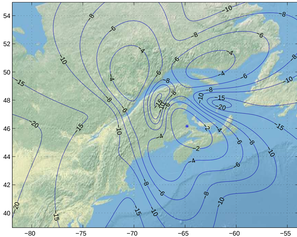
Gain Contours at 385km for PQI. Beam ID=URC, Polarization=h
