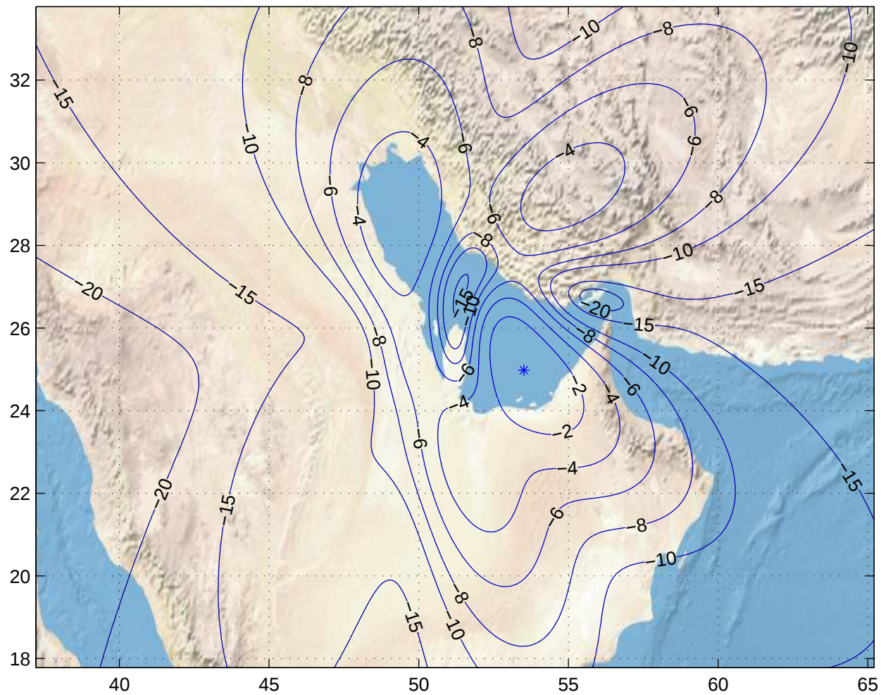
Gain Contours at 385km for DOH. Beam ID=URC, Polarization=h
