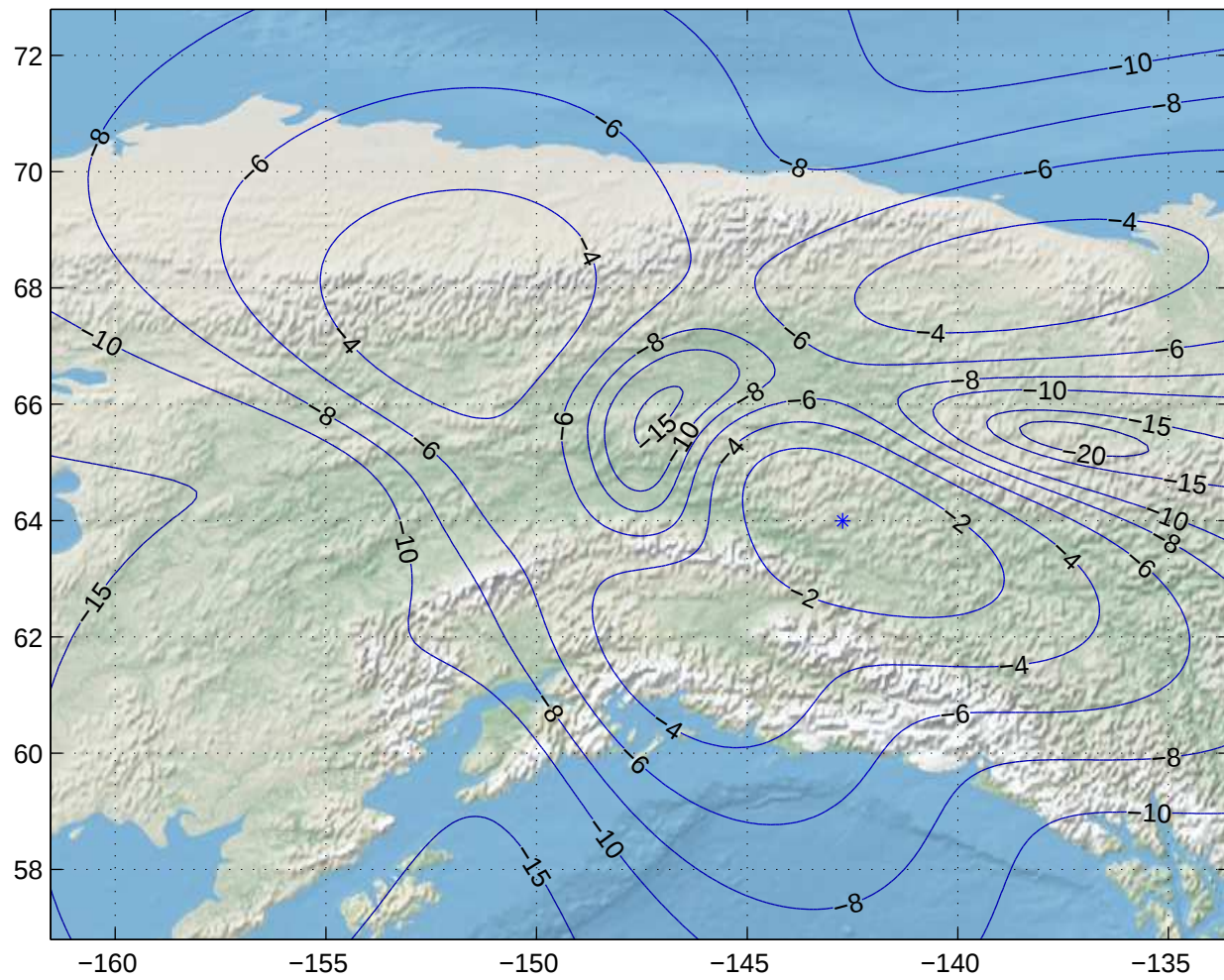
Gain Contours at 385km for FAI. Beam ID=URC, Polarization=h
