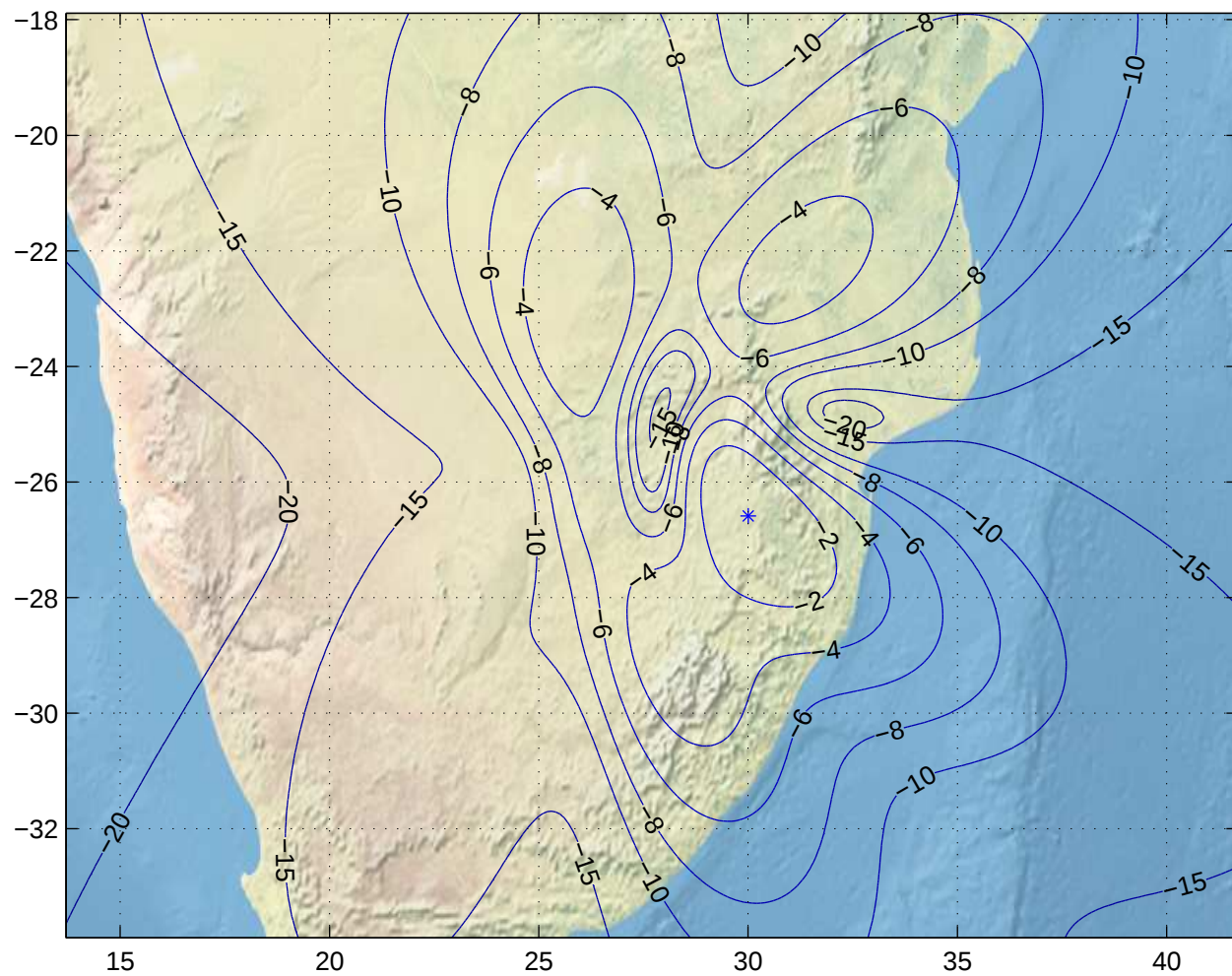
Gain Contours at 385km for JNB. Beam ID=URC, Polarization=h
