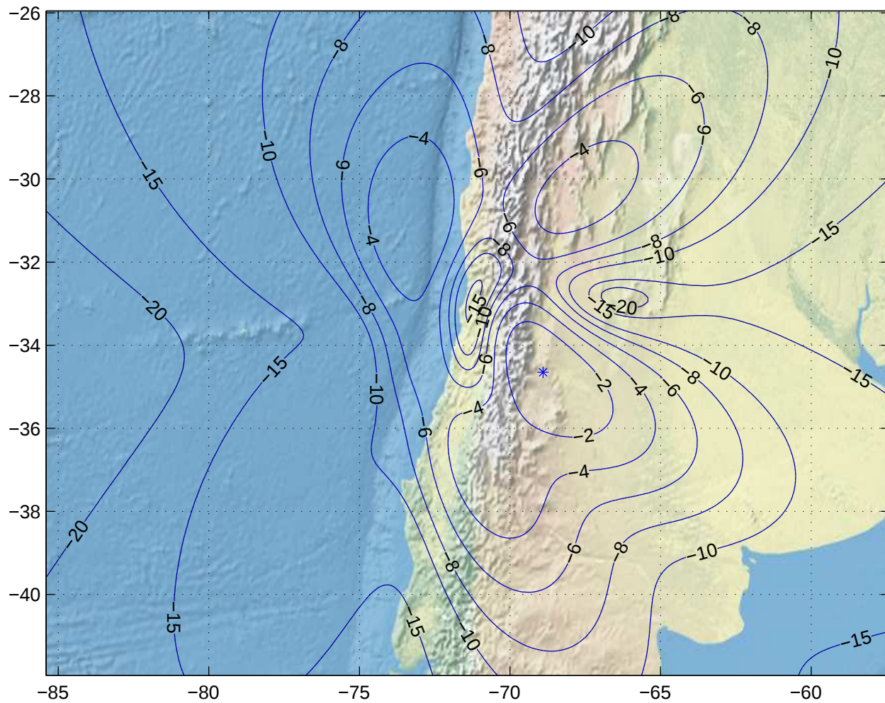
Gain Contours at 385km for SCL. Beam ID=URC, Polarization=h
