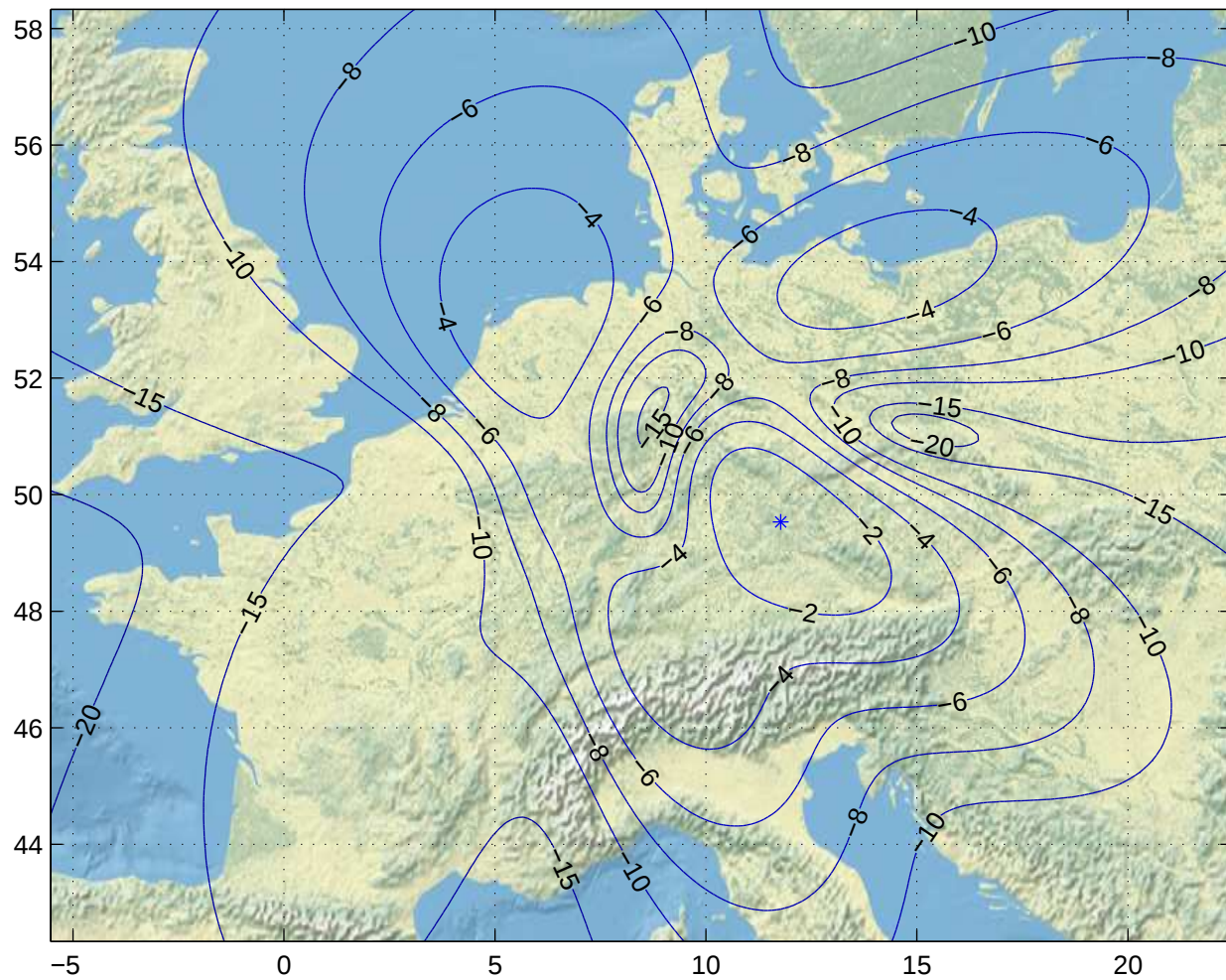
Gain Contours at 385km for FRA. Beam ID=URC, Polarization=h
