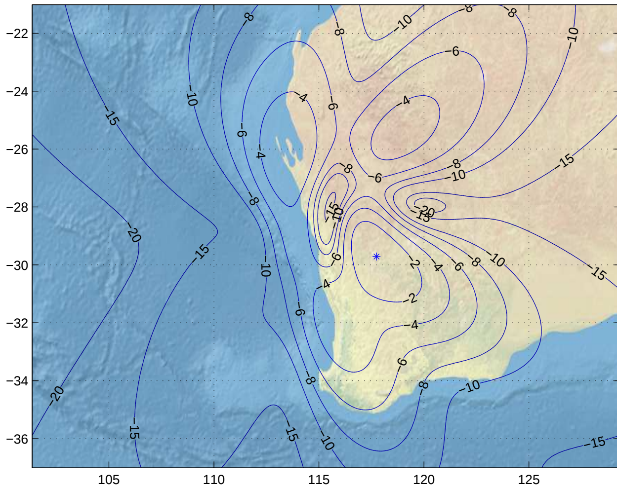
Gain Contours at 385km for GET. Beam ID=URC, Polarization=h
