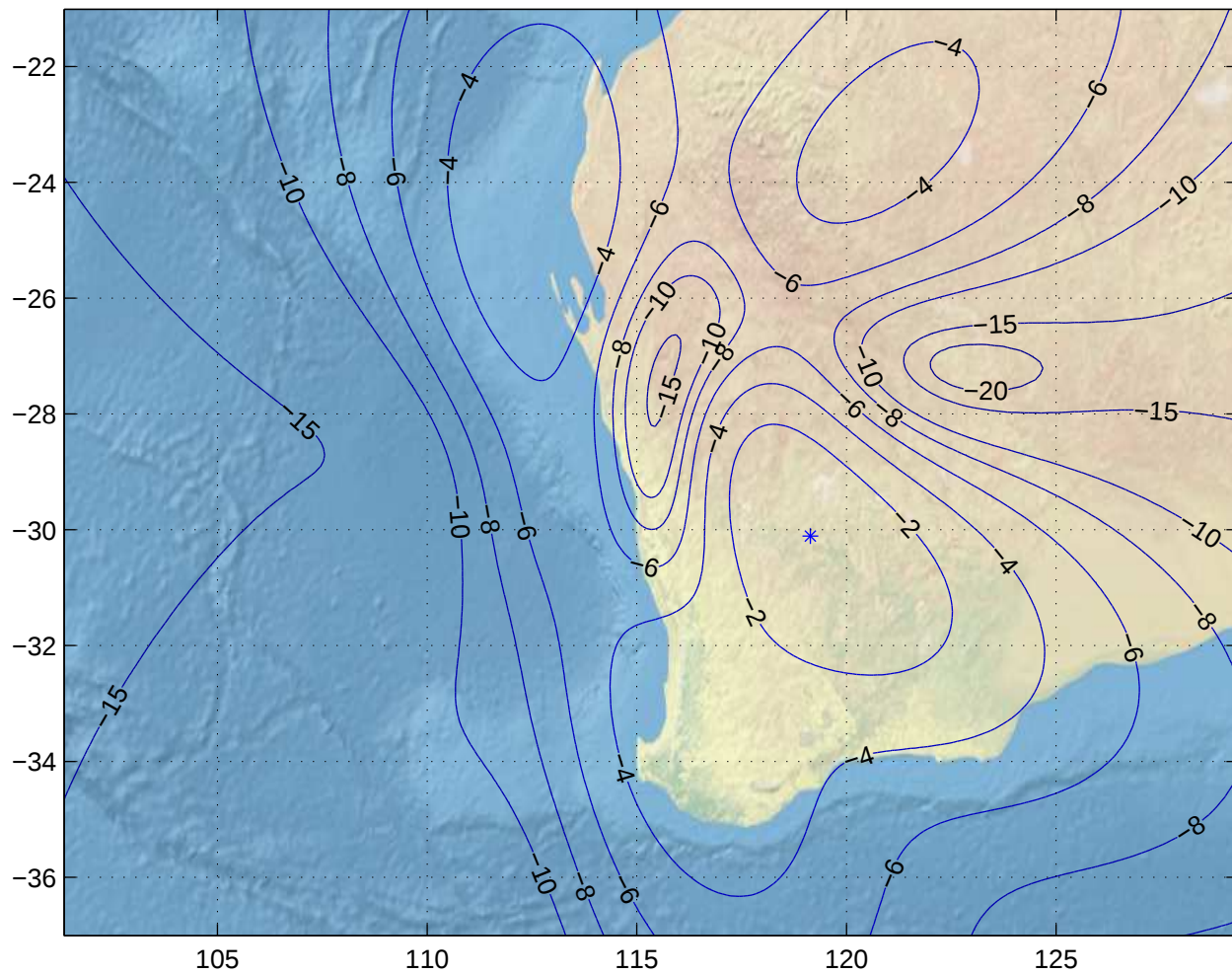
Gain Contours at 600km for GET. Beam ID=URC, Polarization=h
