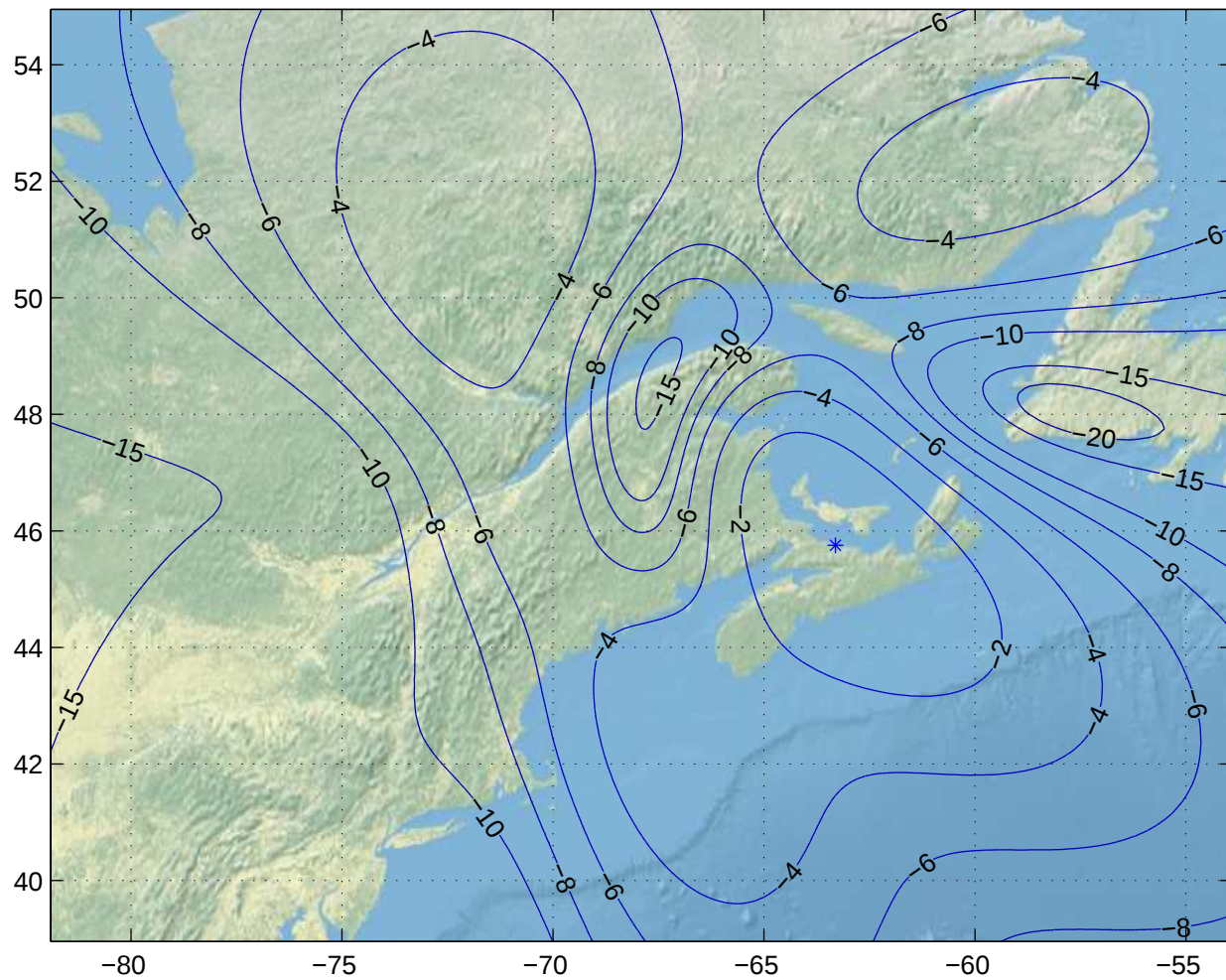
Gain Contours at 600km for PQI. Beam ID=URC, Polarization=h
