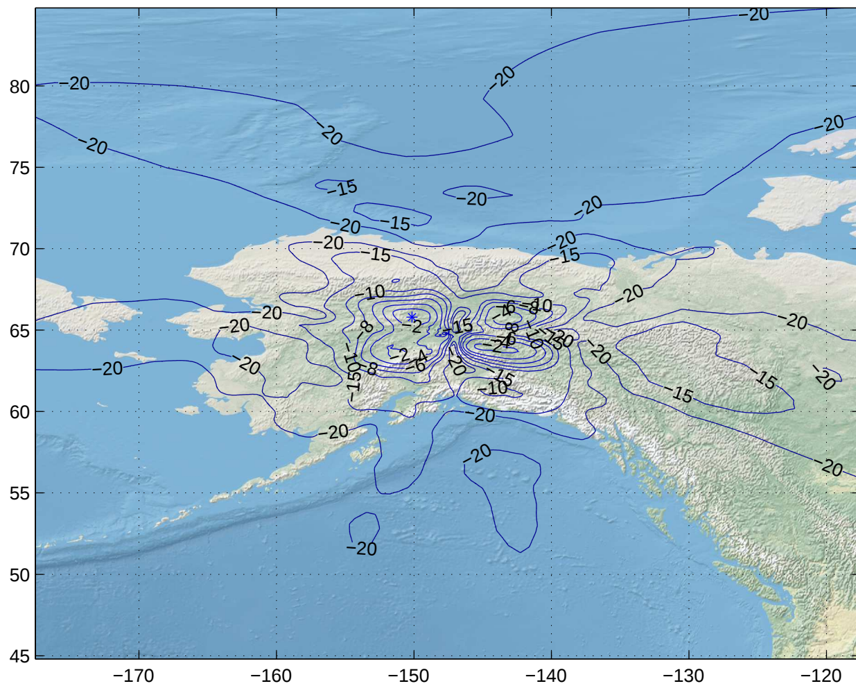
Gain Contours at 575km for FAI. Beam ID=XTX, Polarization=lhcp
