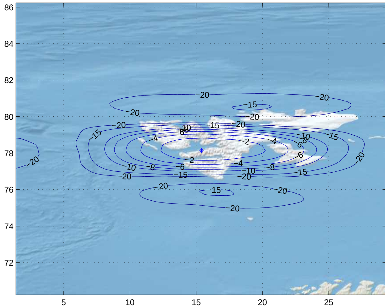
Gain Contours at 575km for LYR. Beam ID=XTC, Polarization=rhcp
