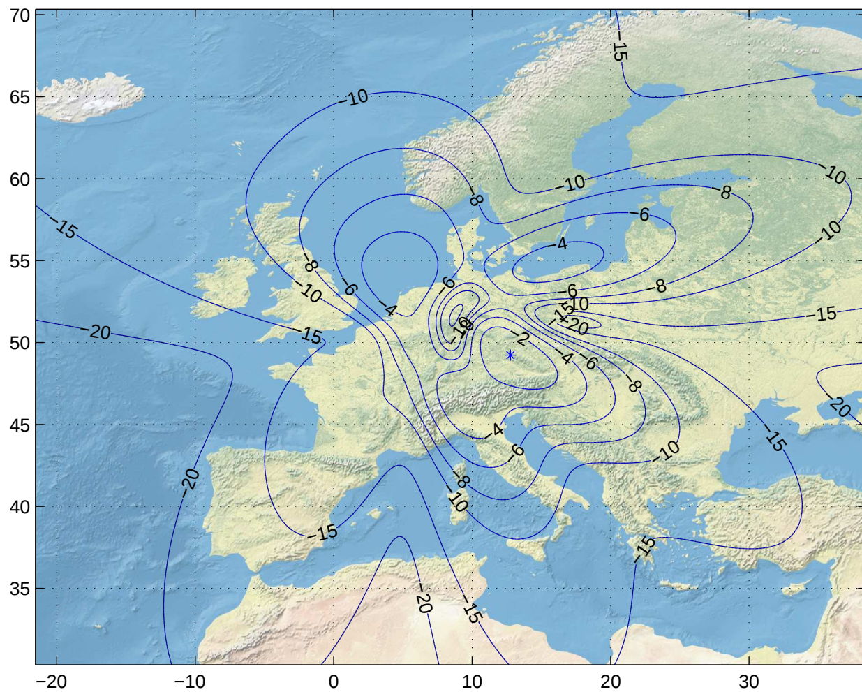
Gain Contours at 505km for FRA. Beam ID=URX, Polarization=rhcp
