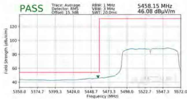
Plot 7-105. Radiated Lower Band Edge Plot (Peak Average – UNII Band 2C)
