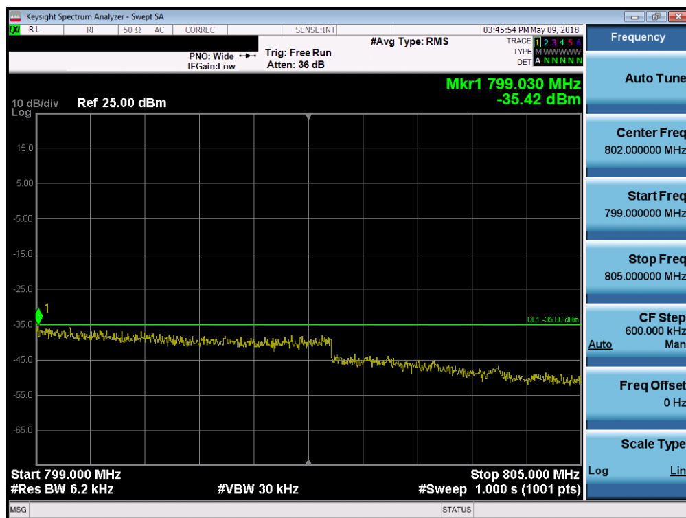
Plot 7-11. Upper Emission Mask Band Edge Plot (LTE B14 - 5MHz QPSK – RB Size 25)
