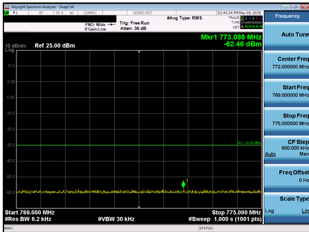
Plot 7-9. Lower Emission Mask Band Edge Plot (LTE B14 - 5MHz QPSK – RB Size 25)
