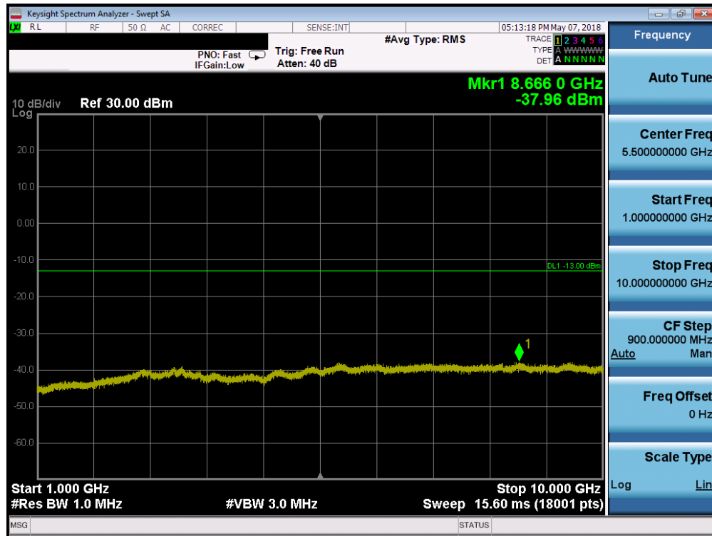
Plot 7-7. Conducted Spurious Plot (LTE B14 – 10.0MHz QPSK – RB Size 1, RB Offset 0 – Mid Channel)
