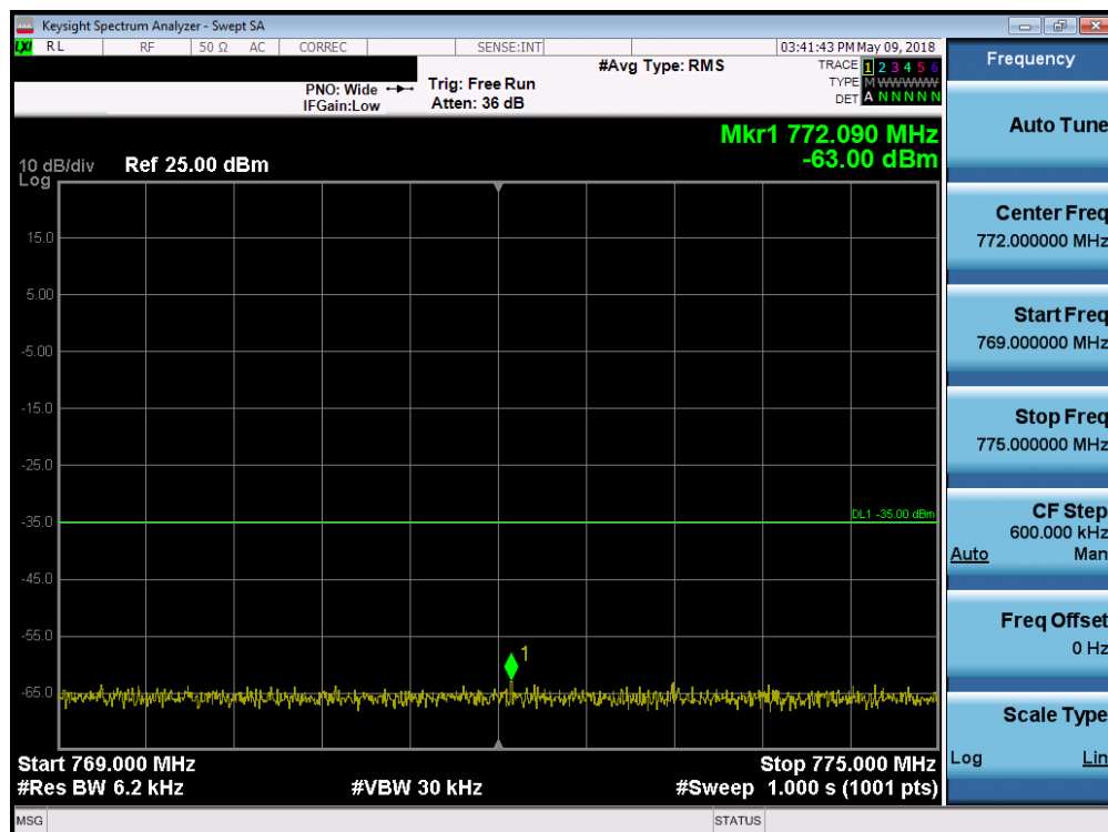
Plot 7-13. Lower Emission Mask Band Edge Plot (LTE B14 - 10MHz QPSK – RB Size 50)
