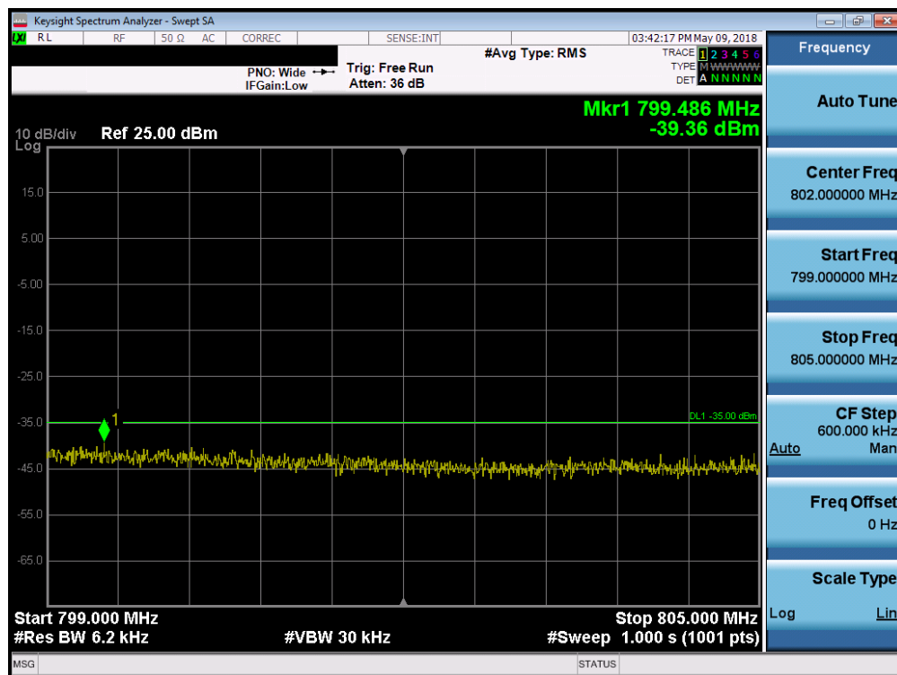
Plot 7-15. Upper Emission Mask Band Edge Plot (LTE B14 - 10MHz QPSK – RB Size 50)
