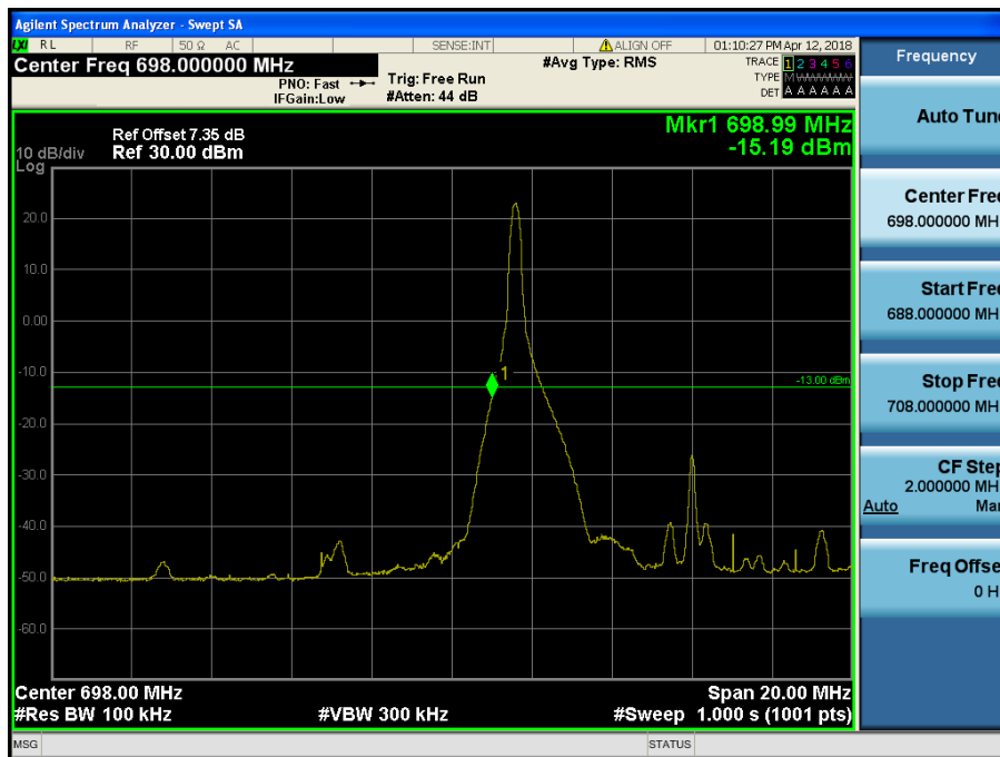
LTE Band 12 / 10MHz / QPSK - RB Size/Offset (1/0)
