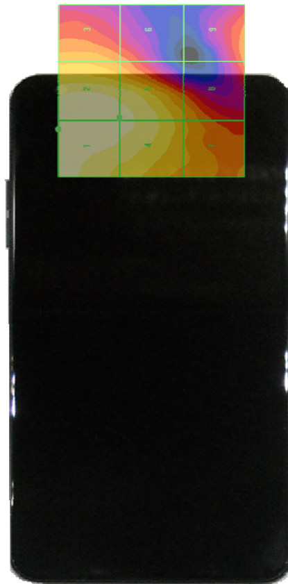
Figure 18-4 E-Field WD Scan overlay
