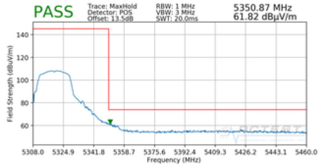
Plot 7-88. Radiated Upper Band Edge Plot (Peak – UNII Band 2A)
