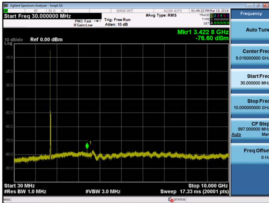
BAND 66/4. Conducted Spurious Plot_1 (132047ch_15MHz_QPSK_RB 1_0)
