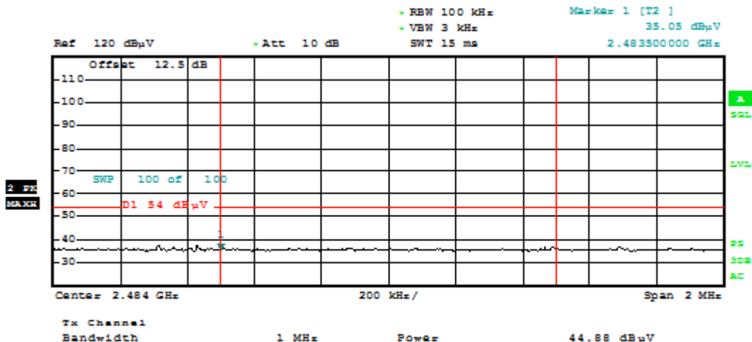
Plot 6-1. Radiated Restricted Upper Band Edge Measurement (Average)
