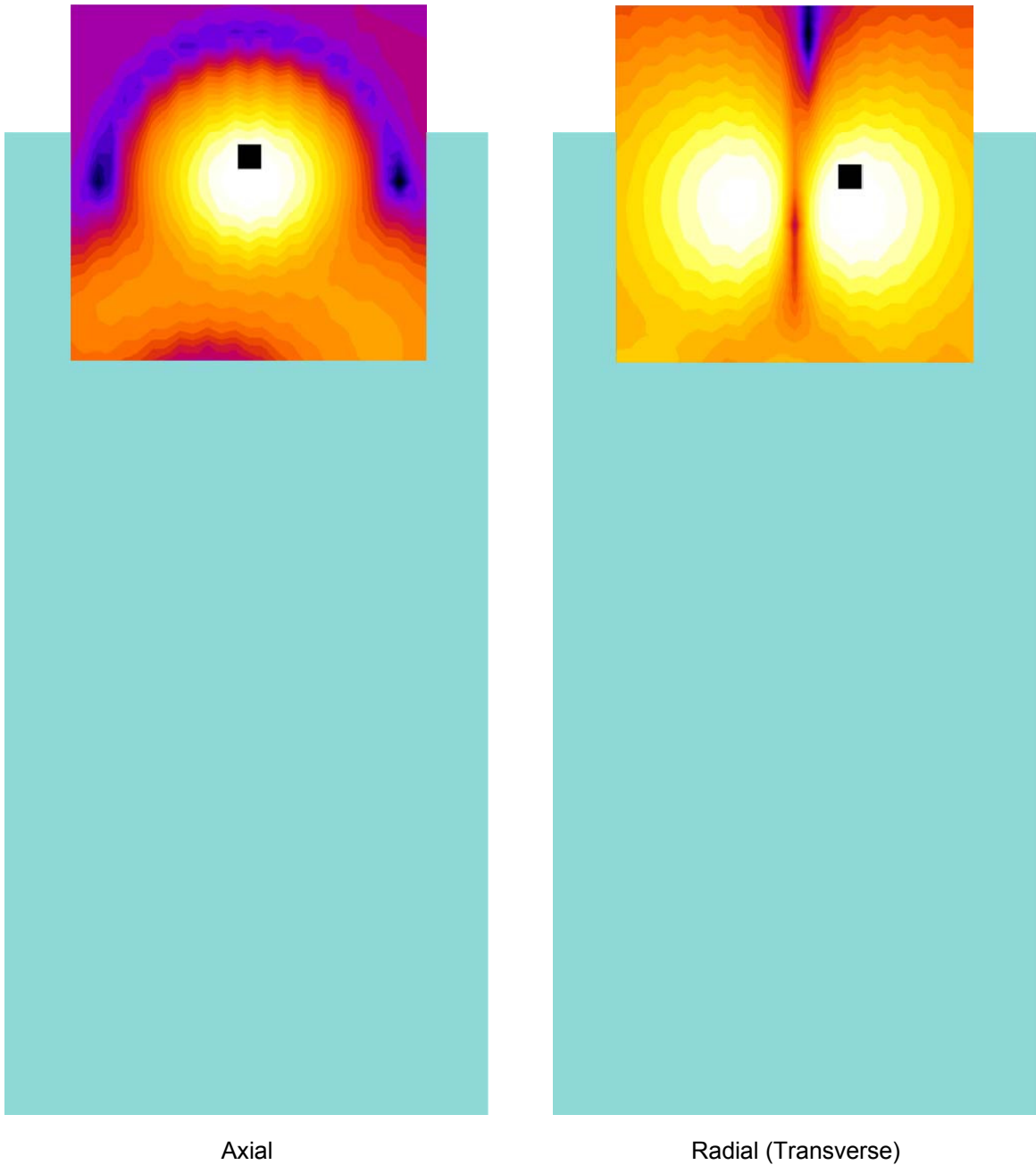
Axial Radial (Transverse) Figure 7-1 T-Coil Scan Overlay Magnetic Field Distributions
