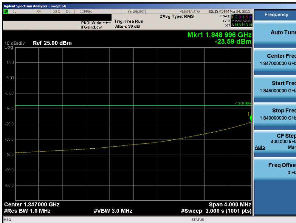
Plot 6-97. Lower Extended Band Edge Plot (Band 2 – 3.0MHz QPSK – RB Size 15)
