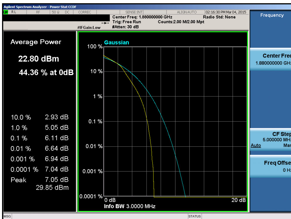
Plot 6-119. PAR Plot (Band 2 – 3.0MHz 16-QAM – RB Size 15)
