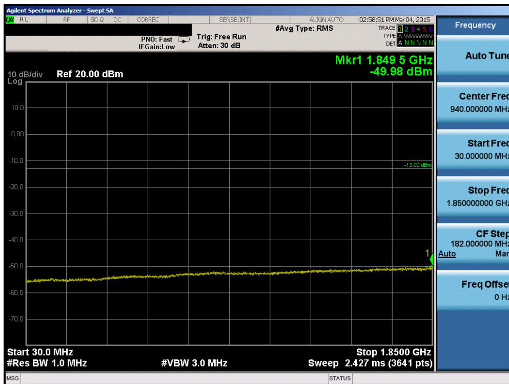
Plot 6-54. Conducted Spurious Plot (Band 2 – 20.0MHz QPSK – RB Size 1, RB Offset 0 – Mid Channel)
