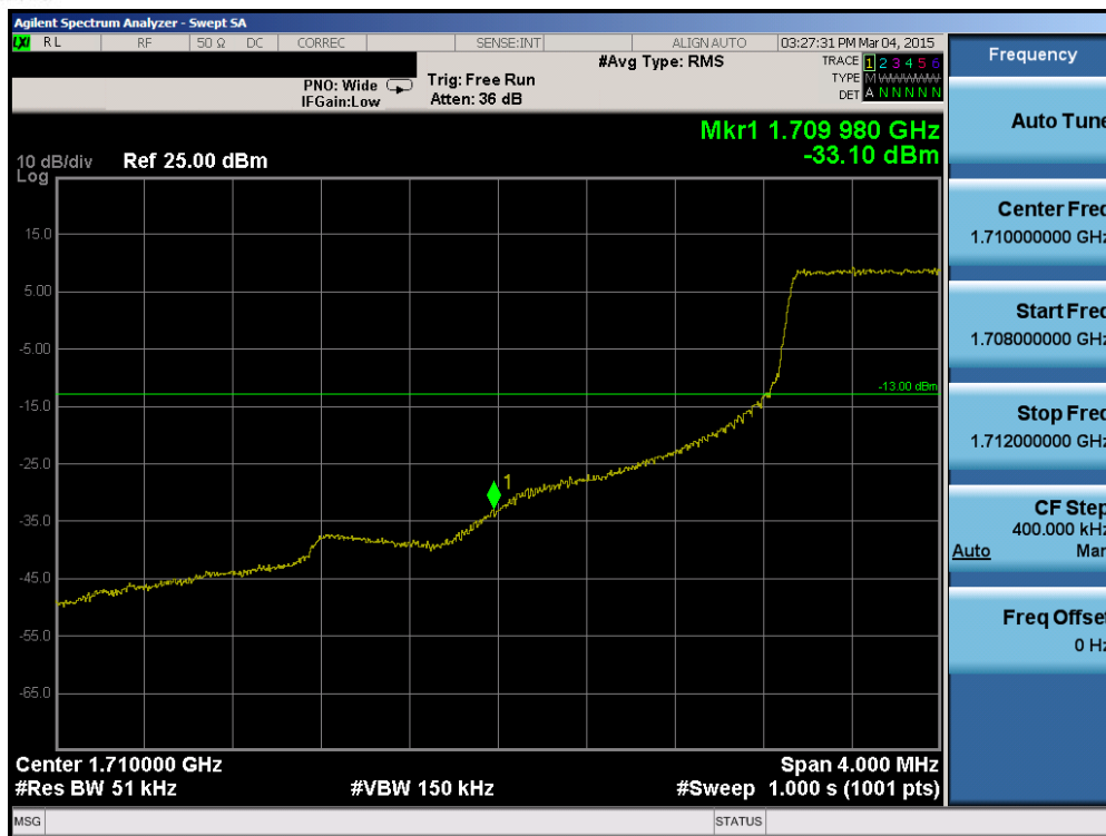
Plot 6-76. Lower Band Edge Plot (Band 4 – 5.0MHz QPSK – RB Size 25)
