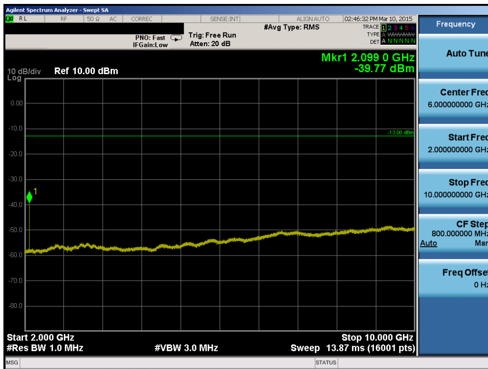
Plot 6-35. Conducted Spurious Plot (Band 12 – 10.0MHz QPSK – RB Size 1, RB Offset 0 – Low Channel)
