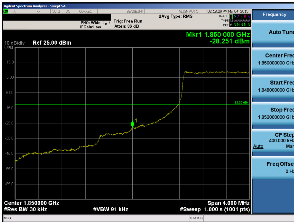
Plot 6-96. Lower Band Edge Plot (Band 2 – 3.0MHz QPSK – RB Size 15)
