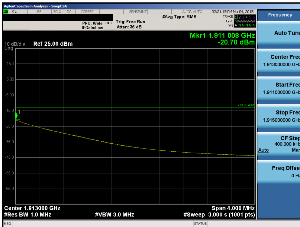
Plot 6-99. Upper Extended Band Edge Plot (Band 2 - 3.0MHz QPSK - RB Size 15)
