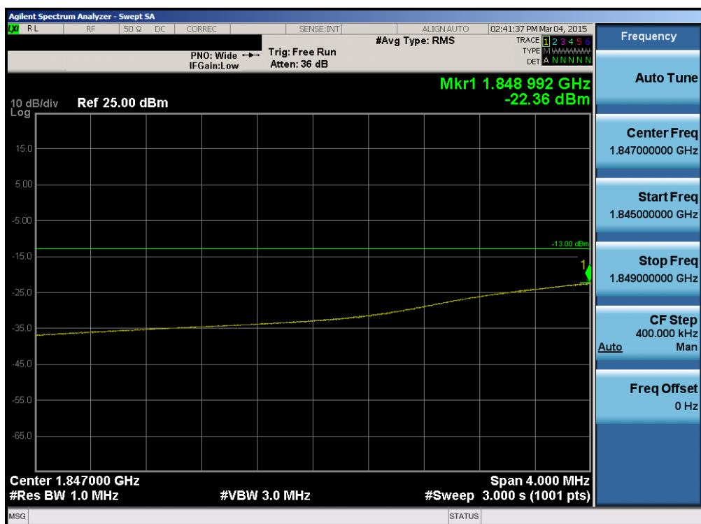
Plot 6-105. Lower Extended Band Edge Plot (Band 2 – 10.0MHz QPSK – RB Size 50)
