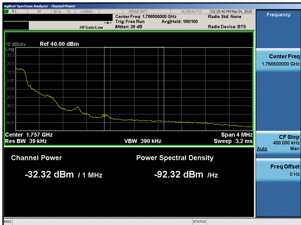
Plot 6-71. Upper Extended Band Edge Plot (Band 4 – 1.4MHz QPSK – RB Size 6)
