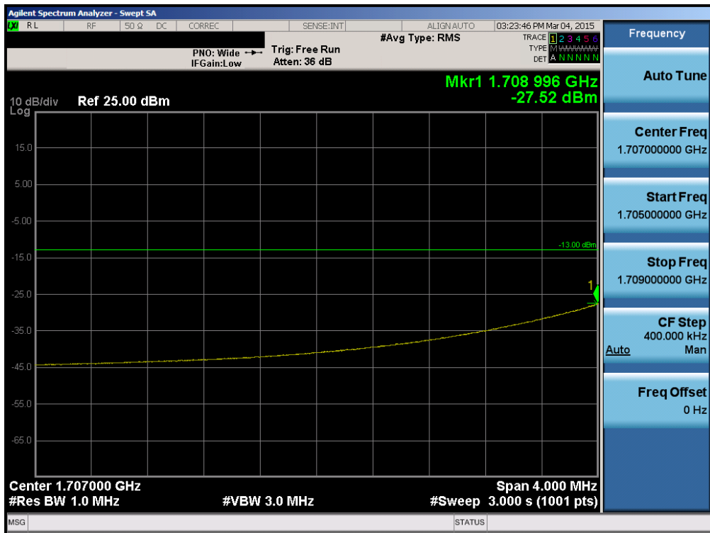
Plot 6-73. Lower Extended Band Edge Plot (Band 4 – 3.0MHz QPSK – RB Size 15)
