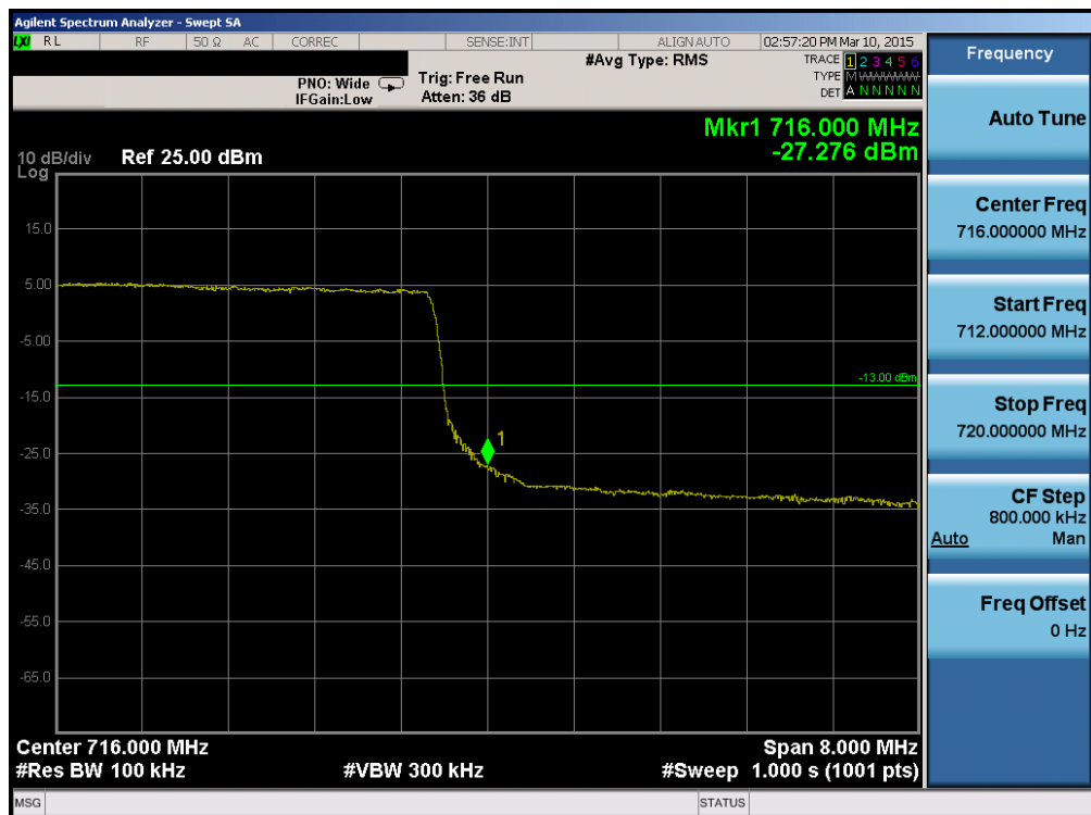
Plot 6-67. Upper Band Edge Plot (Band 12 – 10.0MHz QPSK – RB Size 50)
