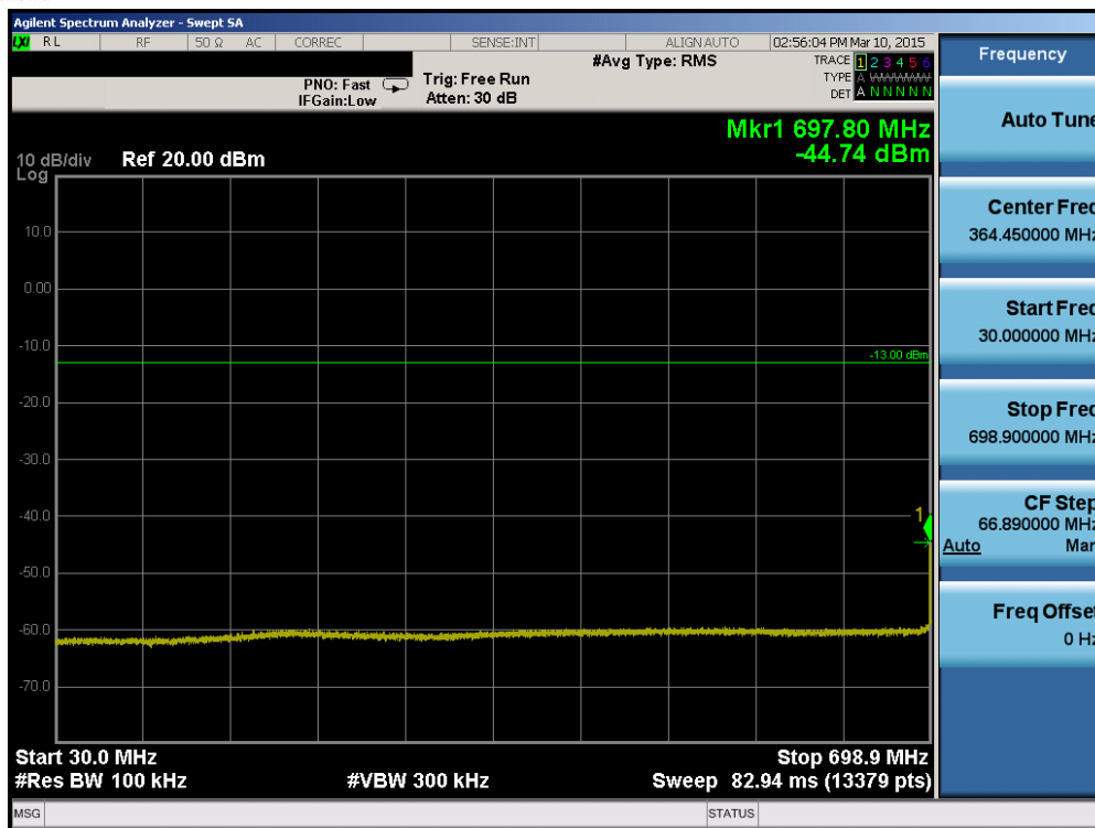
Plot 6-39. Conducted Spurious Plot (Band 12 – 10.0MHz QPSK – RB Size 1, RB Offset 0 – High Channel)
