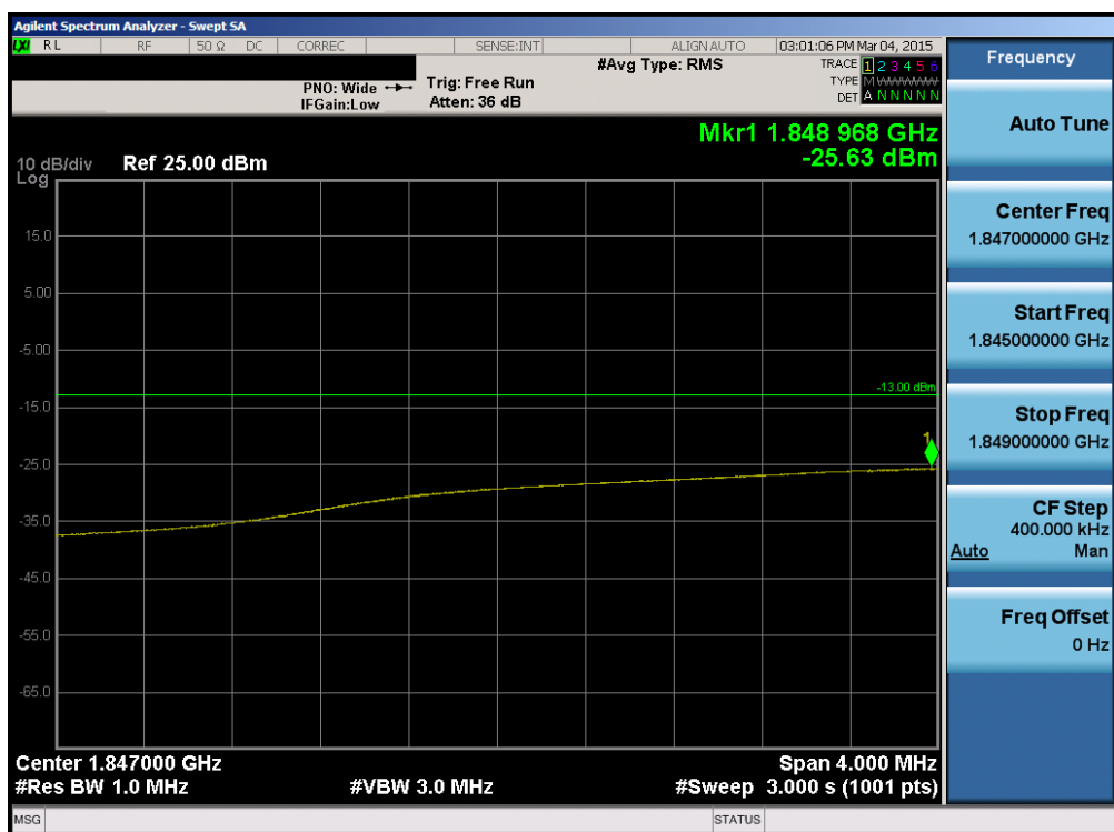
Plot 6-113. Lower Extended Band Edge Plot (Band 2 – 20.0MHz QPSK – RB Size 100)
