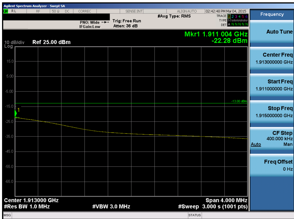
Plot 6-107. Upper Extended Band Edge Plot (Band 2 – 10.0MHz QPSK – RB Size 50)
