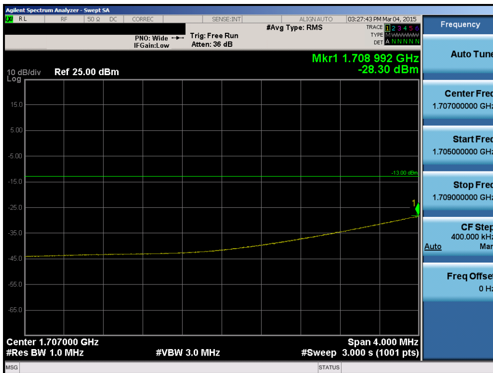
Plot 6-77. Lower Extended Band Edge Plot (Band 4 – 5.0MHz QPSK – RB Size 25)
