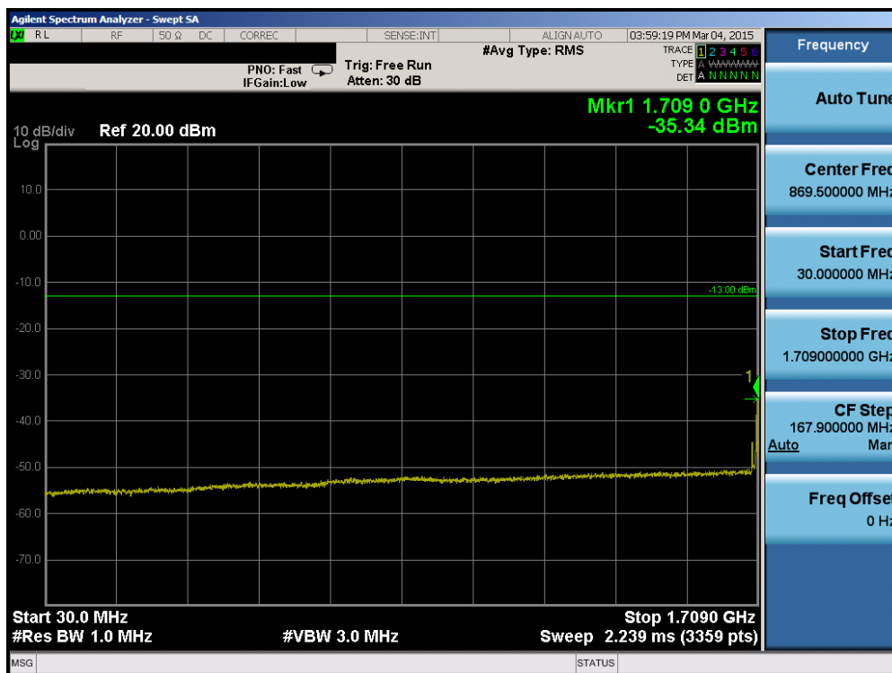
Plot 6-42. Conducted Spurious Plot (Band 4 – 20.0MHz QPSK – RB Size 1, RB Offset 0– Low Channel)
