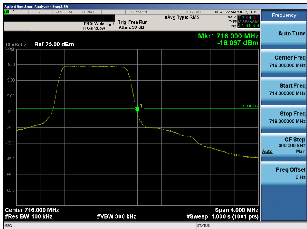
Plot 6-61. Upper Band Edge Plot (Band 12 – 1.4MHz QPSK – RB Size 6)
