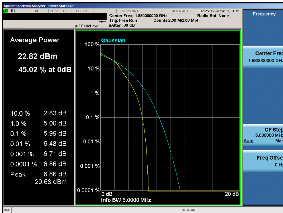
Plot 6-121. PAR Plot (Band 2 – 5.0MHz 16-QAM – RB Size 25)
