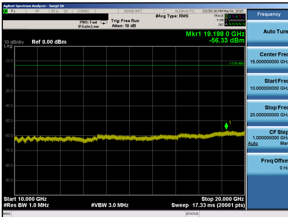
Plot 6-44. Conducted Spurious Plot (Band 4 – 20.0MHz QPSK – RB Size 1, RB Offset 0 – Low Channel)
