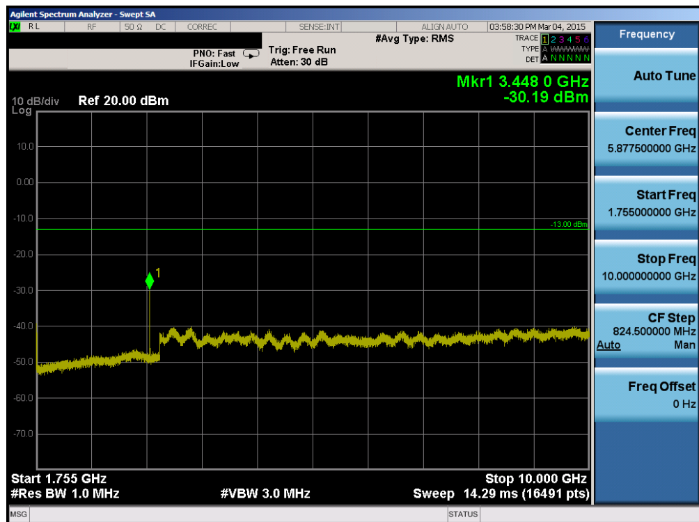
Plot 6-46. Conducted Spurious Plot (Band 4 – 20.0MHz QPSK – RB Size 1, RB Offset 0 – Mid Channel)
