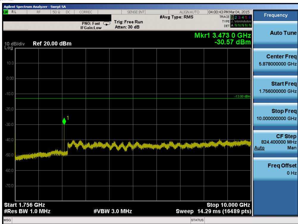
Plot 6-49. Conducted Spurious Plot (Band 4 – 20.0MHz QPSK – RB Size 1, RB Offset 0 – High Channel)
