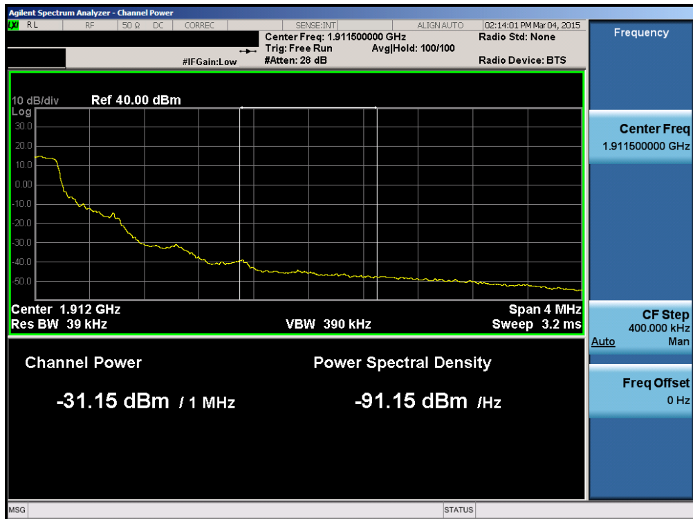
Plot 6-95. Upper Extended Band Edge Plot (Band 2 – 1.4MHz QPSK – RB Size 6)
