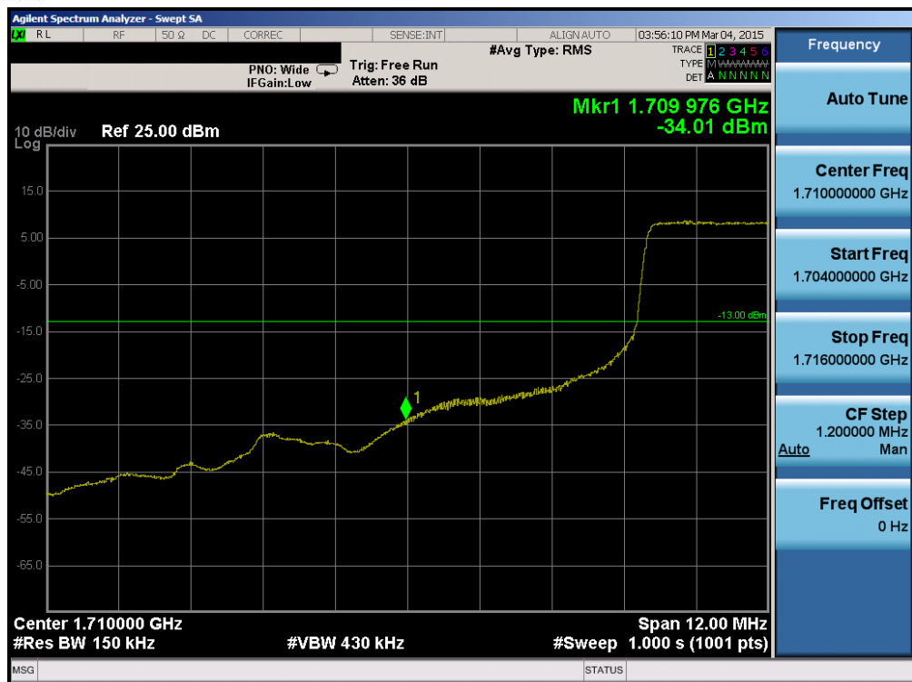
Plot 6-84. Lower Band Edge Plot (Band 4 – 15.0MHz QPSK – RB Size 75)
