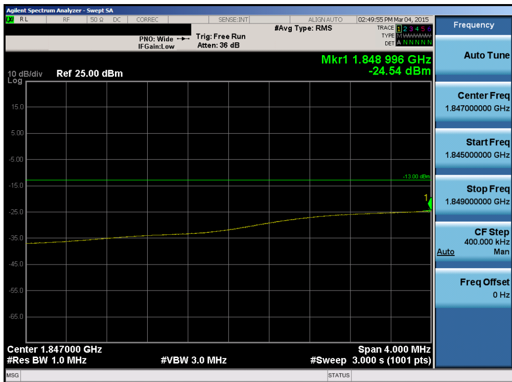
Plot 6-109. Lower Extended Band Edge Plot (Band 2 – 15.0MHz QPSK – RB Size 75)
