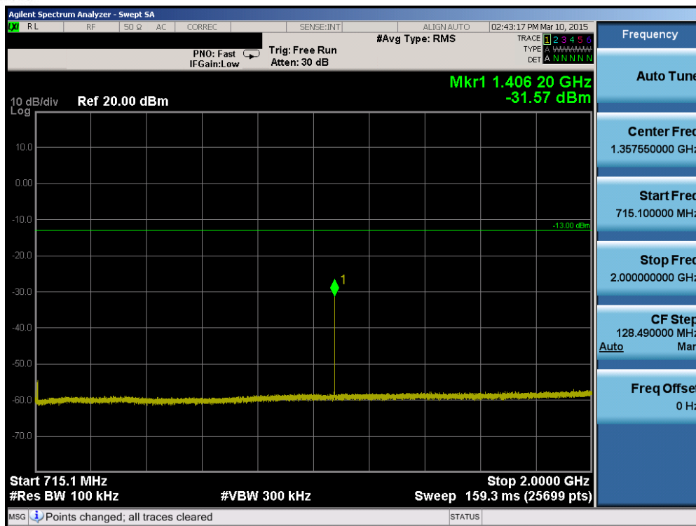
Plot 6-37. Conducted Spurious Plot (Band 12 – 10.0MHz QPSK – RB Size 1, RB Offset 0 – Mid Channel)
