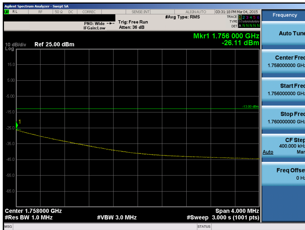
Plot 6-79. Upper Extended Band Edge Plot (Band 4 - 5.0MHz QPSK - RB Size 25)
