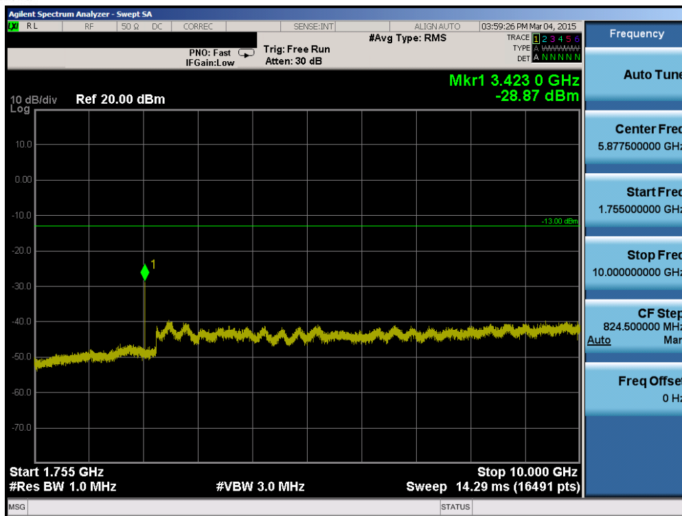
Plot 6-43. Conducted Spurious Plot (Band 4 – 20.0MHz QPSK – RB Size 1, RB Offset 0 – Low Channel)
