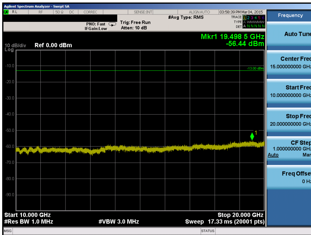
Plot 6-47. Conducted Spurious Plot (Band 4 – 20.0MHz QPSK – RB Size 1, RB Offset 0 – Mid Channel)
