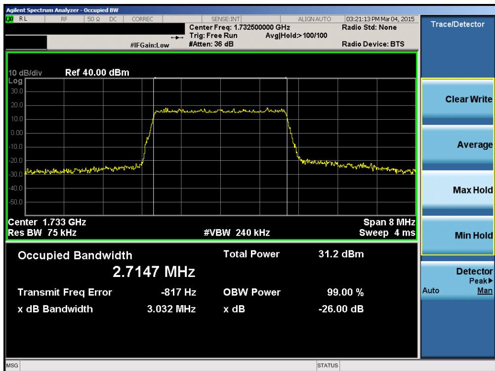
Plot 6-12. Occupied Bandwidth Plot (Band 4 – 3.0MHz 16-QAM – RB Size 15)
