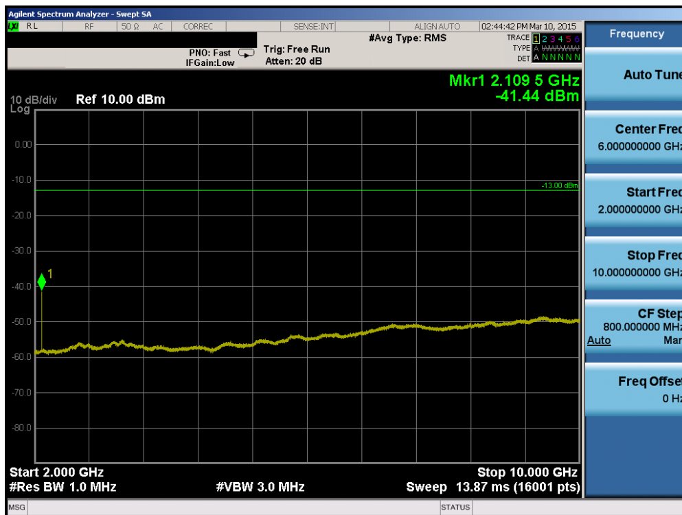
Plot 6-38. Conducted Spurious Plot (Band 12 – 10.0MHz QPSK – RB Size 1, RB Offset 0 – Mid Channel)
