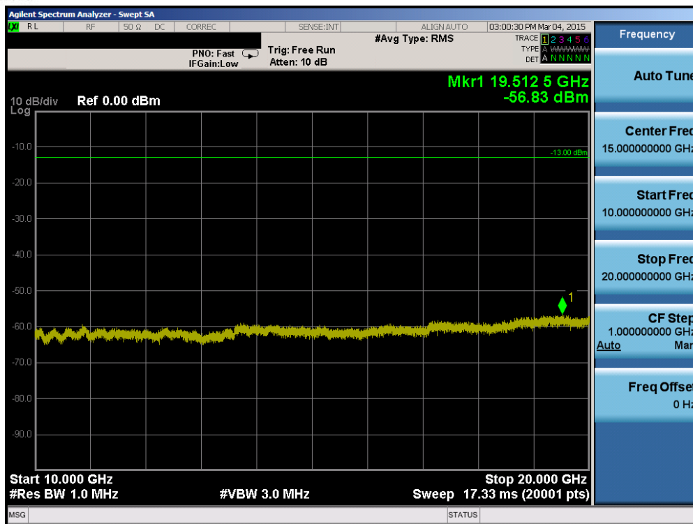
Plot 6-53. Conducted Spurious Plot (Band 2 – 20.0MHz QPSK – RB Size 1, RB Offset 0 – Low Channel)
