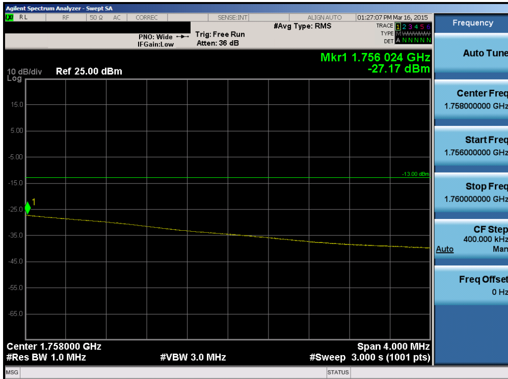
Plot 6-87. Upper Extended Band Edge Plot (Band 4 – 15.0MHz QPSK – RB Size 75)
