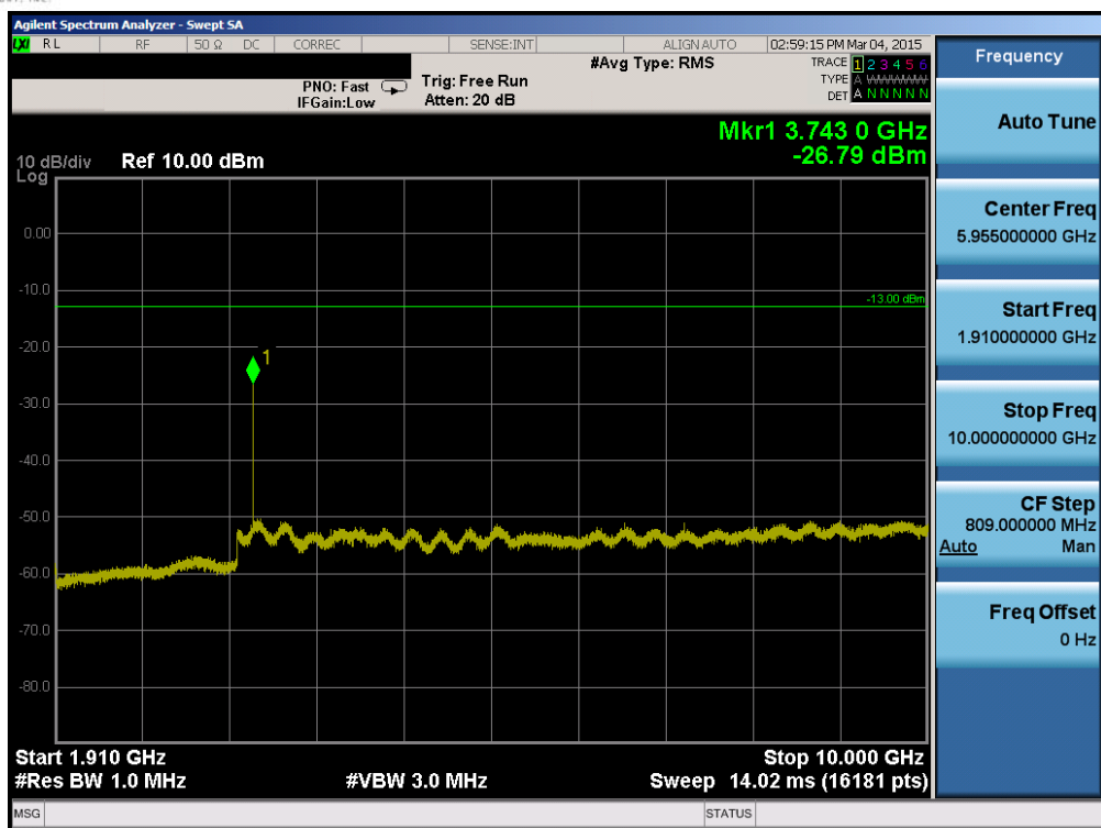
Plot 6-55. Conducted Spurious Plot (Band 2 – 20.0MHz QPSK – RB Size 1, RB Offset 0 – Mid Channel)
