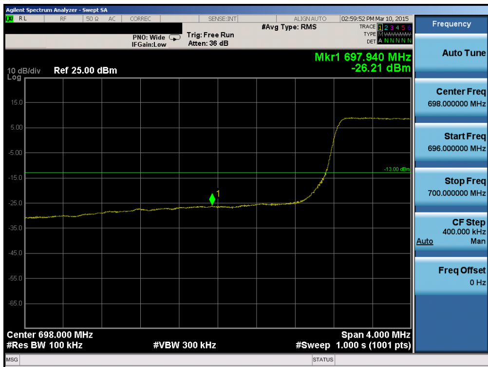
Plot 6-64. Lower Band Edge Plot (Band 12 – 5.0MHz QPSK – RB Size 25)
