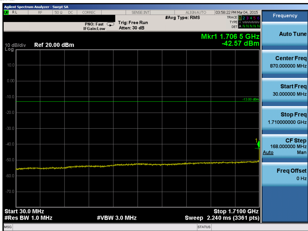
Plot 6-45. Conducted Spurious Plot (Band 4 – 20.0MHz QPSK – RB Size 1, RB Offset 0 – Mid Channel)
