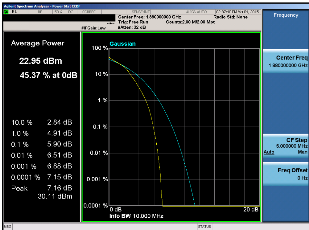
Plot 6-123. PAR Plot (Band 2 – 10.0MHz 16-QAM – RB Size 50)
