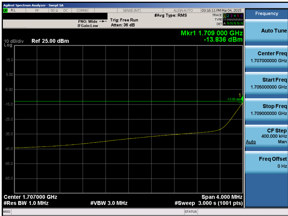
Plot 6-69. Lower Extended Band Edge Plot (Band 4 - 1.4MHz QPSK - RB Size 6)
