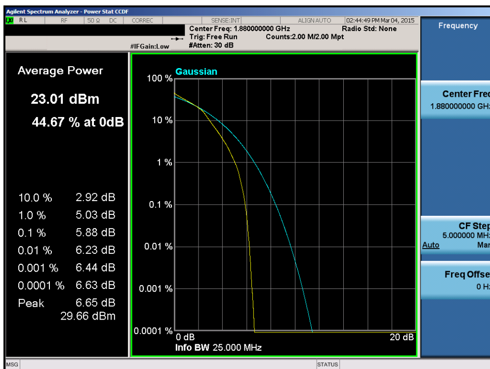
Plot 6-125. PAR Plot (Band 2 – 15.0MHz 16-QAM – RB Size 75)
