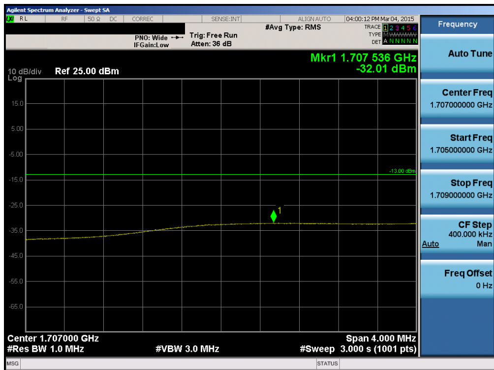
Plot 6-89. Lower Extended Band Edge Plot (Band 4 – 20.0MHz QPSK – RB Size 100)
