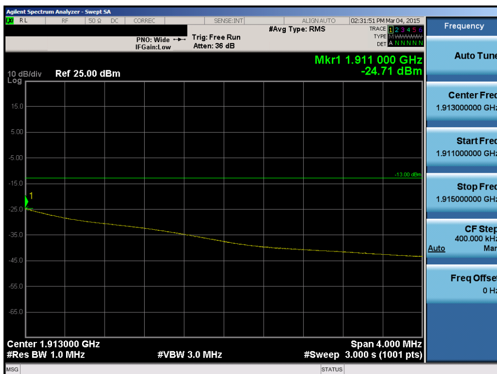
Plot 6-103. Upper Extended Band Edge Plot (Band 2 – 5.0MHz QPSK – RB Size 25)
