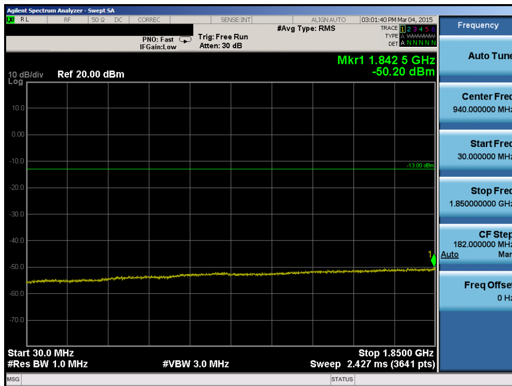
Plot 6-57. Conducted Spurious Plot (Band 2 – 20.0MHz QPSK – RB Size 1, RB Offset 0 – High Channel)
