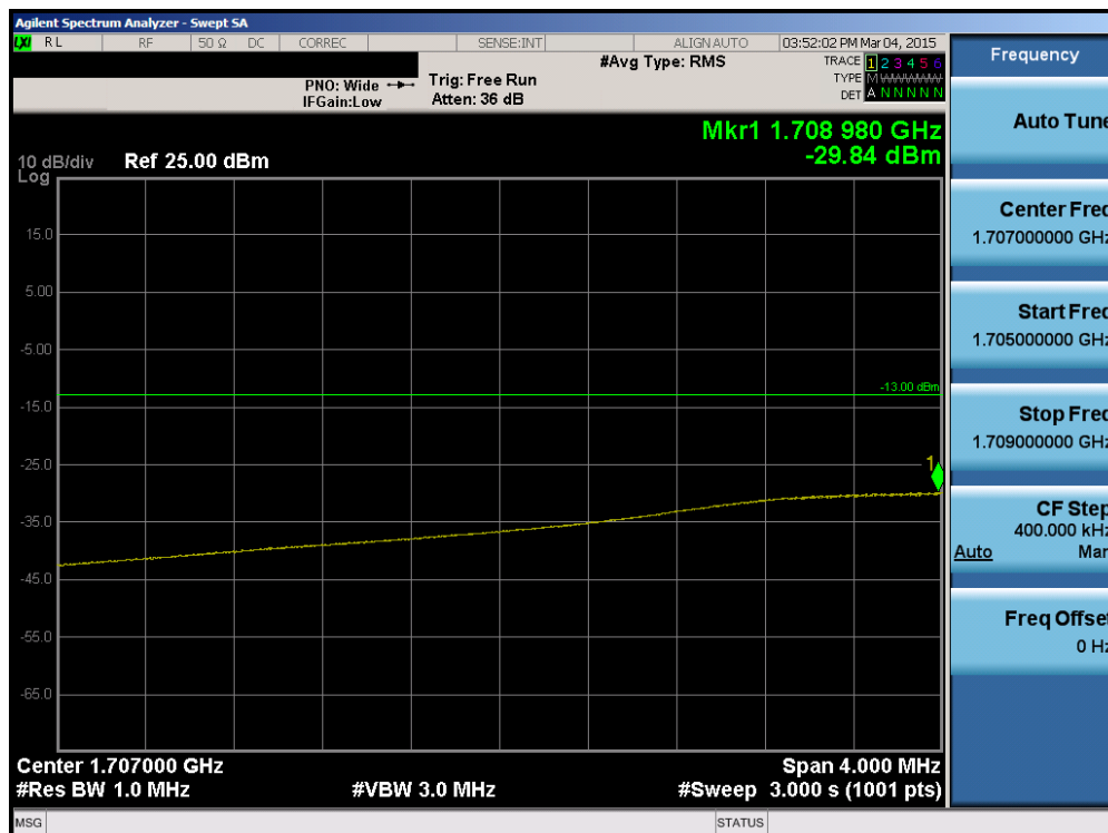
Plot 6-81. Lower Extended Band Edge Plot (Band 4 – 10.0MHz QPSK – RB Size 50)
