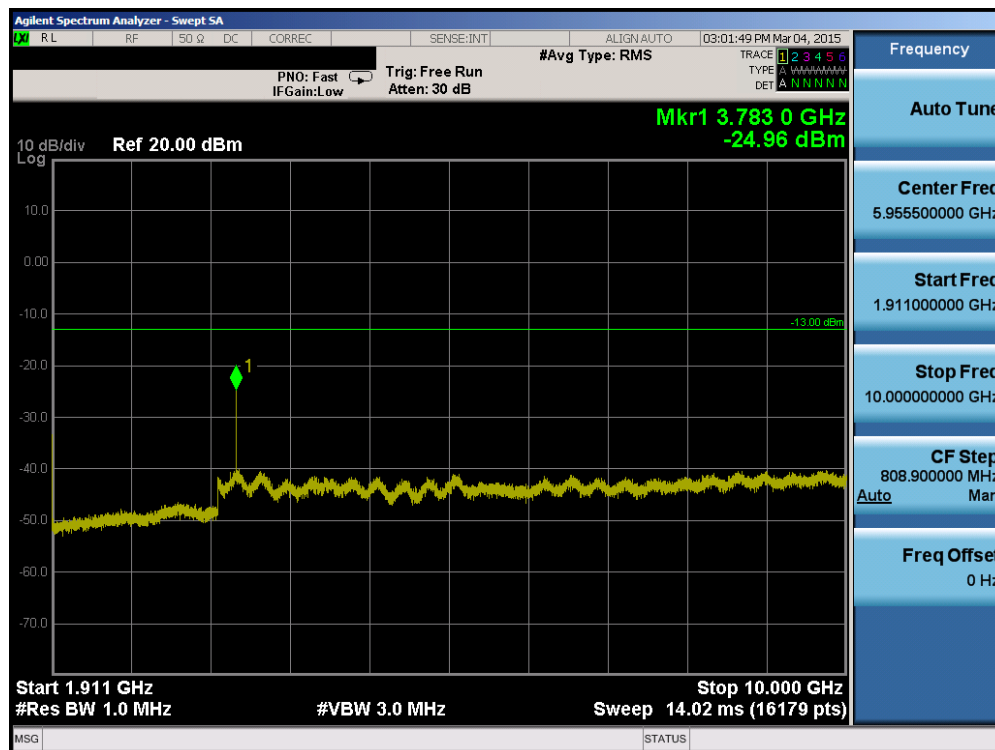
Plot 6-58. Conducted Spurious Plot (Band 2 – 20.0MHz QPSK – RB Size 1, RB Offset 0 – High Channel)
