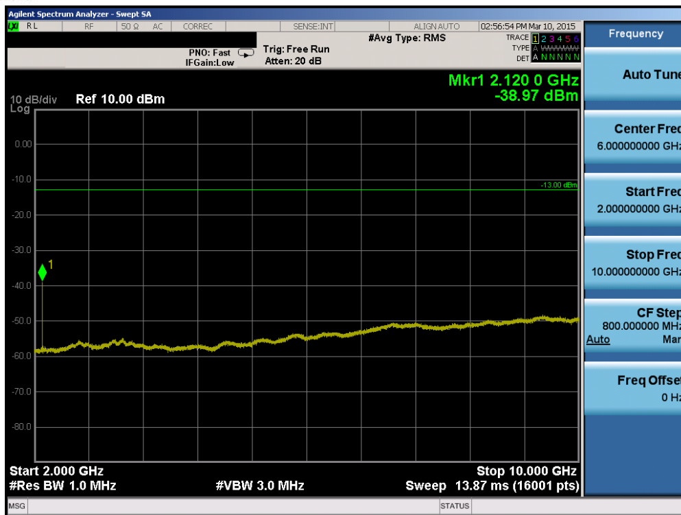
Plot 6-41. Conducted Spurious Plot (Band 12 – 10.0MHz QPSK – RB Size 1, RB Offset 0 – High Channel)
