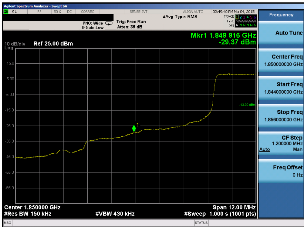
Plot 6-108. Lower Band Edge Plot (Band 2 – 15.0MHz QPSK – RB Size 75)
