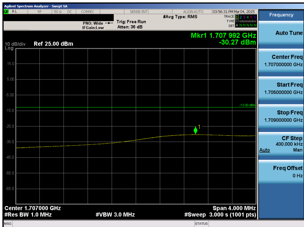
Plot 6-85. Lower Extended Band Edge Plot (Band 4 – 15.0MHz QPSK – RB Size 75)
