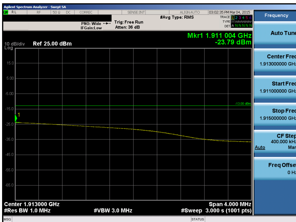
Plot 6-115. Upper Extended Band Edge Plot (Band 2 – 20.0MHz QPSK – RB Size 100)
