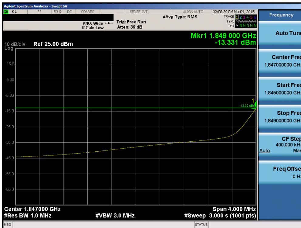
Plot 6-93. Lower Extended Band Edge Plot (Band 2 – 1.4MHz QPSK – RB Size 6)
