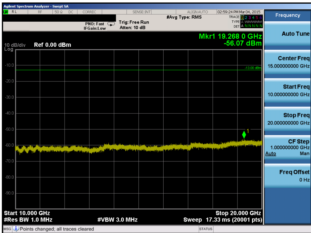
Plot 6-56. Conducted Spurious Plot (Band 2 – 20.0MHz QPSK – RB Size 1, RB Offset 0 – Mid Channel)
