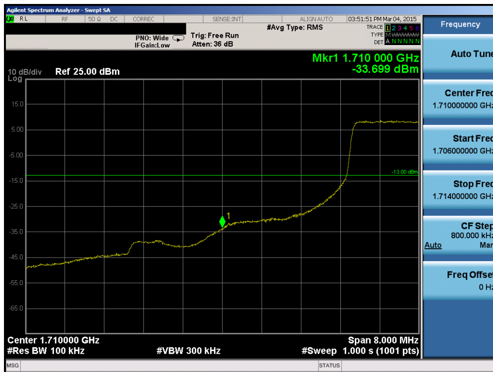
Plot 6-80. Lower Band Edge Plot (Band 4 – 10.0MHz QPSK – RB Size 50)
