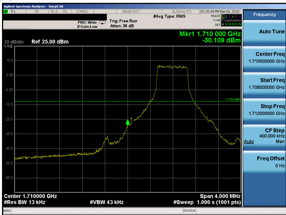
Plot 6-68. Lower Band Edge Plot (Band 4 - 1.4MHz QPSK - RB Size 6)
