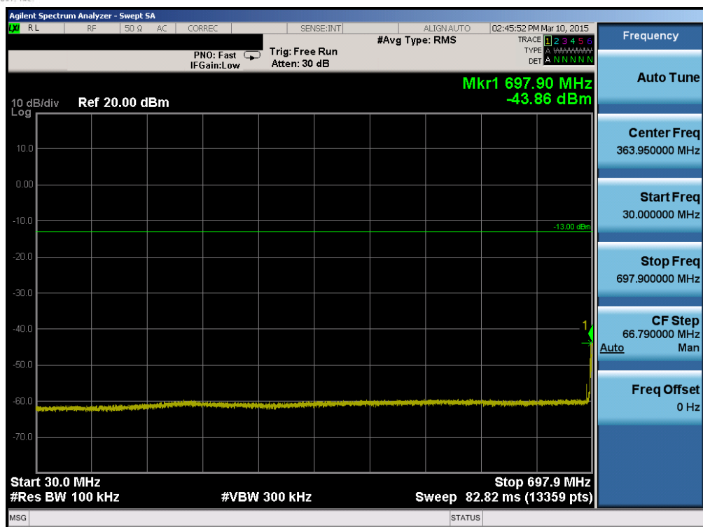
Plot 6-33. Conducted Spurious Plot (Band 12 – 10.0MHz QPSK – RB Size 1, RB Offset 0– Low Channel)
