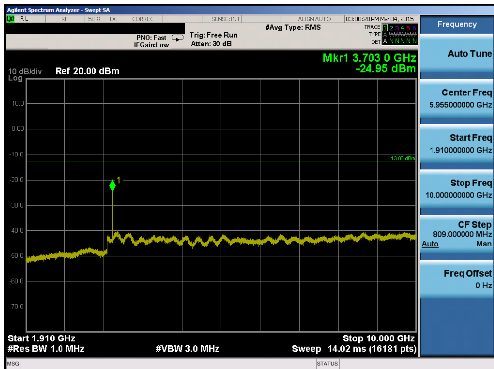
Plot 6-52. Conducted Spurious Plot (Band 2 – 20.0MHz QPSK – RB Size 1, RB Offset 0 – Low Channel)
