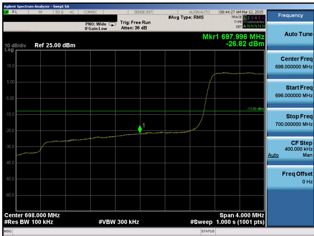
Plot 6-62. Lower Band Edge Plot (Band 12 - 3.0MHz QPSK - RB Size 15)
