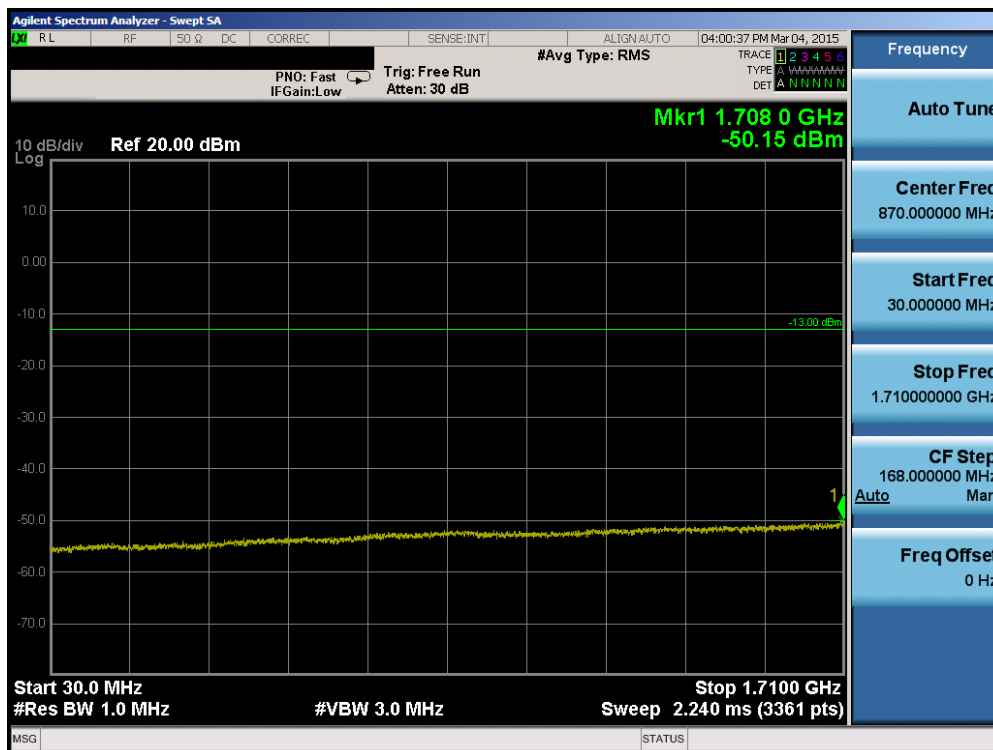
Plot 6-48. Conducted Spurious Plot (Band 4 – 20.0MHz QPSK – RB Size 1, RB Offset 0 – High Channel)
