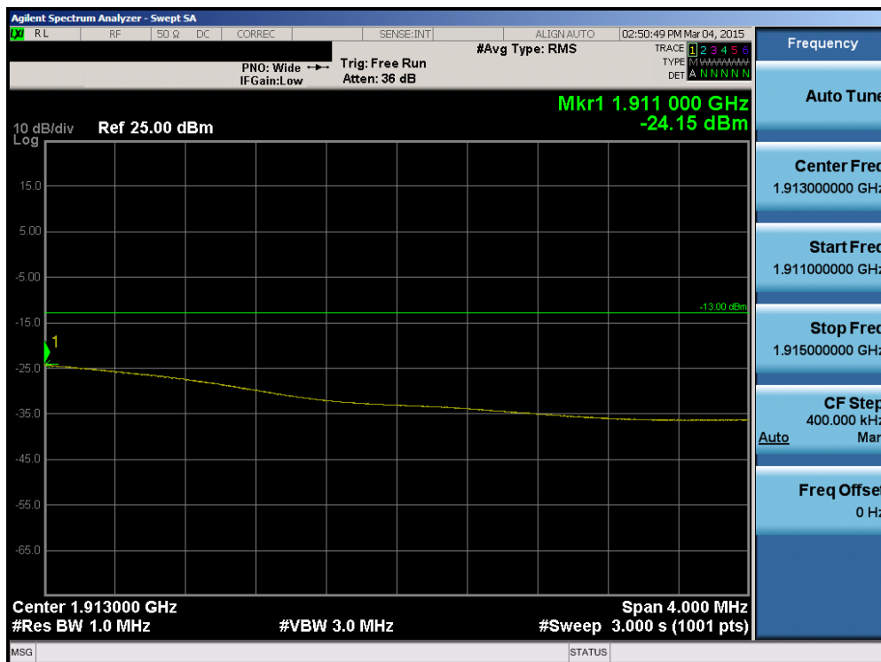
Plot 6-111. Upper Extended Band Edge Plot (Band 2 – 15.0MHz QPSK – RB Size 75)
