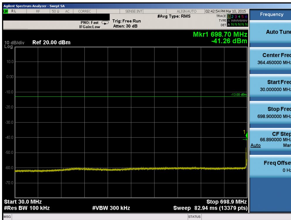
Plot 6-36. Conducted Spurious Plot (Band 12 – 10.0MHz QPSK – RB Size 1, RB Offset 0 – Mid Channel)
