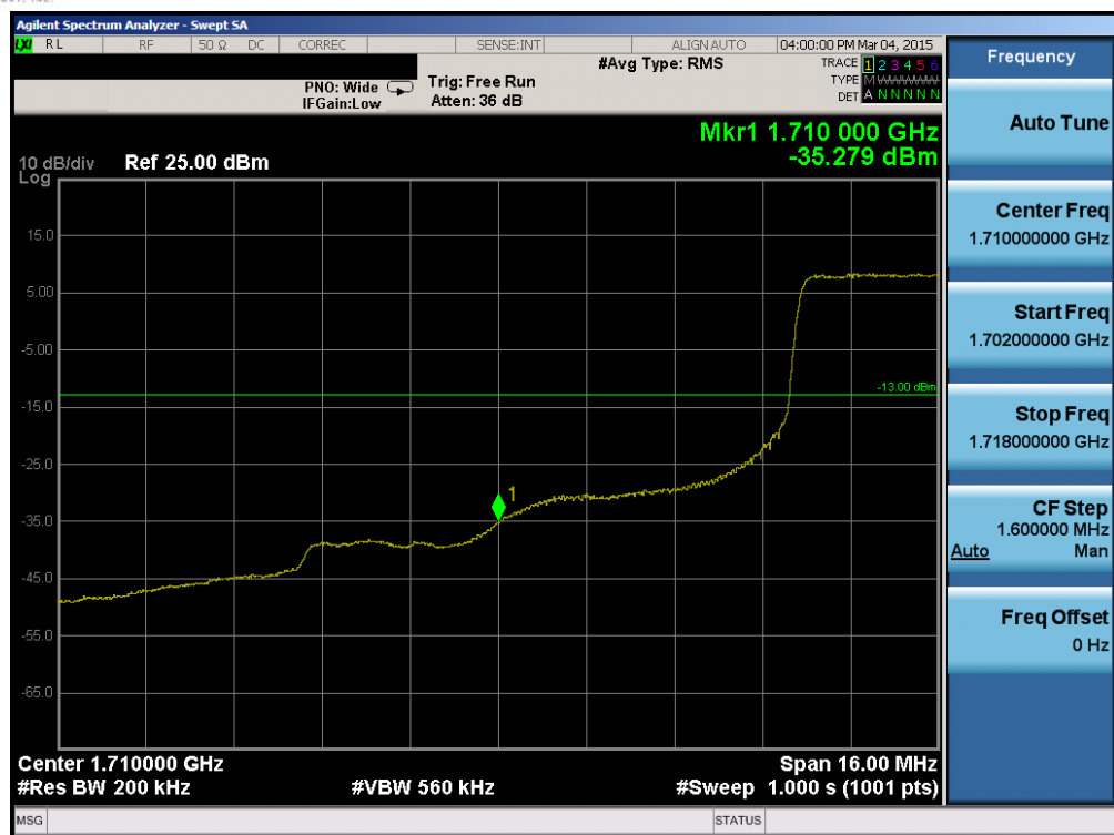
Plot 6-88. Lower Band Edge Plot (Band 4 – 20.0MHz QPSK – RB Size 100)
