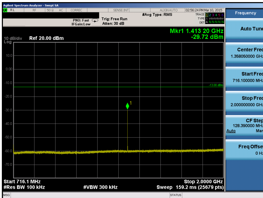
Plot 6-40. Conducted Spurious Plot (Band 12 – 10.0MHz QPSK – RB Size 1, RB Offset 0 – High Channel)
