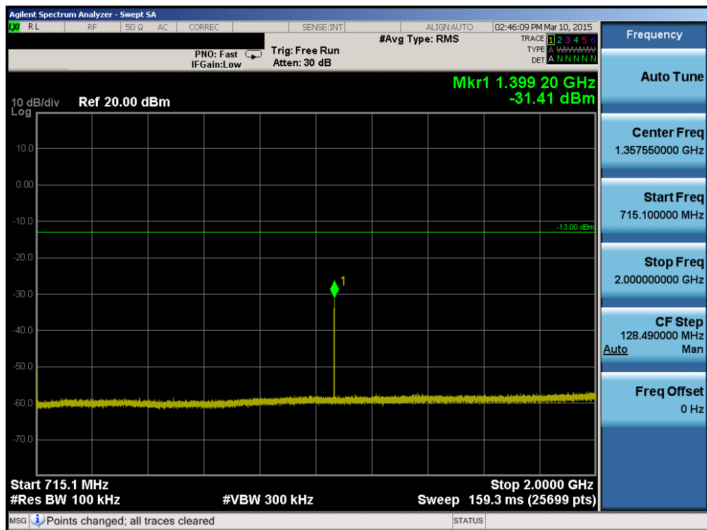
Plot 6-34. Conducted Spurious Plot (Band 12 – 10.0MHz QPSK – RB Size 1, RB Offset 0 – Low Channel)
