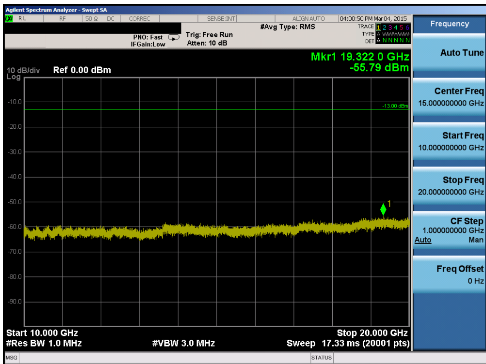
Plot 6-50. Conducted Spurious Plot (Band 4 – 20.0MHz QPSK – RB Size 1, RB Offset 0 – High Channel)
