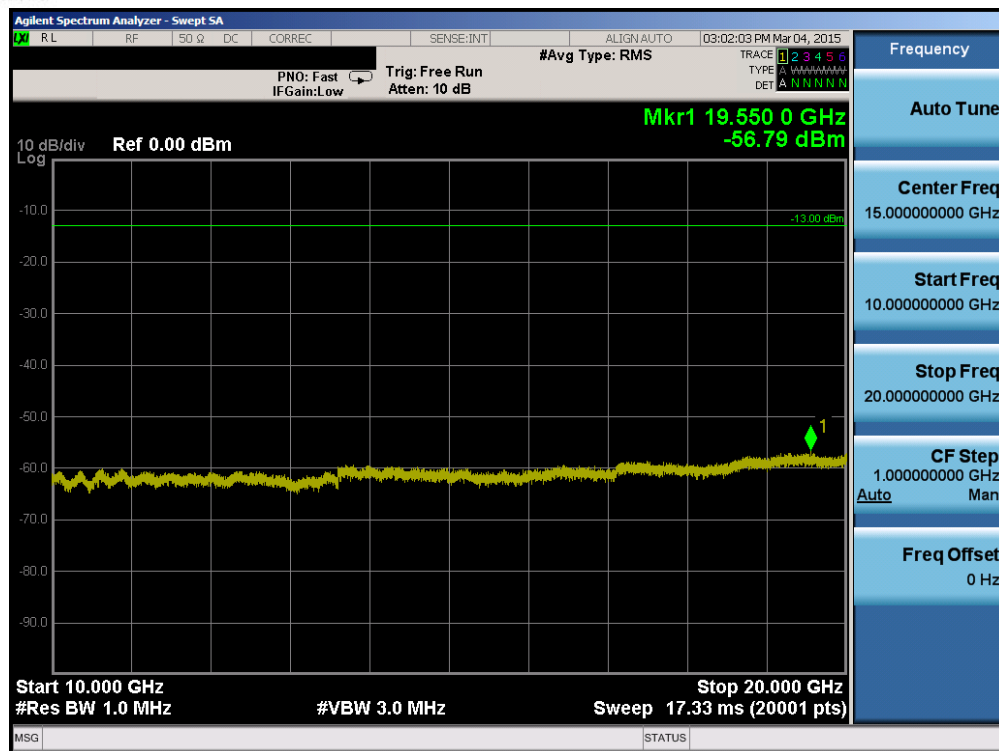
Plot 6-59. Conducted Spurious Plot (Band 2 – 20.0MHz QPSK – RB Size 1, RB Offset 0 – High Channel)
