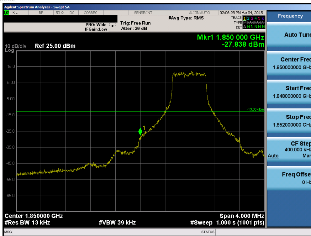
Plot 6-92. Lower Band Edge Plot (Band 2 – 1.4MHz QPSK – RB Size 6)
