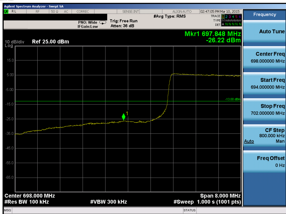
Plot 6-66. Lower Band Edge Plot (Band 12 – 10.0MHz QPSK – RB Size 50)
