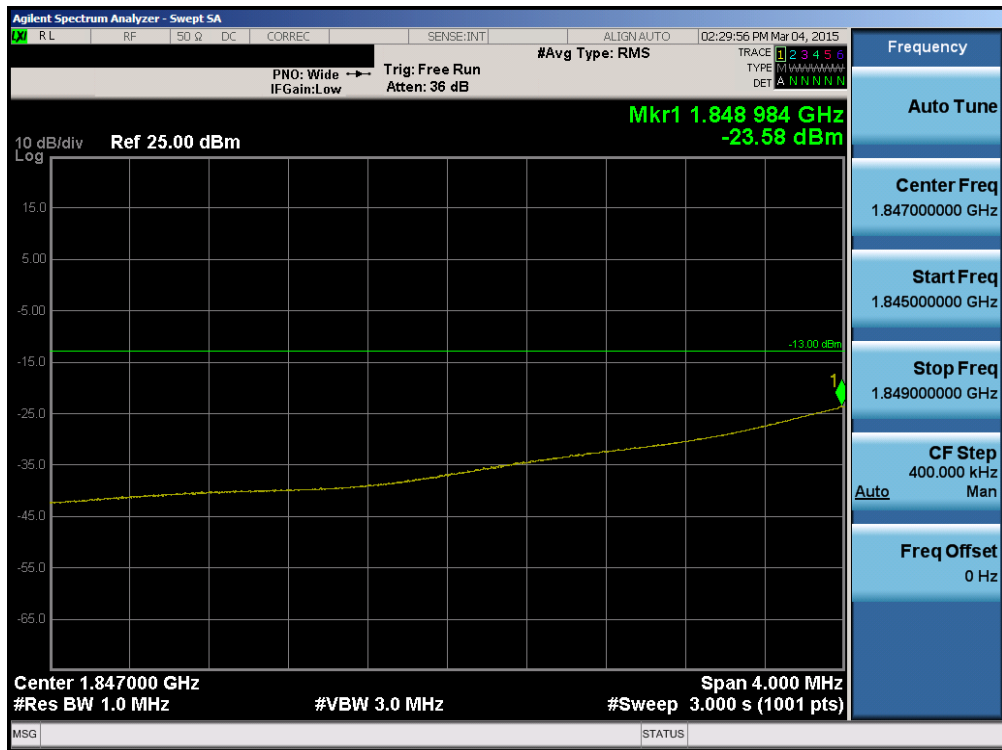
Plot 6-101. Lower Extended Band Edge Plot (Band 2 – 5.0MHz QPSK – RB Size 25)
