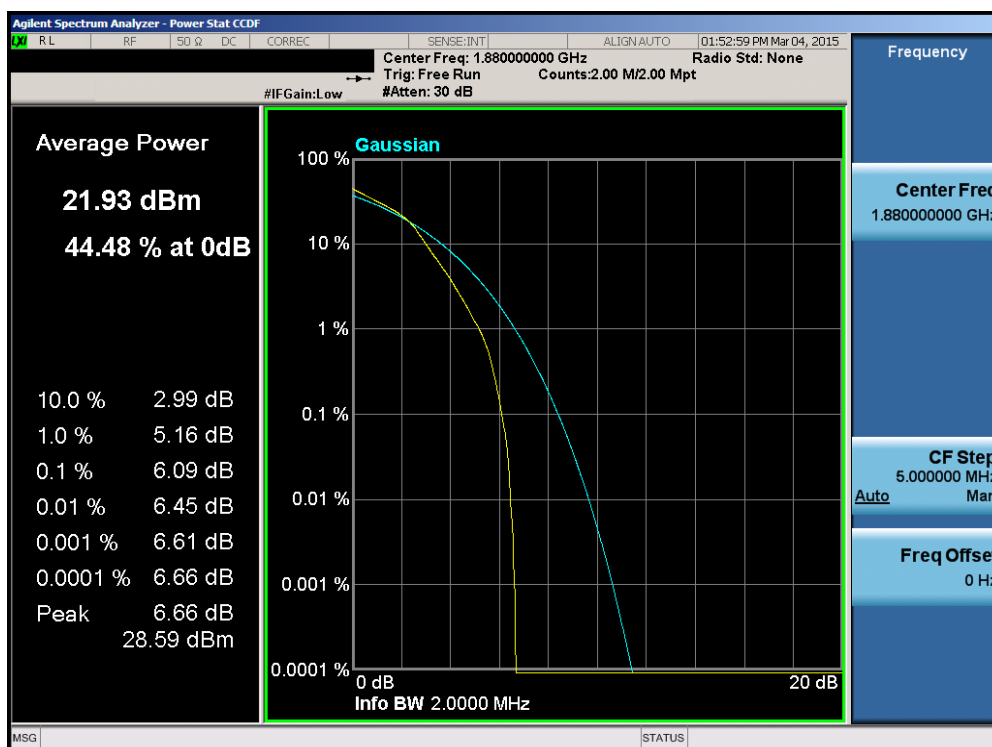
Plot 6-117. PAR Plot (Band 2 – 1.4MHz 16-QAM – RB Size 6)
