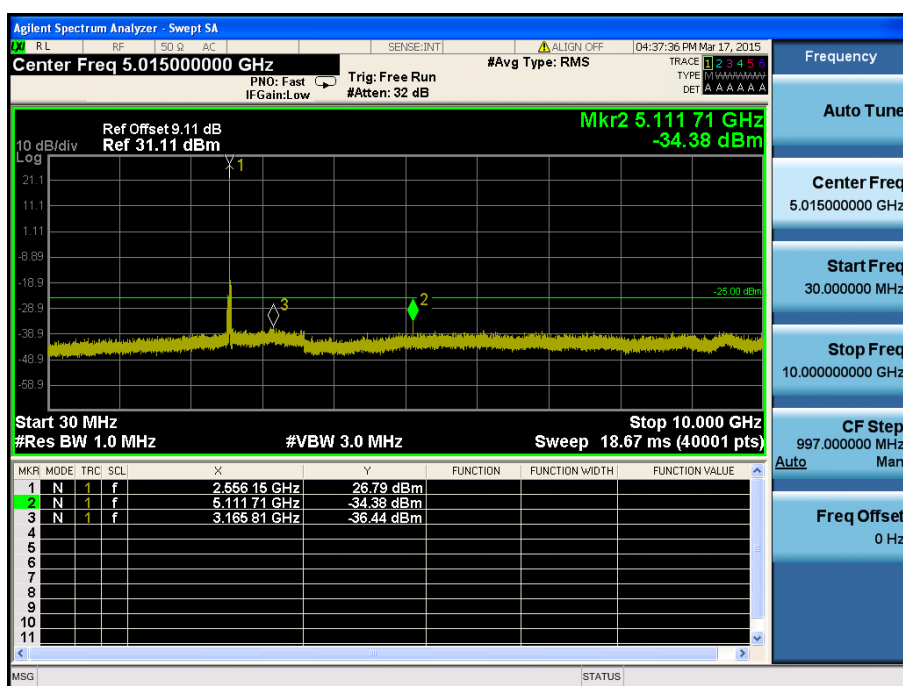
LTE Band 7 / 15MHz / QPSK - RB Size/Offset (1/0) – High Channel
