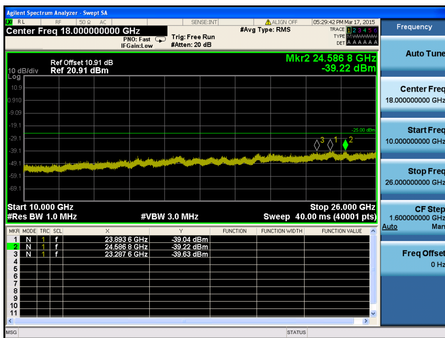
LTE Band 7 / 5MHz / 16QAM - RB Size/Offset (1/24) – Mid Channel
