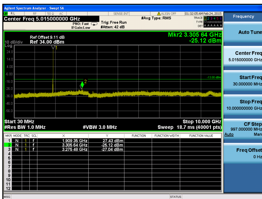
LTE Band 2 / 15MHz / 16QAM - RB Size/Offset (1/74) – High Channel
