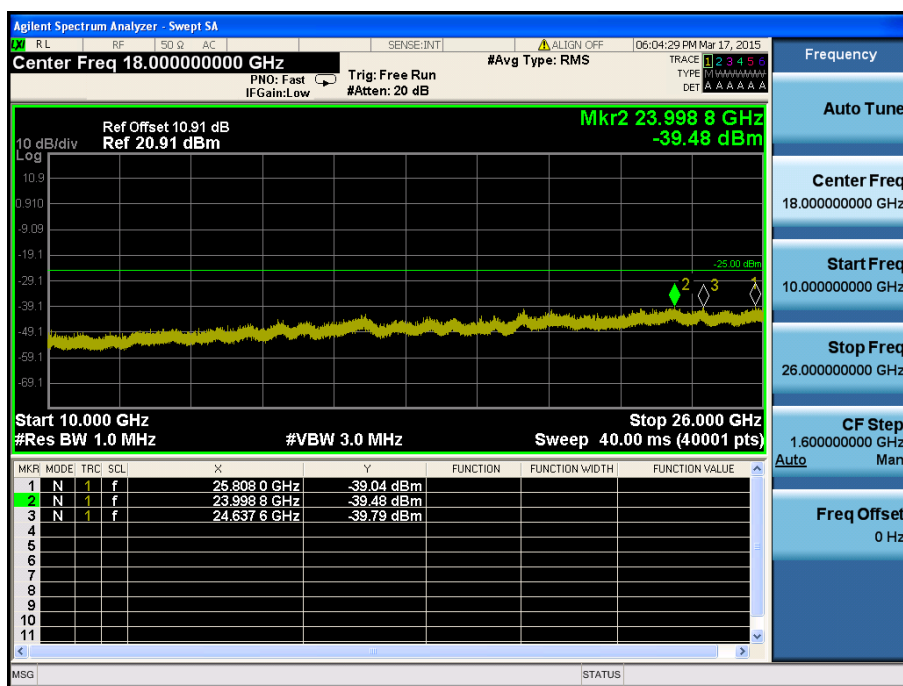
LTE Band 7 / 10MHz / 16QAM - RB Size/Offset (1/25) – High Channel
