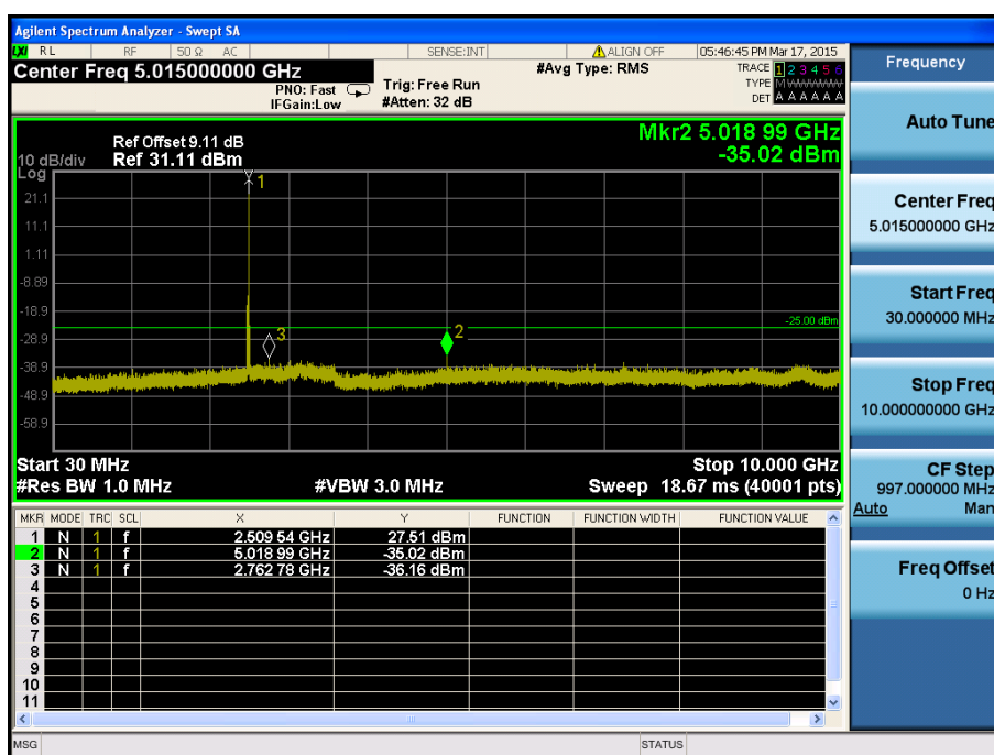
LTE Band 7 / 10MHz / 16QAM - RB Size/Offset (1/49) – Low Channel
