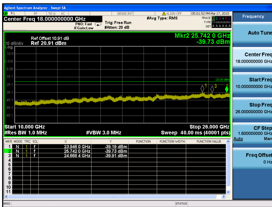
LTE Band 7 / 20MHz / QPSK - RB Size/Offset (1/99) – Mid Channel
