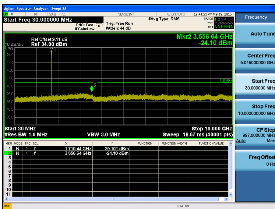
LTE Band 4 / 1.4MHz / 16QAM - RB Size/Offset (1/0) – Low Channel
