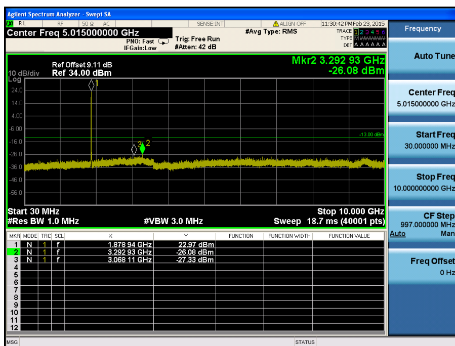
LTE Band 2 / 5MHz / 16QAM - RB Size/Offset (25/0) – Mid Channel
