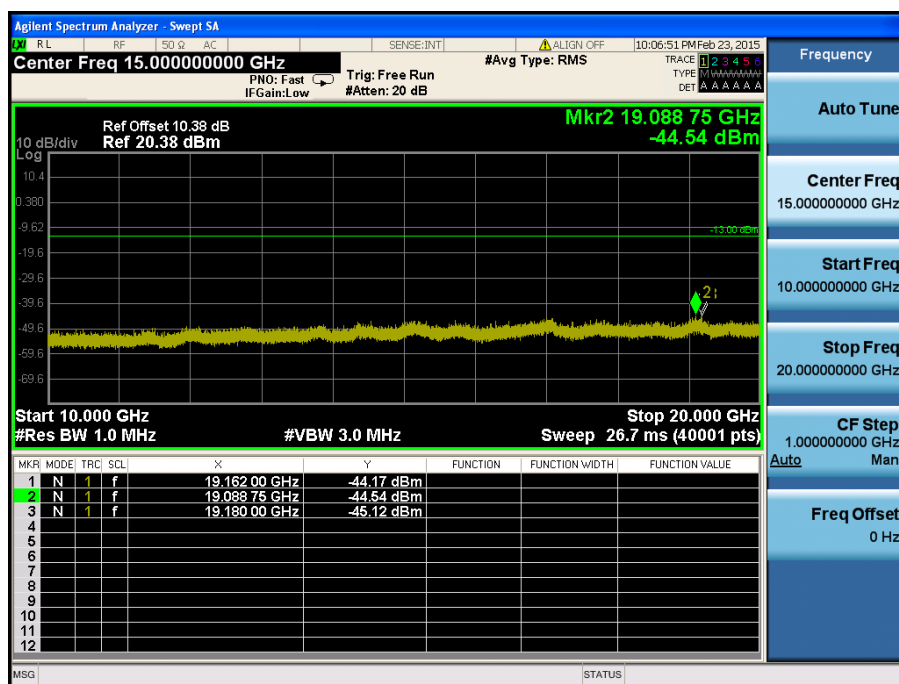
LTE Band 2 / 3MHz / 16QAM - RB Size/Offset (1/0) – Low Channel
