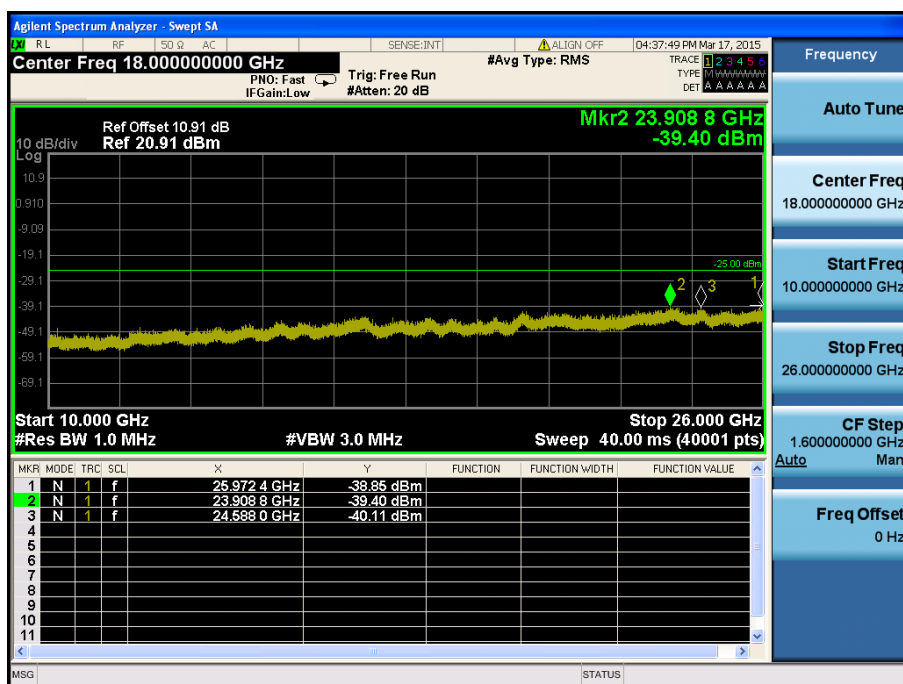
LTE Band 7 / 15MHz / QPSK - RB Size/Offset (1/0) – High Channel
