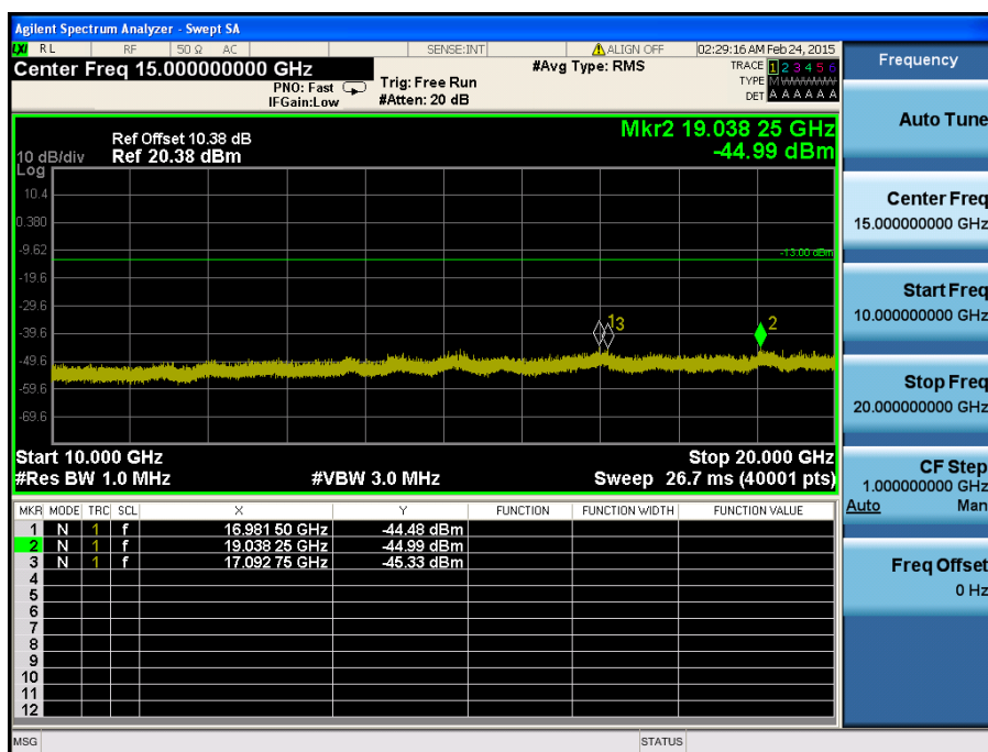
LTE Band 2 / 20MHz / 16QAM - RB Size/Offset (1/99) – High Channel
