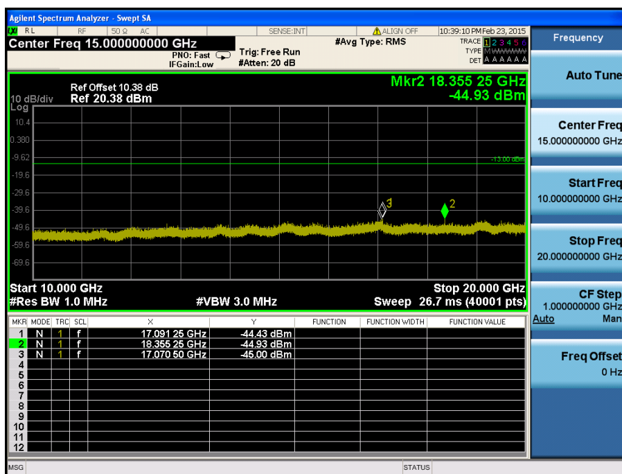
LTE Band 2 / 3MHz / 16QAM - RB Size/Offset (1/0) – High Channel
