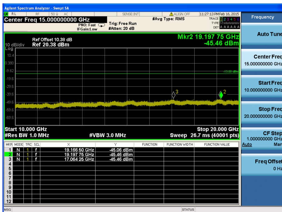
LTE Band 2 / 15MHz / QPSK - RB Size/Offset (1/37) – Mid Channel
