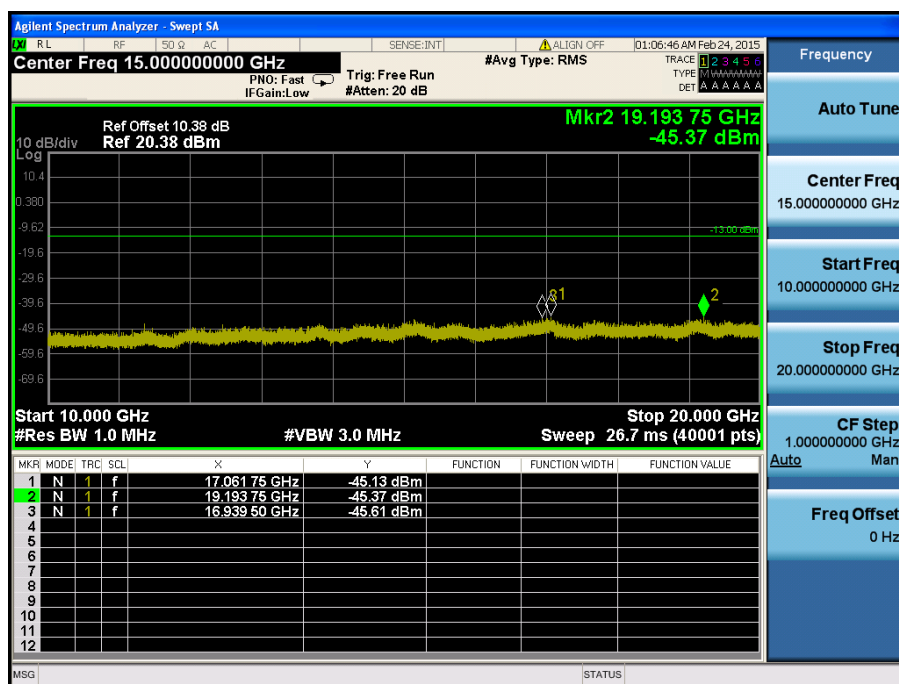
LTE Band 2 / 15MHz / 16QAM - RB Size/Offset (36/19) – Low Channel
