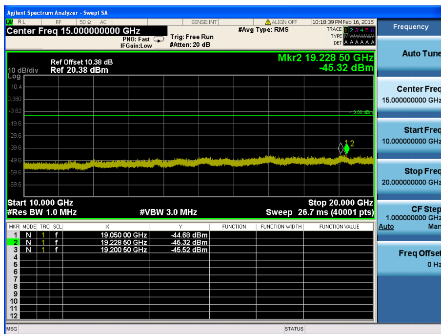
LTE Band 2 / 10MHz / QPSK - RB Size/Offset (25/0) – Low Channel
