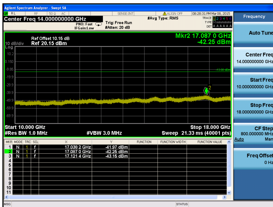
LTE Band 4 / 1.4MHz / QPSK - RB Size/Offset (1/3) – Mid Channel
