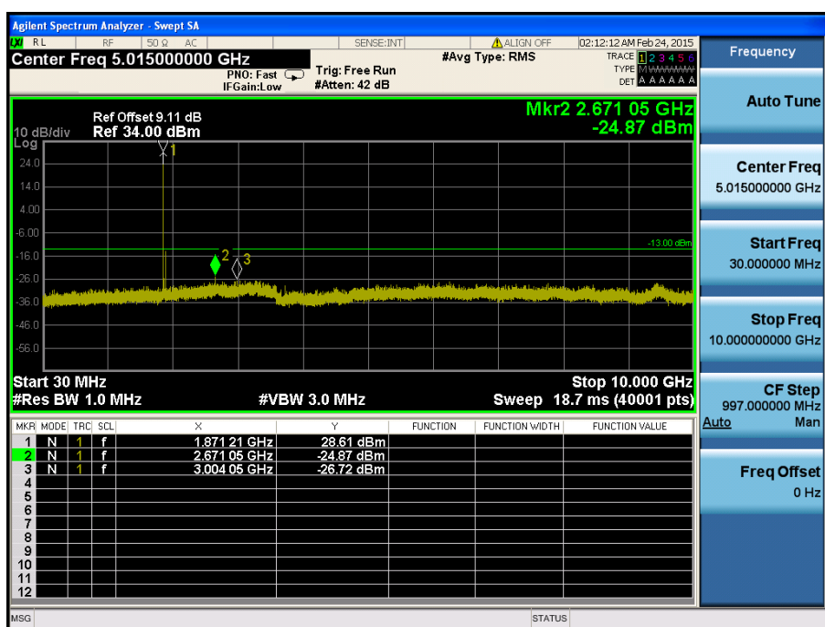
LTE Band 2 / 20MHz / 16QAM - RB Size/Offset (1/0) – Mid Channel
