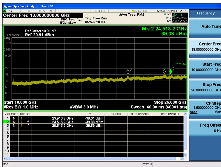
LTE Band 7 / 10MHz / 16QAM - RB Size/Offset (1/49) – Mid Channel
