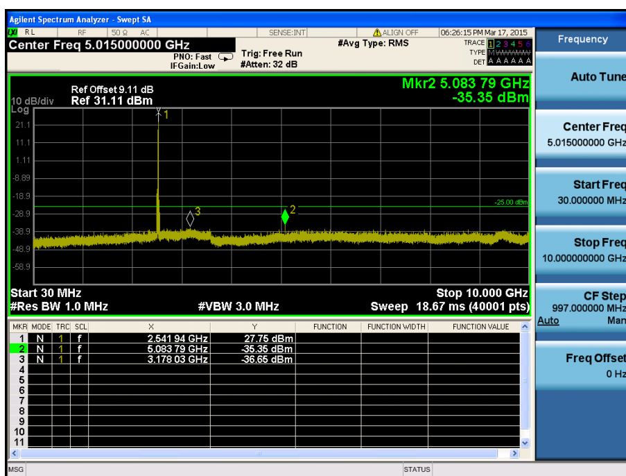
LTE Band 7 / 15MHz / 16QAM - RB Size/Offset (1/74) – Mid Channel
