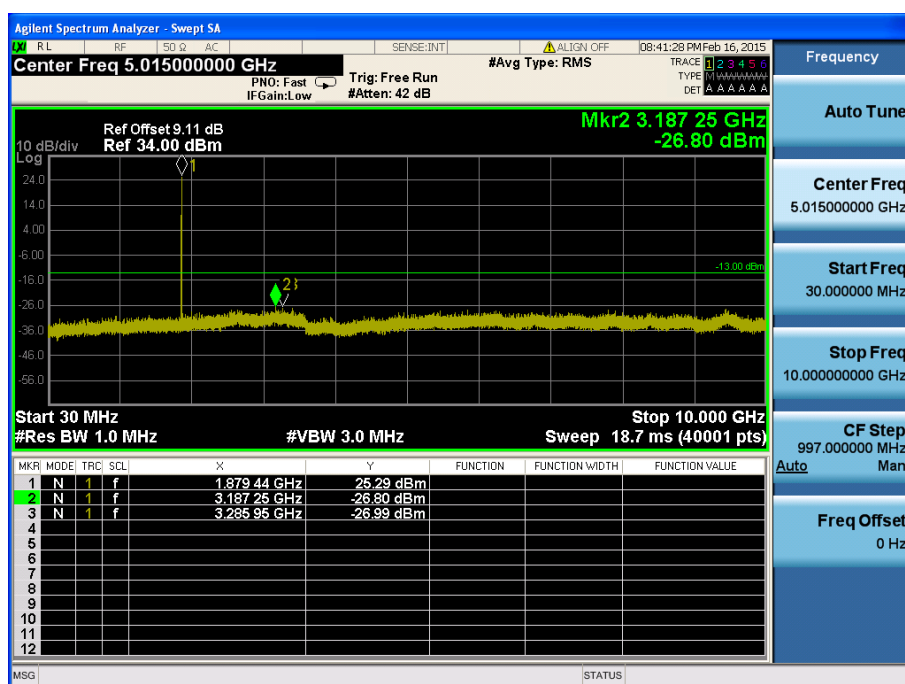
LTE Band 2 / 3MHz / QPSK - RB Size/Offset (8/0) – Mid Channel
