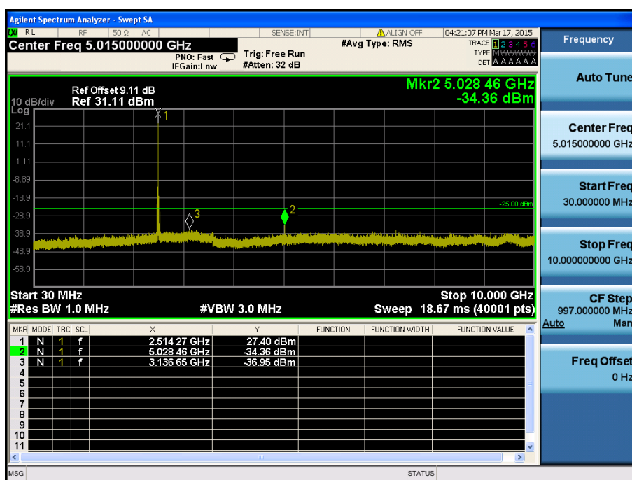
LTE Band 7 / 15MHz / QPSK - RB Size/Offset (1/74) – Low Channel
