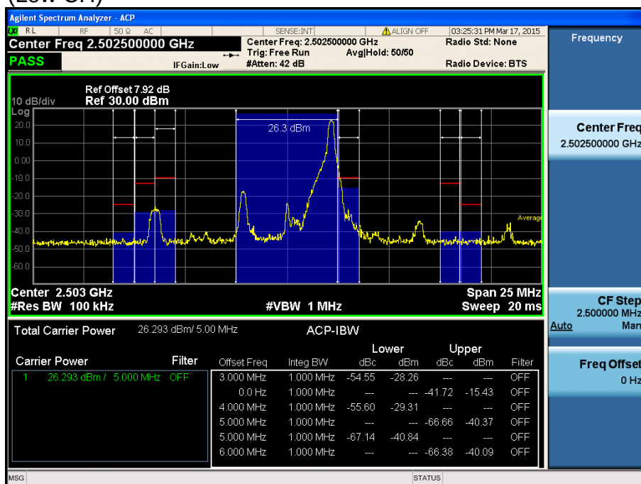
LTE Band 7 / 5MHz / QPSK - RB Size/Offset (1/24)
