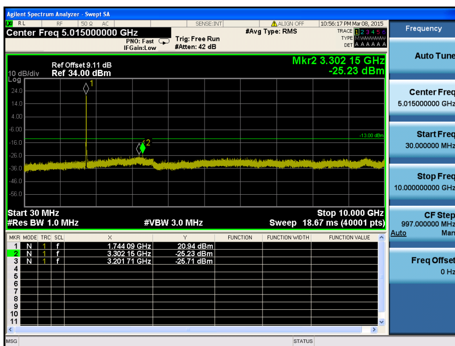
LTE Band 4 / 20MHz / 16QAM - RB Size/Offset (50/25) – High Channel
