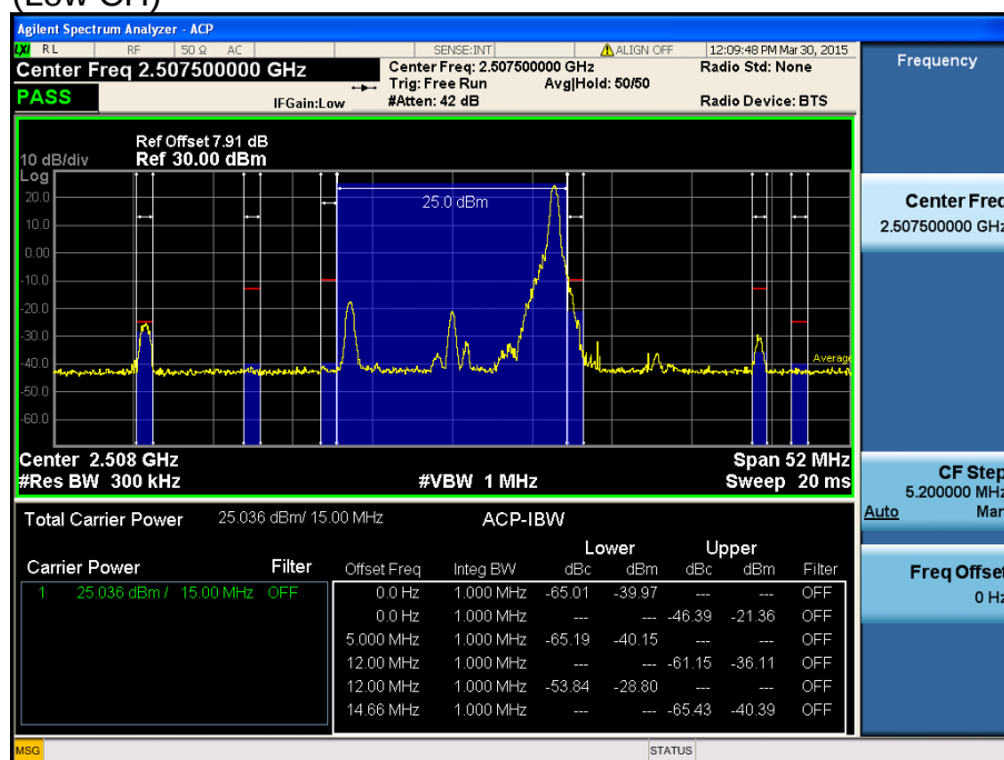
LTE Band 7 / 15MHz / 16QAM - RB Size/Offset (1/74)
