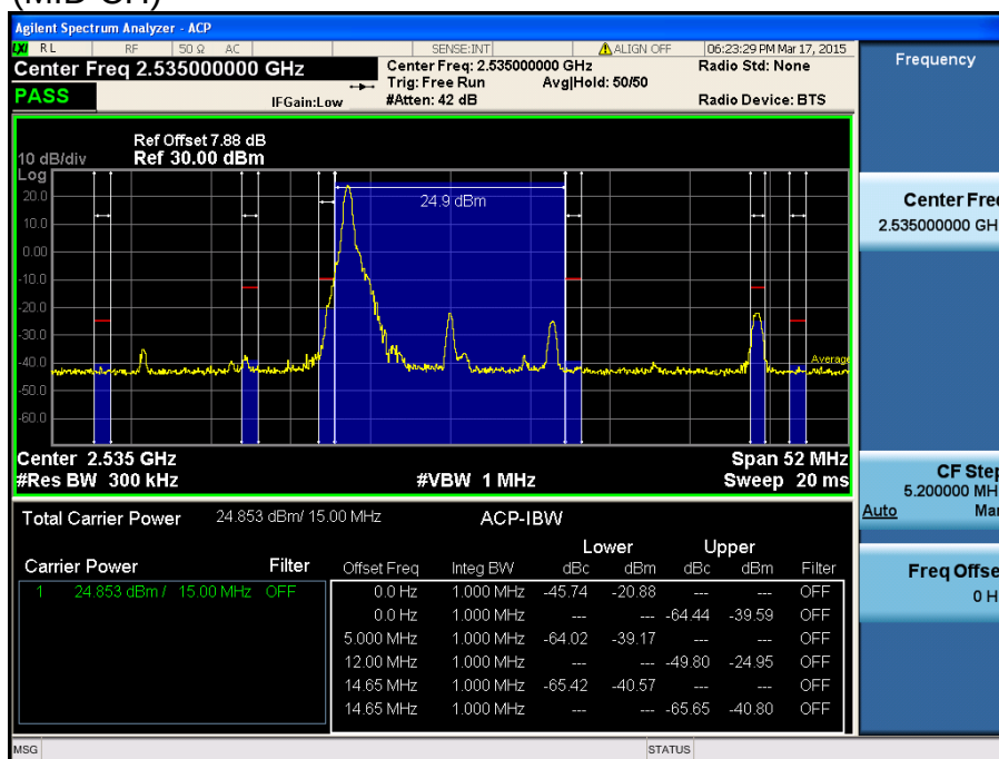
LTE Band 7 / 15MHz / 16QAM - RB Size/Offset (1/0)
