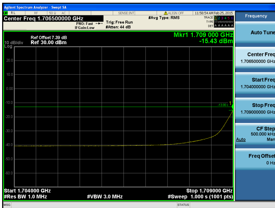
LTE Band 4 / 1.4MHz / QPSK - RB Size/Offset (3/1)
