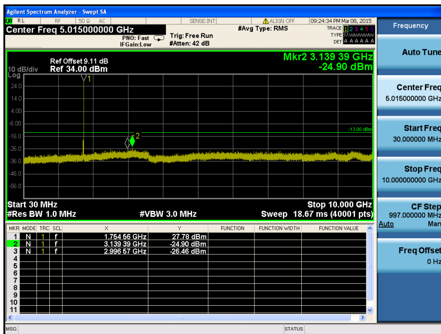
LTE Band 4 / 15MHz / QPSK - RB Size/Offset (1/74) – High Channel
