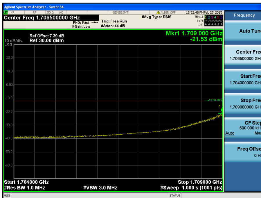
LTE Band 4 / 3MHz / QPSK - RB Size/Offset (8/3)
