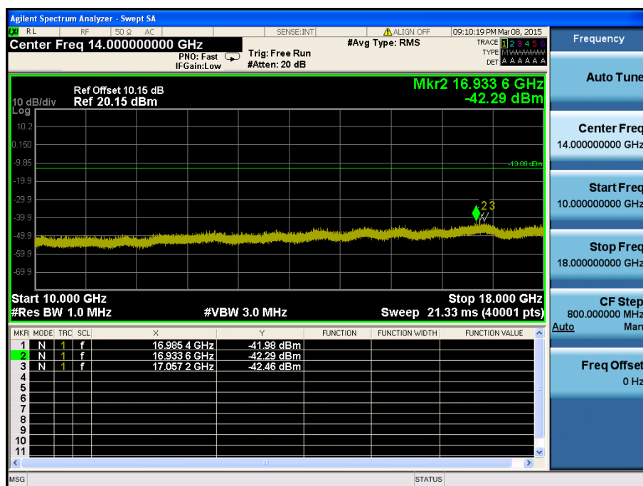
LTE Band 4 / 10MHz / QPSK - RB Size/Offset (1/0) – High Channel
