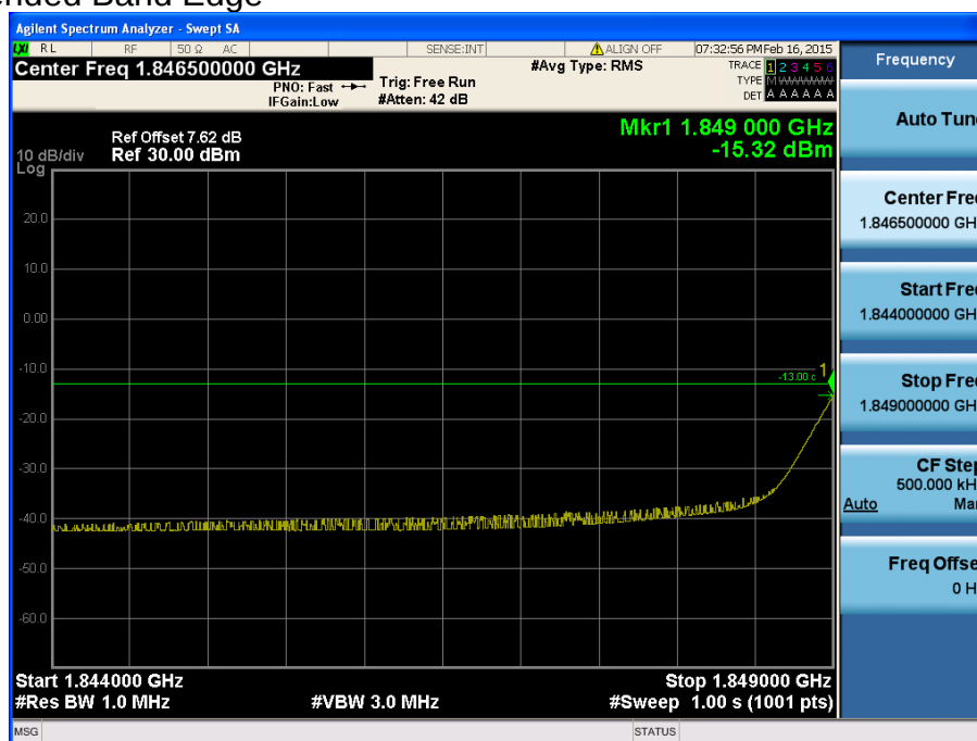
LTE Band 2 / 1.4MHz / QPSK - RB Size/Offset (3/1)
