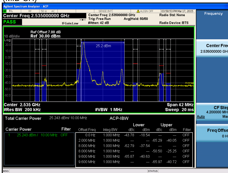
LTE Band 7 / 10MHz / QPSK - RB Size/Offset (1/0)
