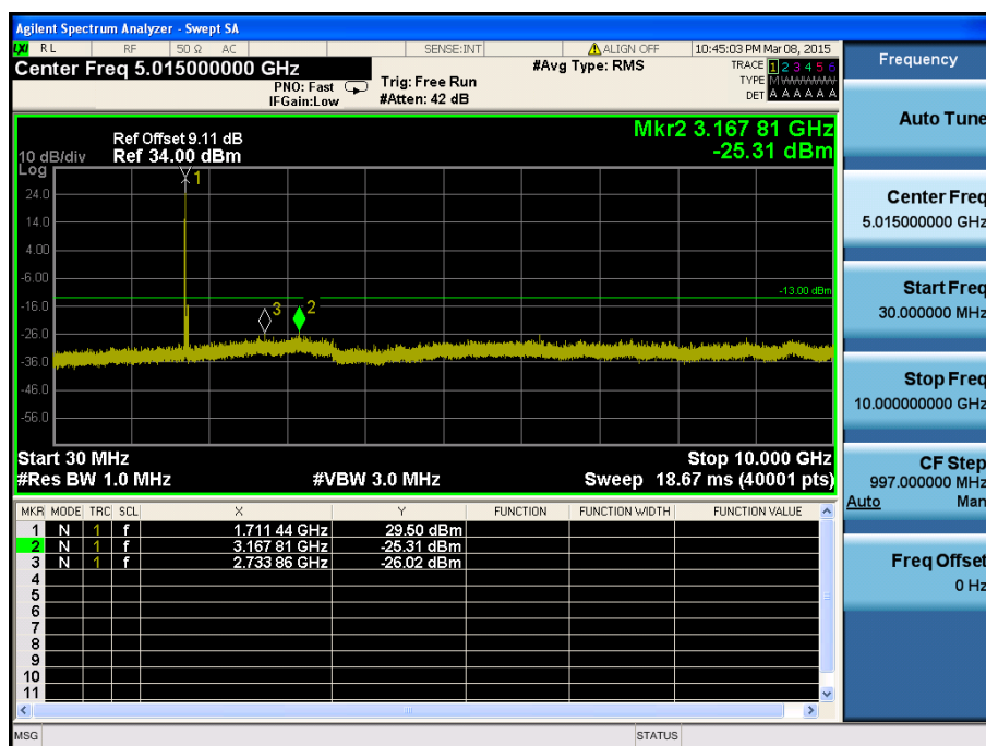
LTE Band 4 / 20MHz / 16QAM - RB Size/Offset (1/0) –Low Channel
