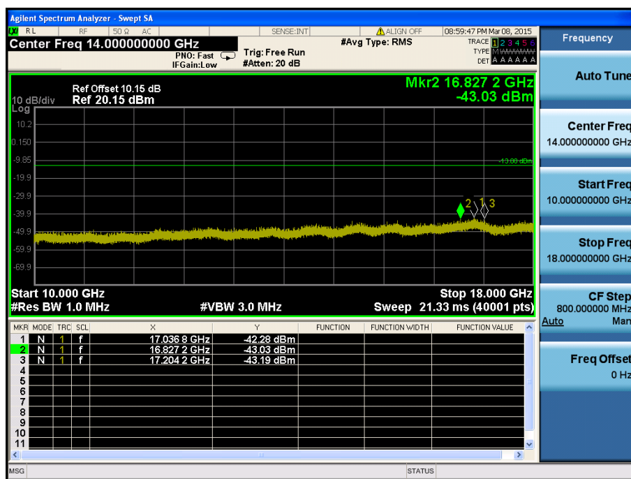
LTE Band 4 / 5MHz / QPSK - RB Size/Offset (12/6) – High Channel
