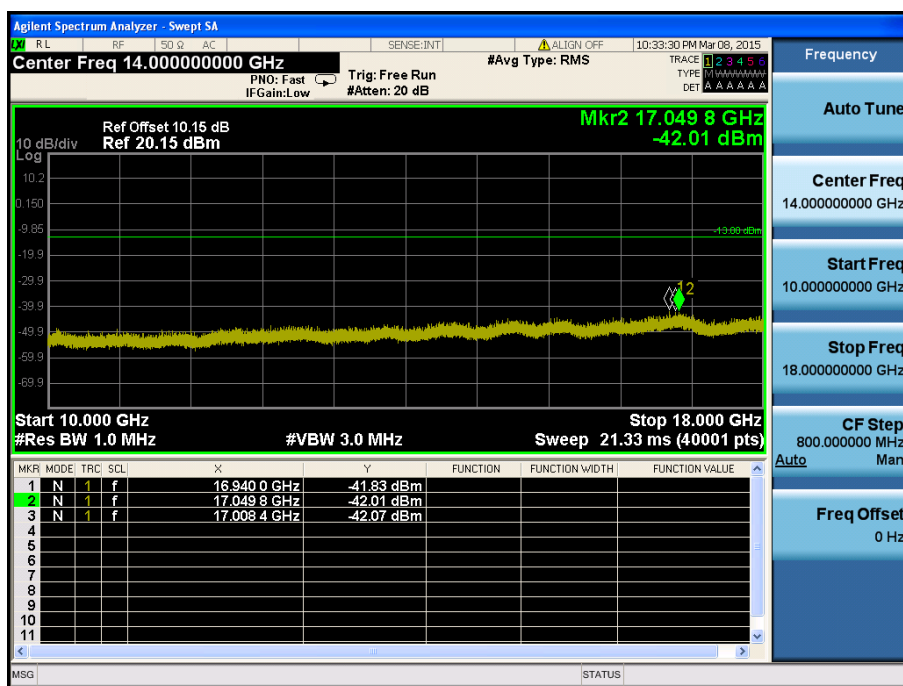
LTE Band 4 / 15MHz / QPSK - RB Size/Offset (1/74)–Low Channel
