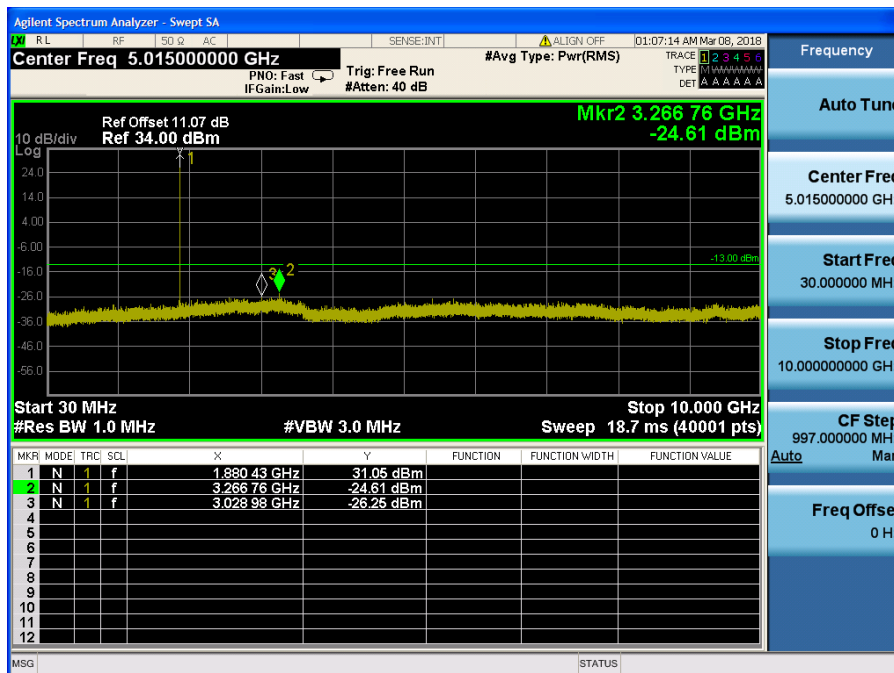
LTE Band 2 / 1.4MHz / 64QAM - RB Size/Offset (1/2) – Mid Channel
