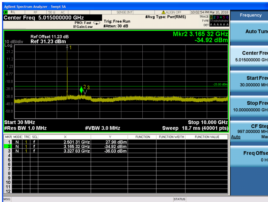
LTE Band 7 / 5MHz / 16QAM - RB Size/Offset (12/0) – Low Channel
