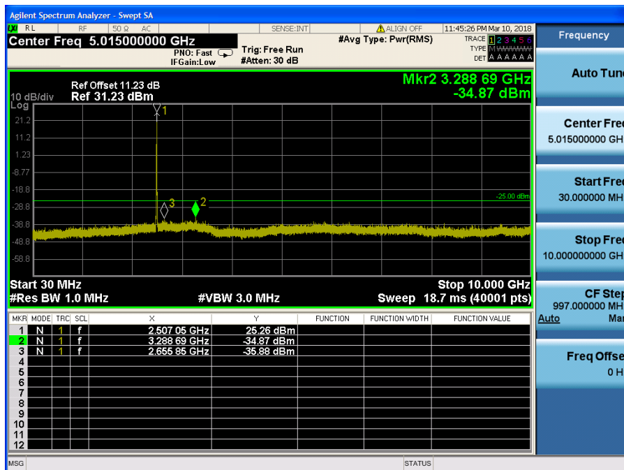
LTE Band 7 / 10MHz / 64QAM - RB Size/Offset (25/25) – Low Channel
