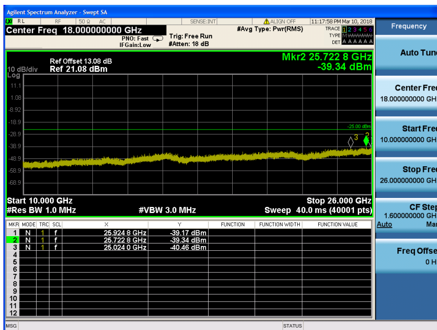
LTE Band 7 / 20MHz / 16QAM - RB Size/Offset (50/50) – High Channel
