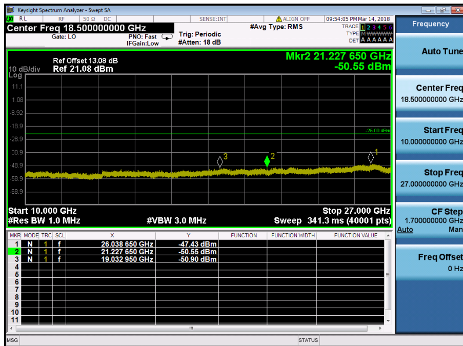
LTE Band 41 / 5MHz / QPSK - RB Size/Offset (1/0) – Mid Channel
