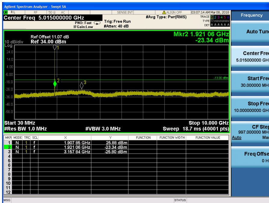
LTE Band 2 / 5MHz / 64QAM - RB Size/Offset (25/0) – High Channel
