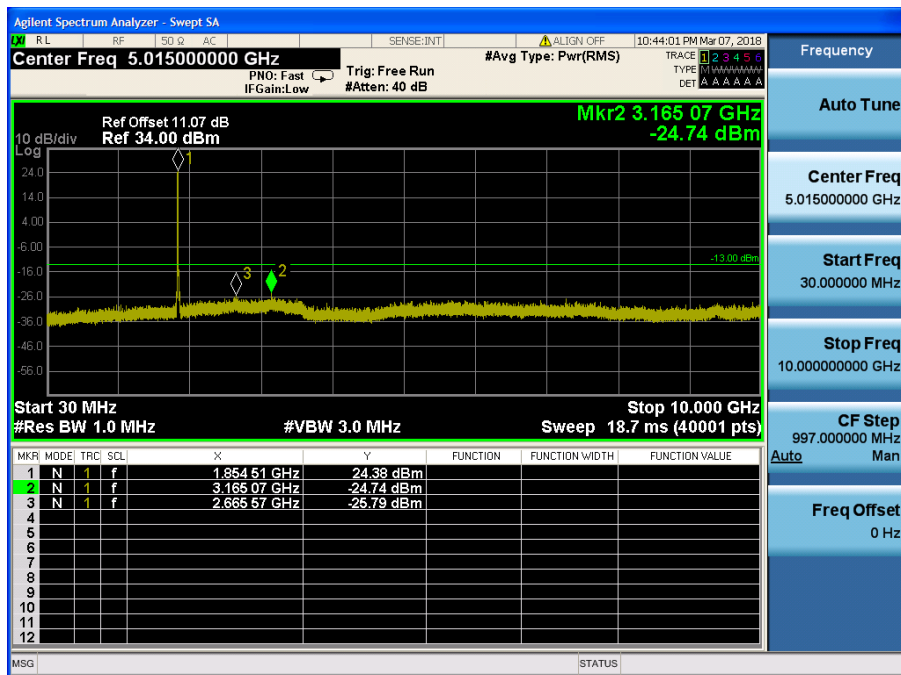
LTE Band 2 / 10MHz / 16QAM - RB Size/Offset (50/0) – Low Channel
