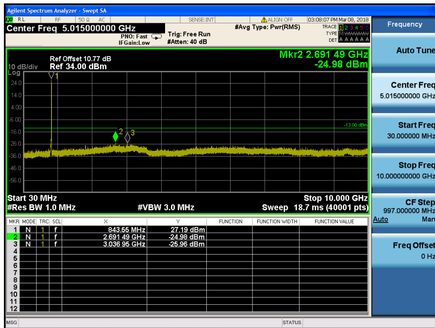
LTE Band 5 / 10MHz / 16QAM - RB Size/Offset (50/0) – High Channel
