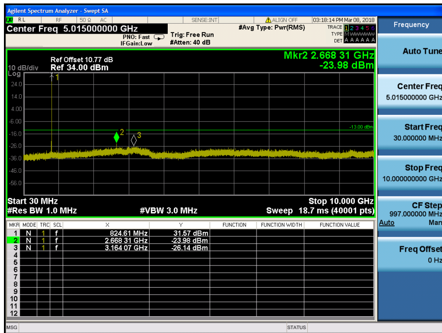
LTE Band 5 / 1.4MHz / 64QAM - RB Size/Offset (3/0) – Low Channel
