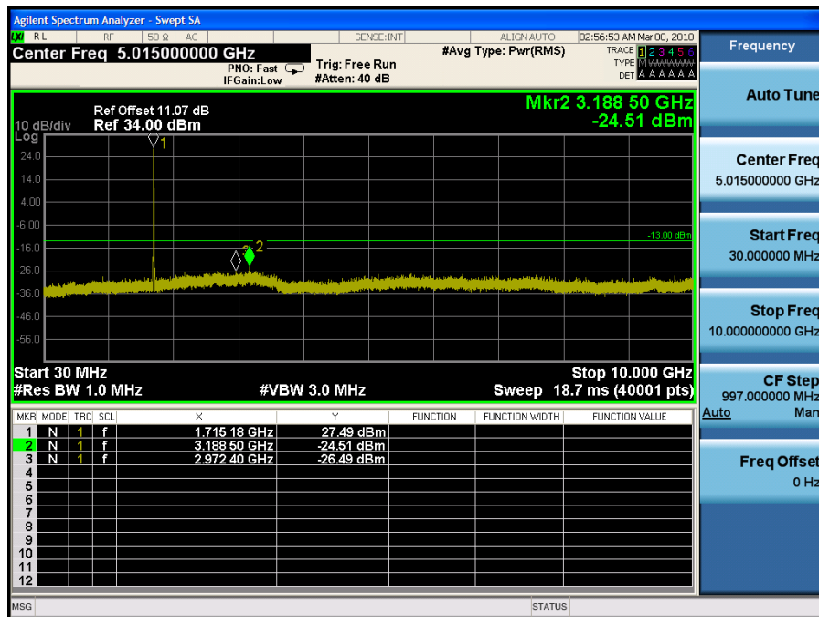
LTE Band 4 / 10MHz / 64QAM - RB Size/Offset (25/12) – Low Channel
