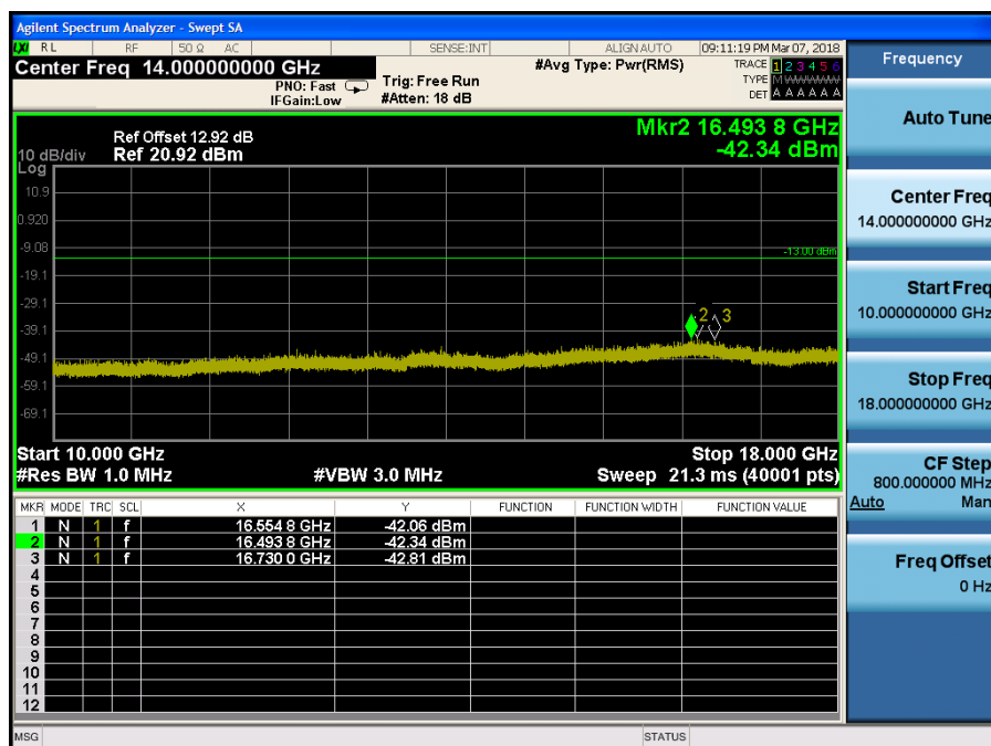
LTE Band 4 / 3MHz / 16QAM - RB Size/Offset (1/0) – Mid Channel
