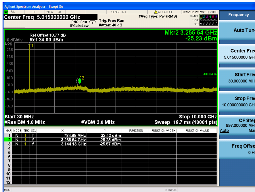
LTE Band 13 / 5MHz / 64QAM - RB Size/Offset (1/12) – High Channel
