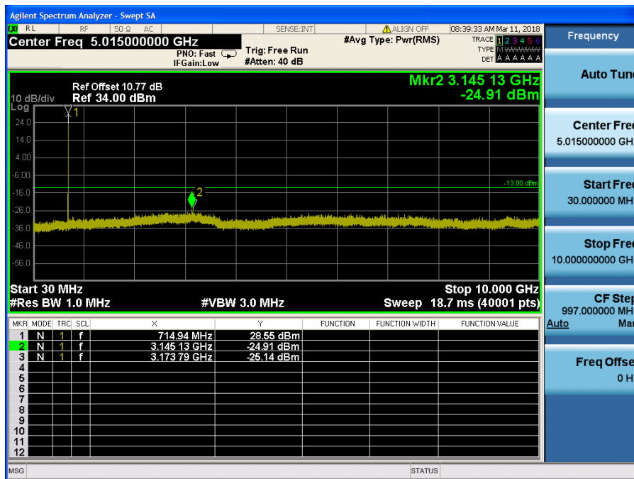
LTE Band 17 / 5MHz / 64QAM - RB Size/Offset (12/13) – High Channel
