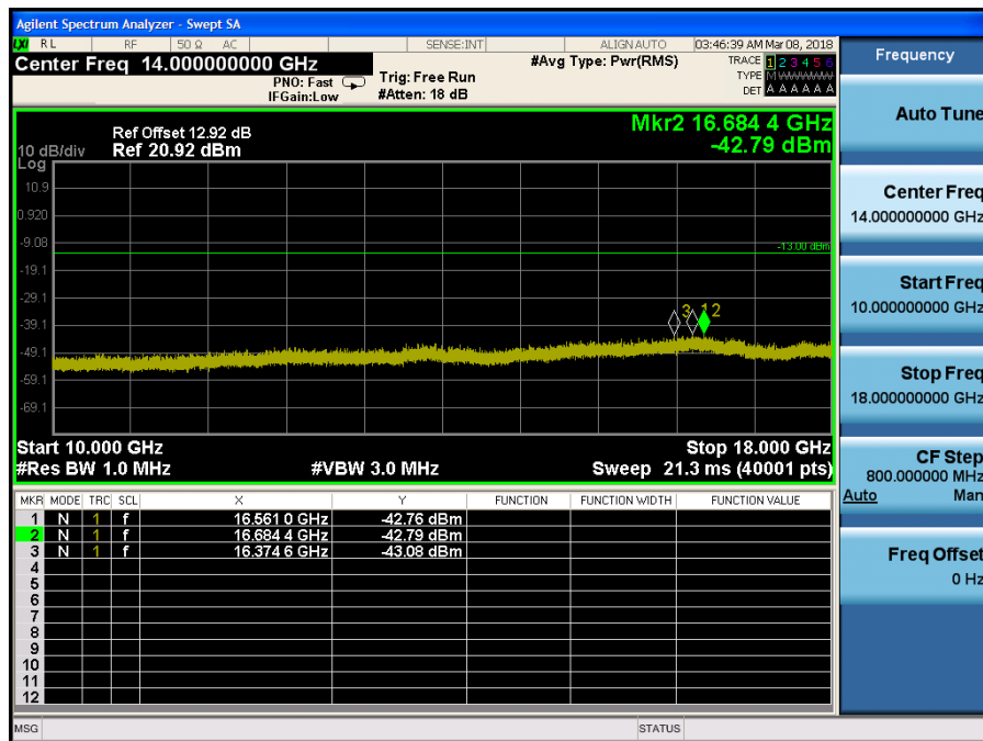
LTE Band 4 / 15MHz / 64QAM - RB Size/Offset (75/0)–Low Channel
