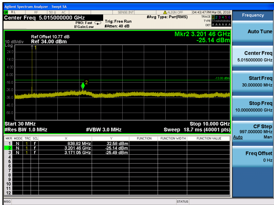
LTE Band 5 / 5MHz / 64QAM - RB Size/Offset (1/24) – Mid Channel
