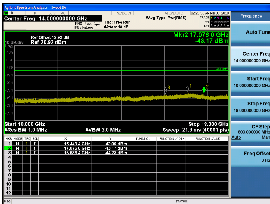
LTE Band 4 / 5MHz / 64QAM - RB Size/Offset (1/24) – Mid Channel
