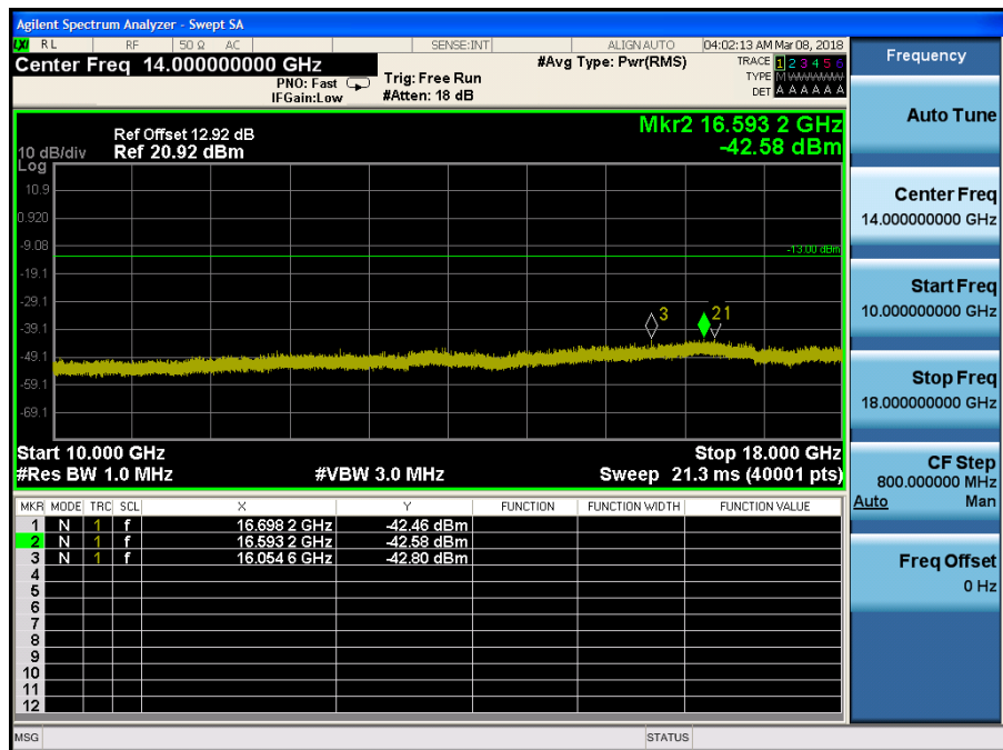
LTE Band 4 / 15MHz / 64QAM - RB Size/Offset (36/0) – High Channel
