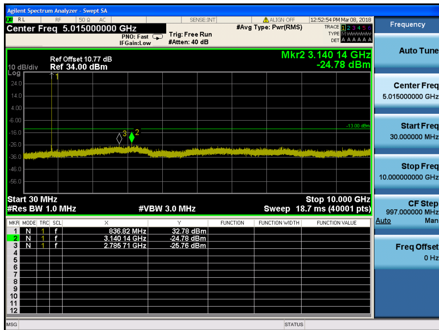
LTE Band 5 / 1.4MHz / 16QAM - RB Size/Offset (1/2) – Mid Channel
