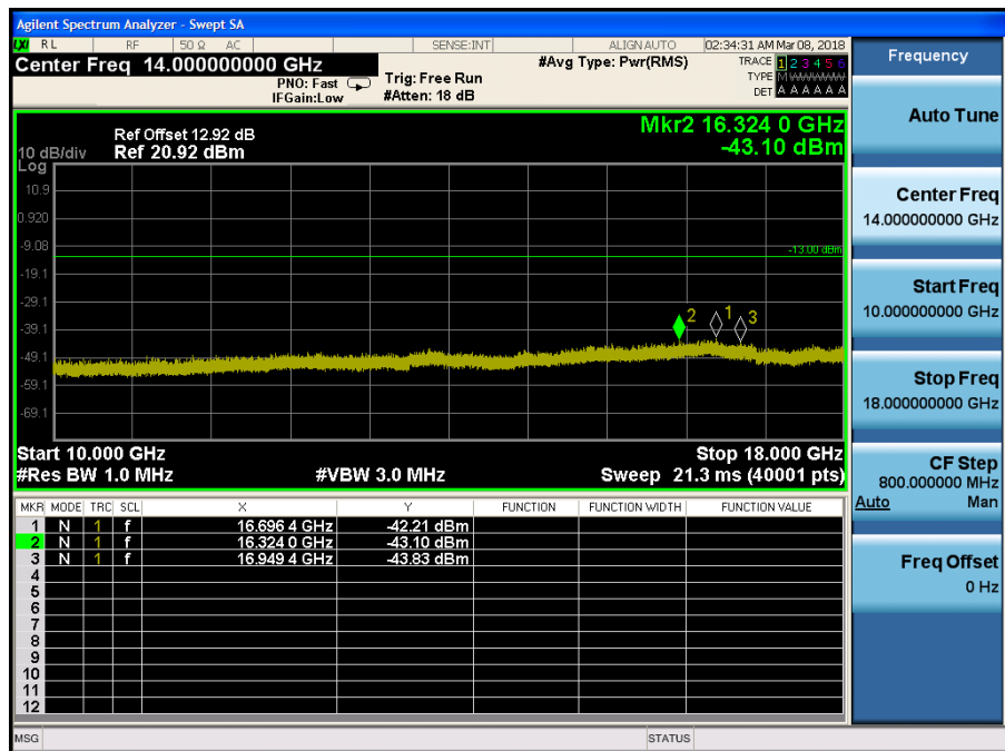
LTE Band 4 / 5MHz / 64QAM - RB Size/Offset (12/0) – High Channel
