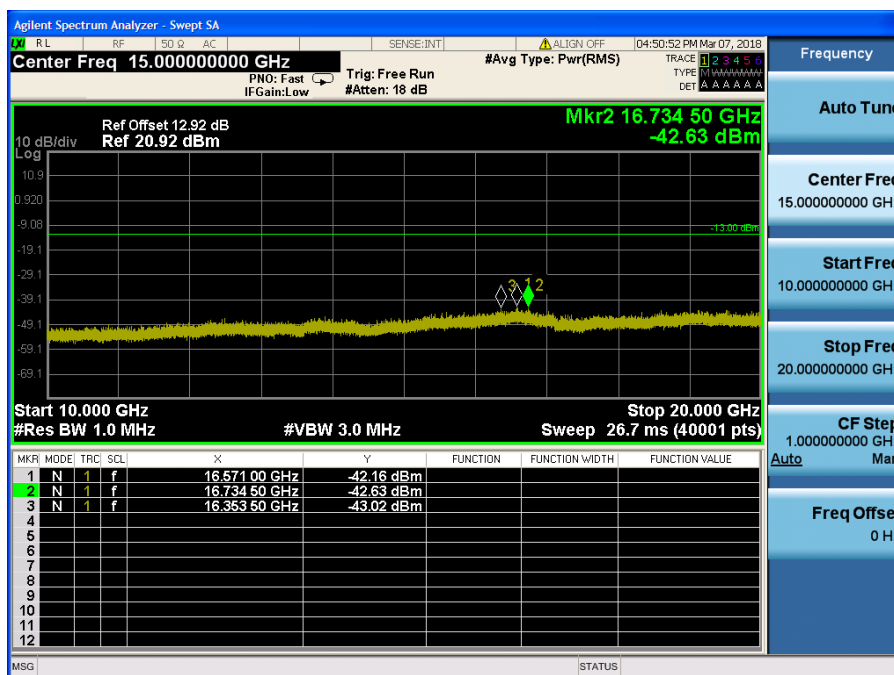
LTE Band 2 / 5MHz / QPSK - RB Size/Offset (12/13) – Low Channel
