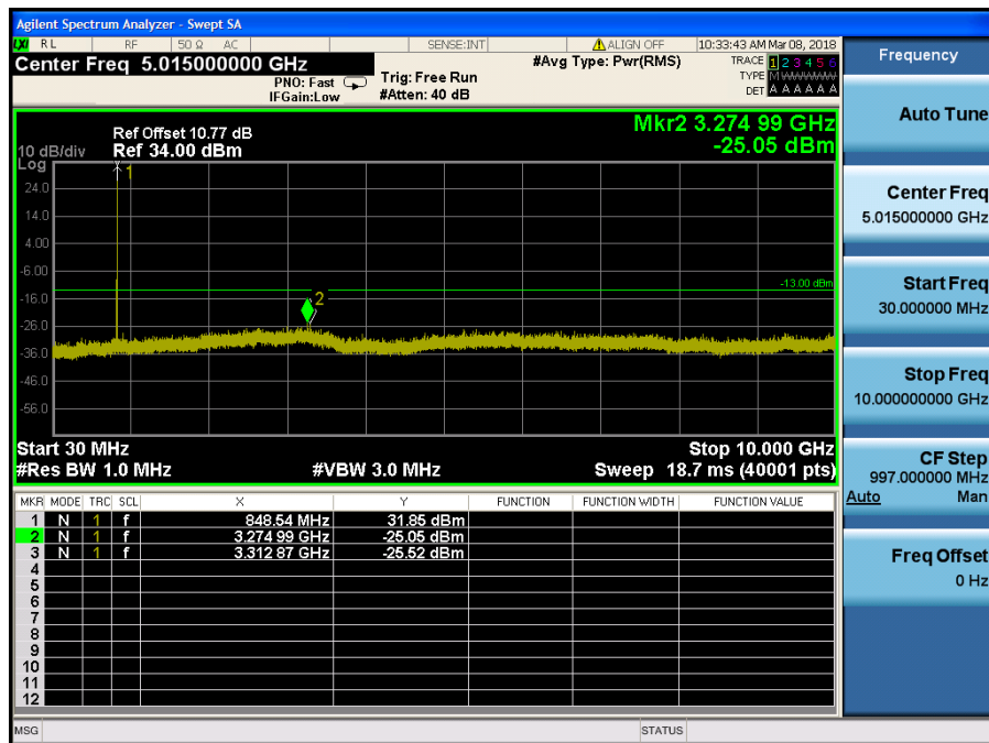
LTE Band 5 / 1.4MHz / QPSK - RB Size/Offset (3/2) – High Channel
