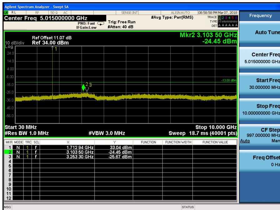
LTE Band 4 / 3MHz / 16QAM - RB Size/Offset (1/14) – Low Channel
