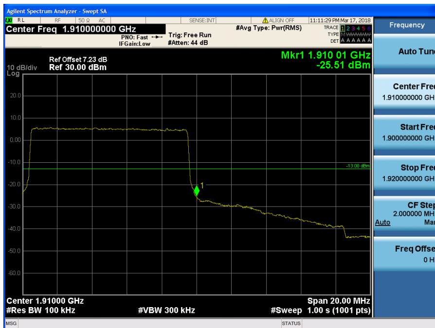
LTE Band 2 / 10MHz / QPSK - RB Size/Offset (50/0)
