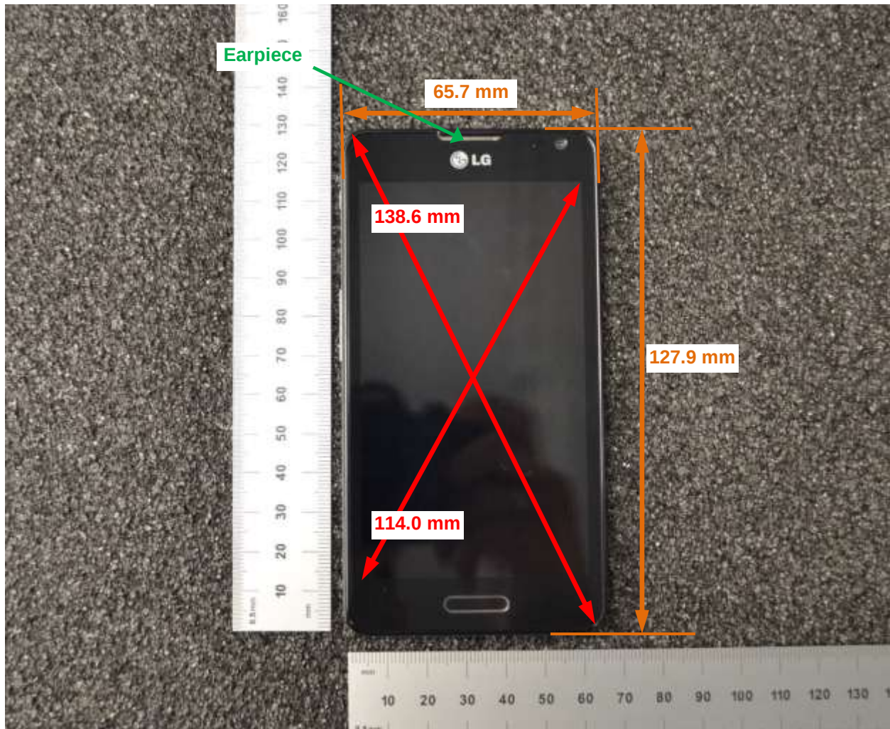
Overall Dimensions
