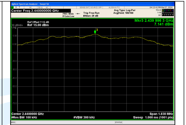
In-Band Reference Level 2LE_Channel 19
