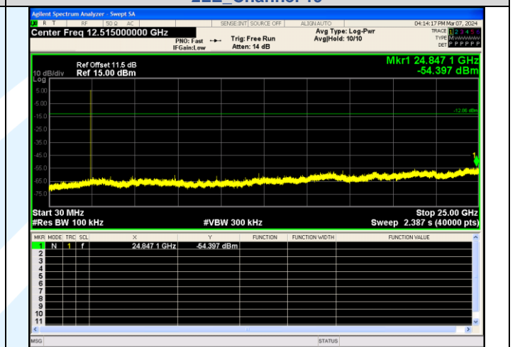
Spurious Emissions 2LE_Channel 19
