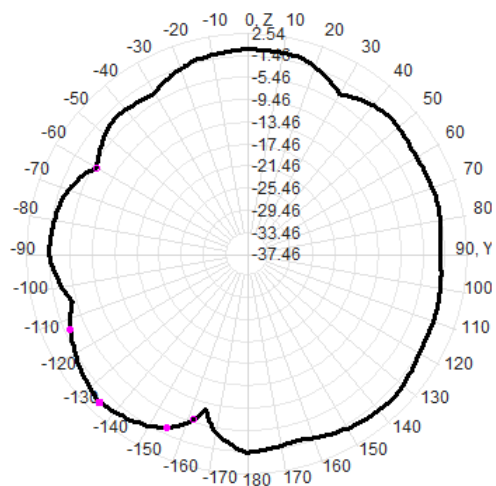
2.4G phi=90deg
