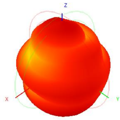
2.4G 3D
