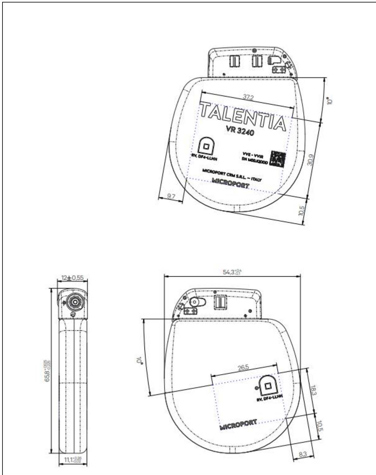
Dimensions (mm)
