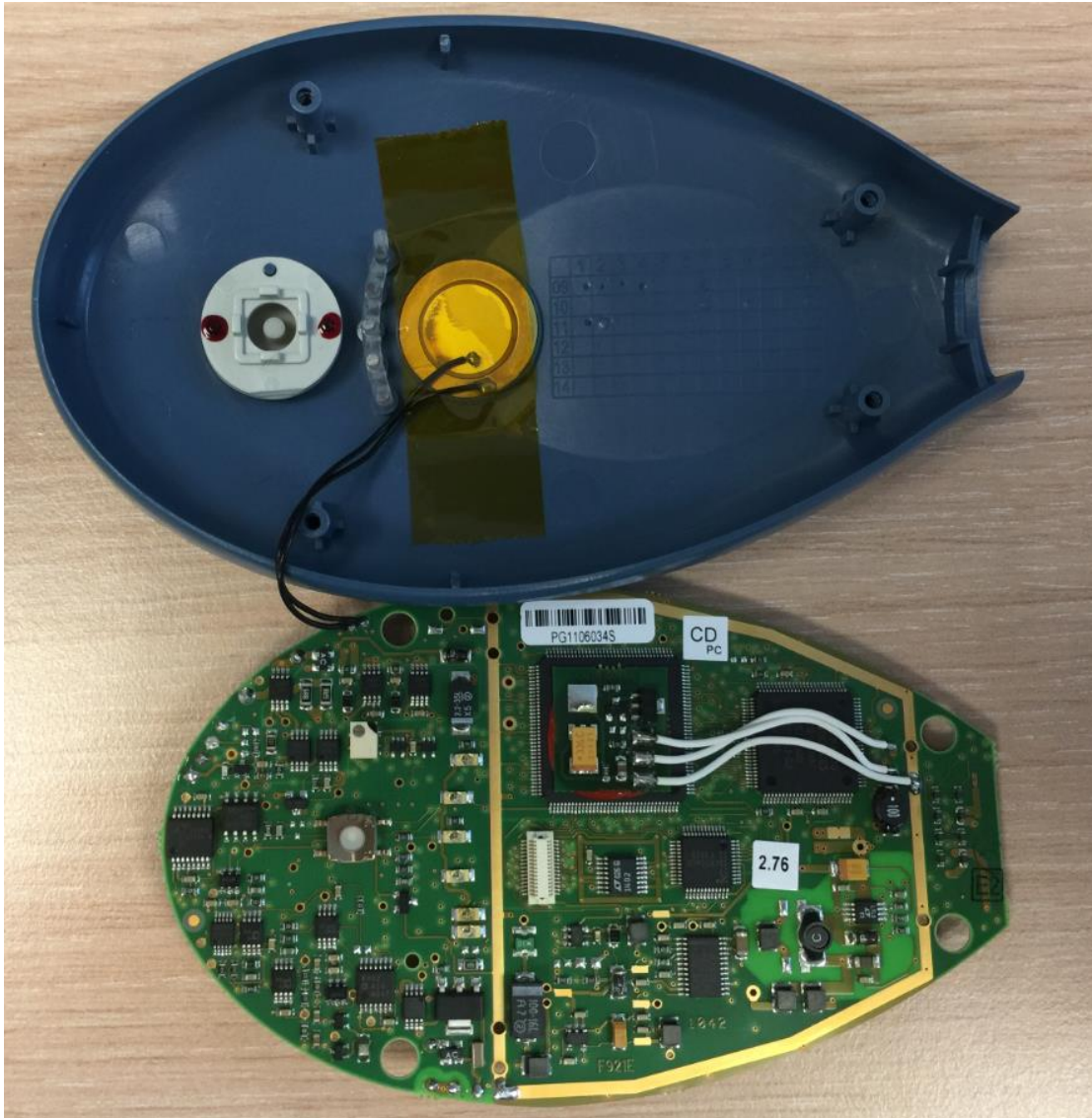
Electronic card top
