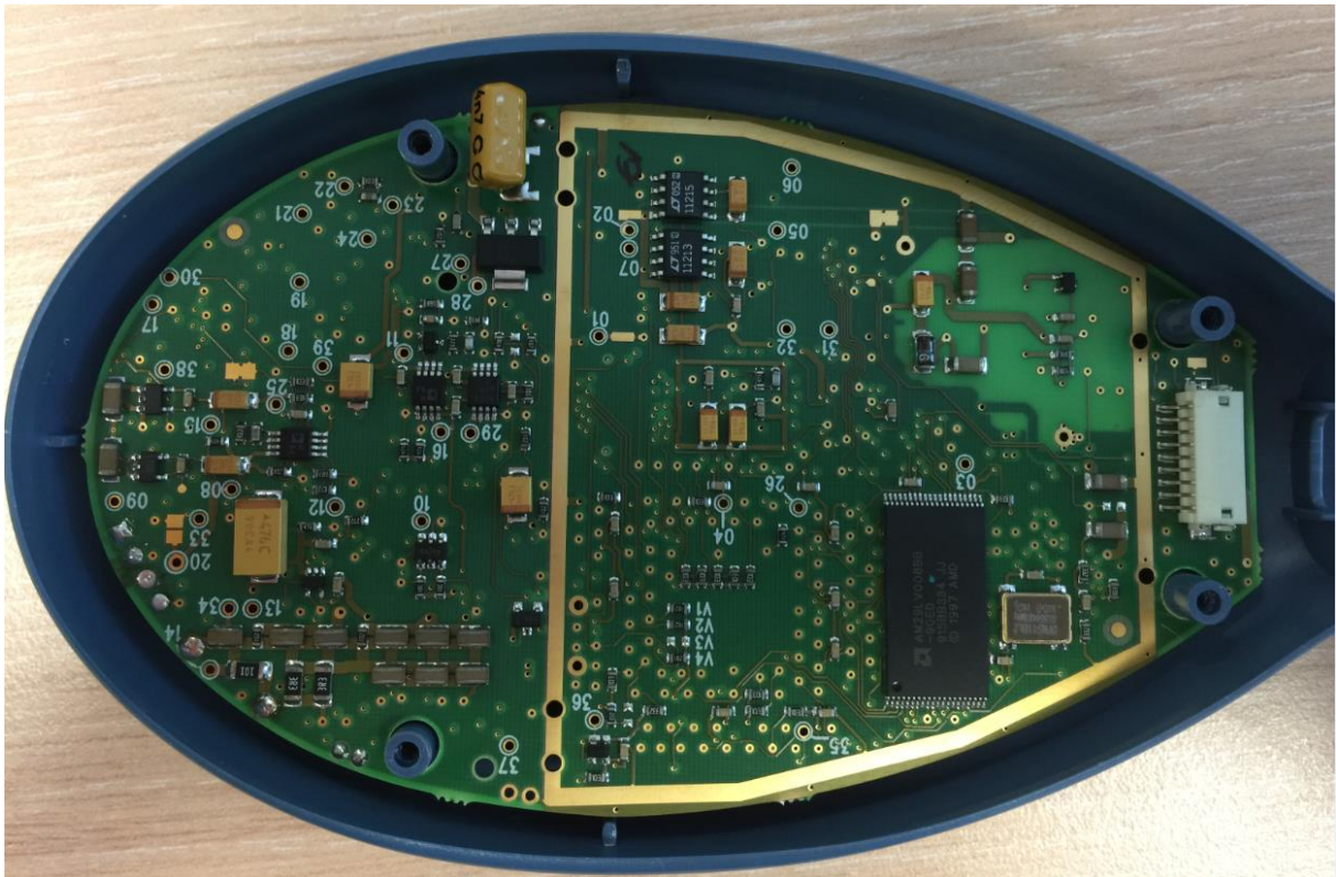
Electronic card bottom
