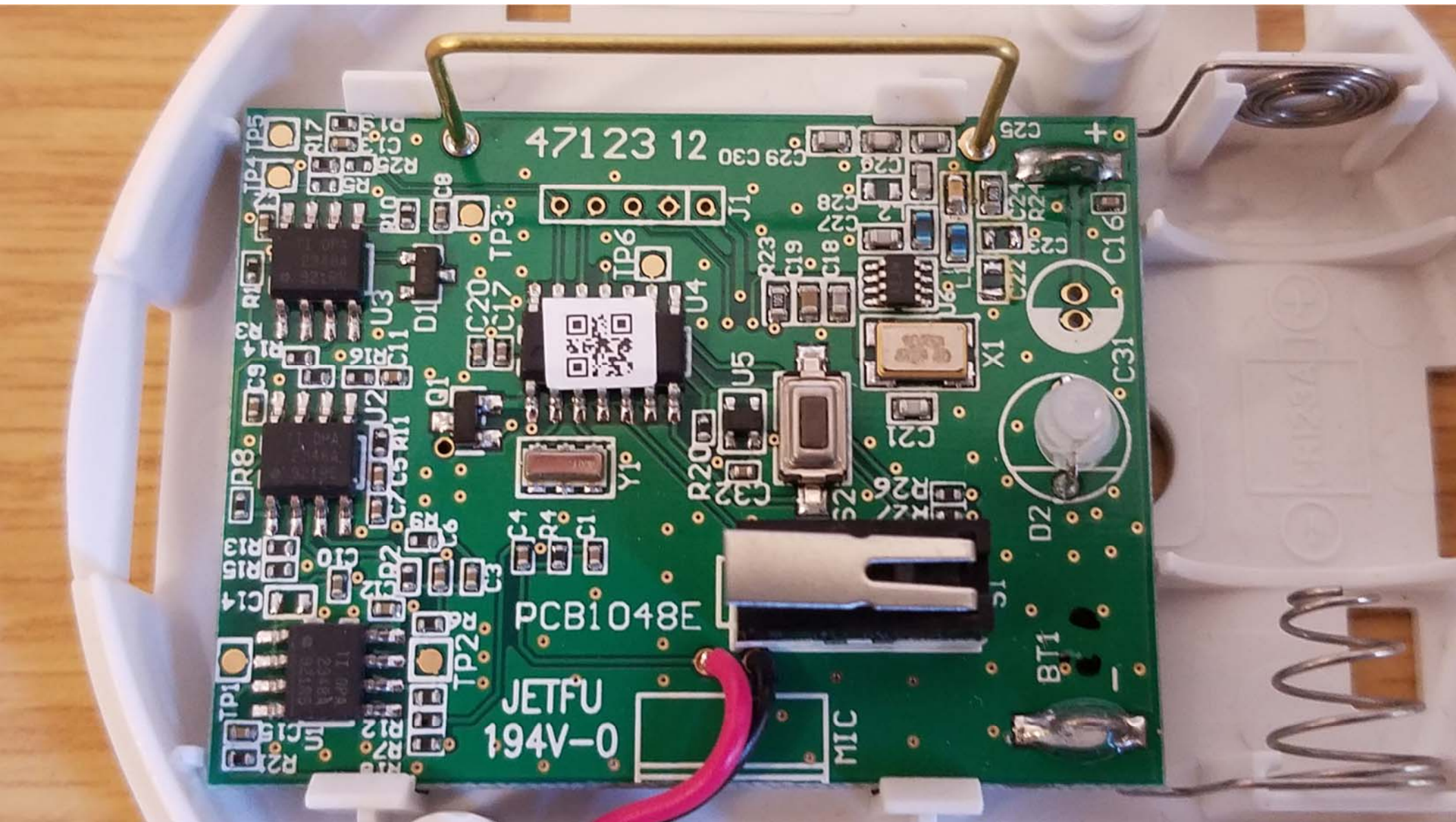
Top View of the PCB - #1
