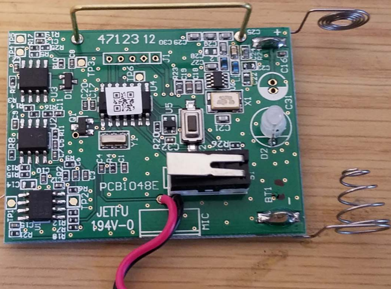
Top View of the PCB - View #2
