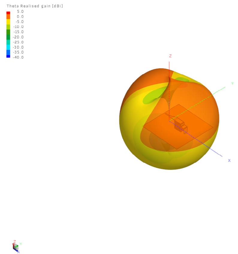
Theta Polarization
