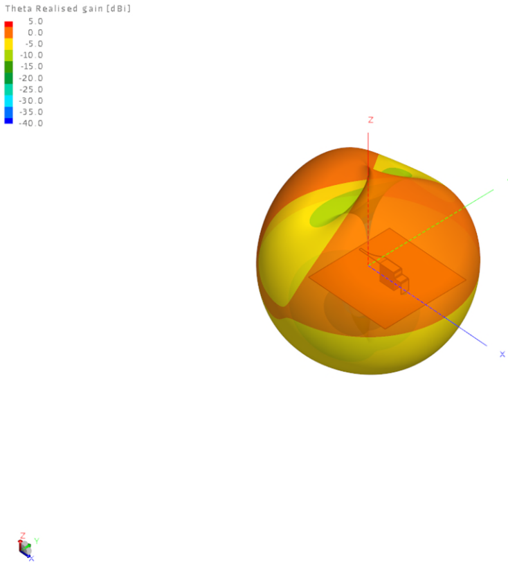
Theta Polarization
