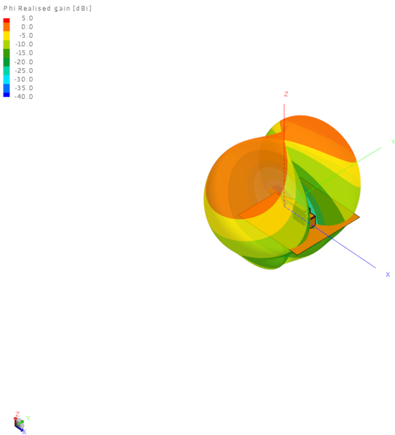
Phi Polarization
