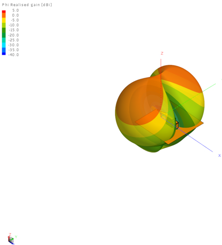
Phi Polarization
