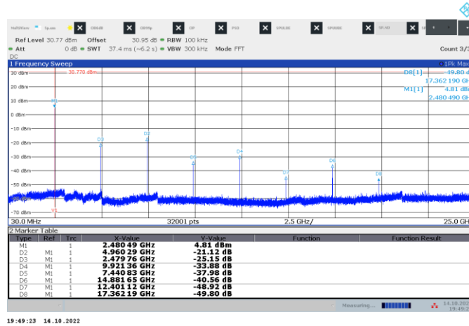
Figure 8.6-7: Conducted spurious emissions outside restricted band, TX on High channel
