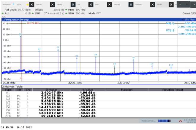
Figure 8.6-5: Conducted spurious emissions outside restricted band, TX on Low channel
