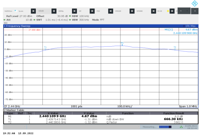
Figure 8.4-2: 6 dB bandwidth on BLE, Tx mid channel
