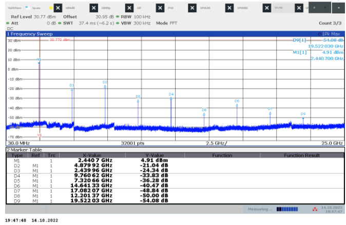
Figure 8.6-6: Conducted spurious emissions outside restricted band, TX on Mid channel
