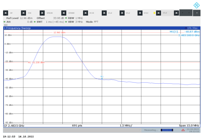
Figure 8.6-2: Conducted spurious emissions at band edge within restricted band, TX on High channel, Peak
