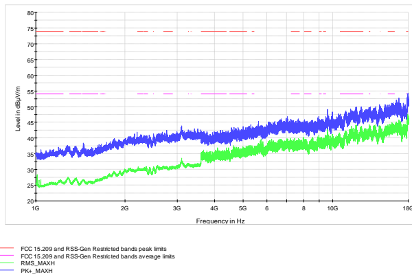
Figure 8.6-9: Radiated spurious emissions 1 GHz to 18 GHz – Sample plot
