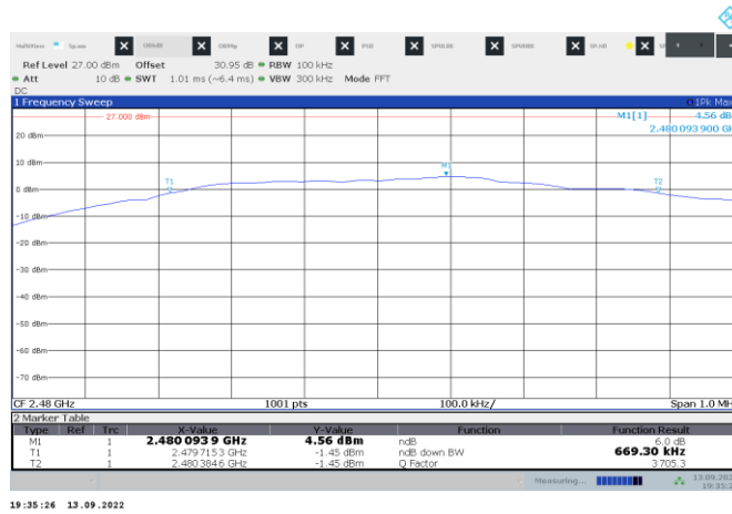
Figure 8.4-3: 6 dB bandwidth on BLE, Tx high channel
