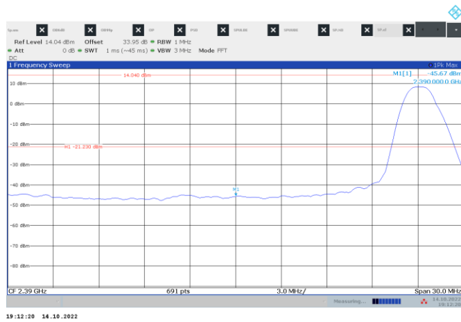
Figure 8.6-1: Conducted spurious emission at band edge within restricted band, TX on low channel, Peak
