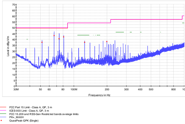
Figure 8.6-8: Radiated spurious emissions 30 MHz to 1 GHz – Sample plot
