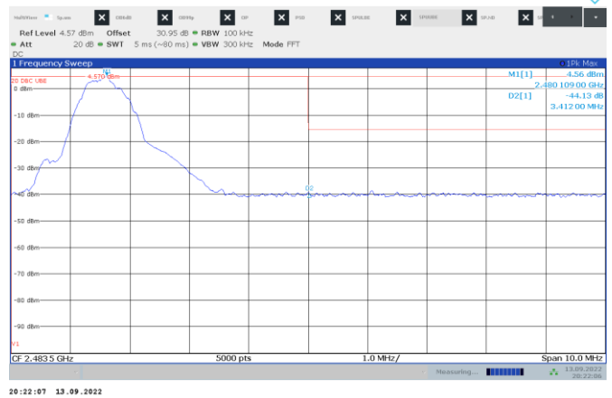
Figure 8.6-4: Conducted spurious emissions at band edge outside restricted band, TX on High channel
