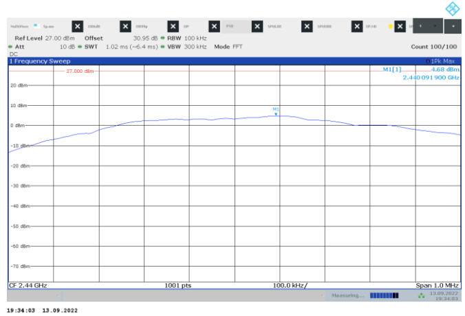
Figure 8.7-2: PSD on mid channel
