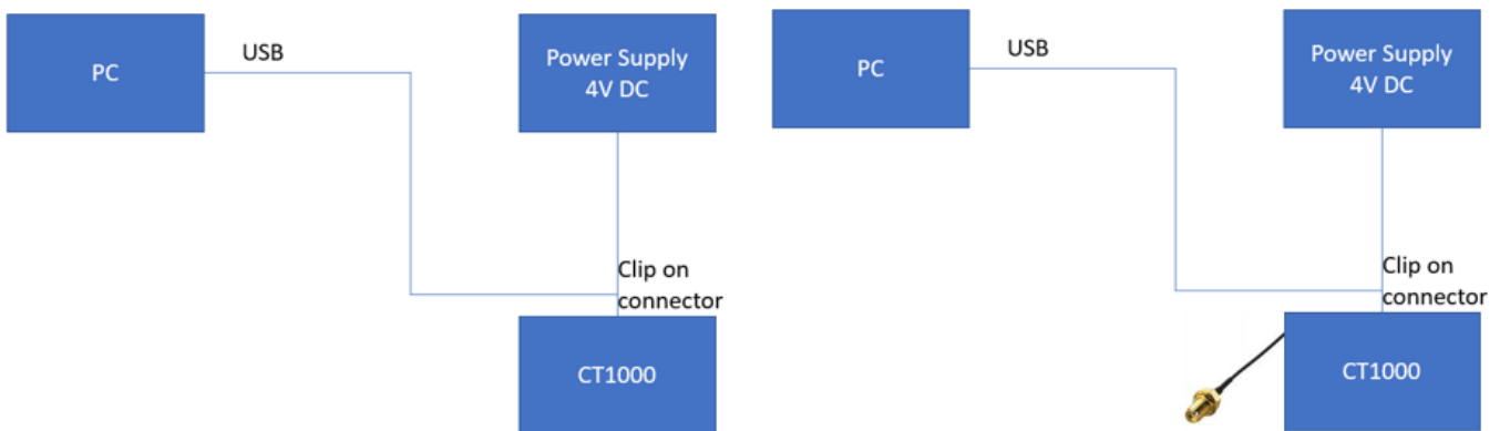
Figure 5.5-1: Radiated testing block diagram (Left) and Antenna port testing block diagram (Right)
