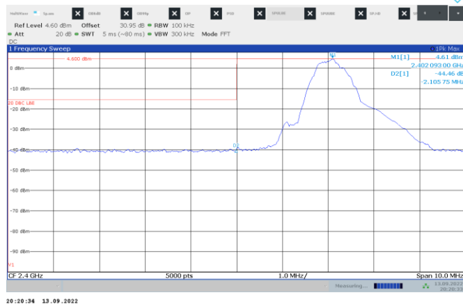
Figure 8.6-3: Conducted spurious emission at band edge outside restricted band, TX on low channel
