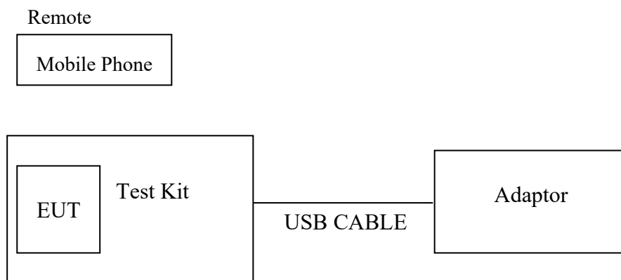
Fig. 2-2 Configuration (CE)
