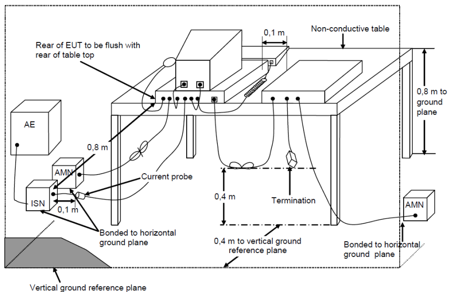
Measurement set up for AC Wireline Conducted Emissions Test
