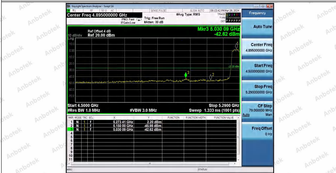
11AC40MIMO_Ant1_High_5310
