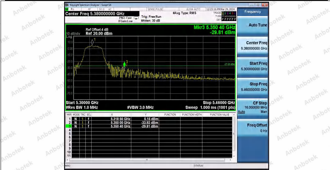
11AC20MIMO_Ant2_High_5320
