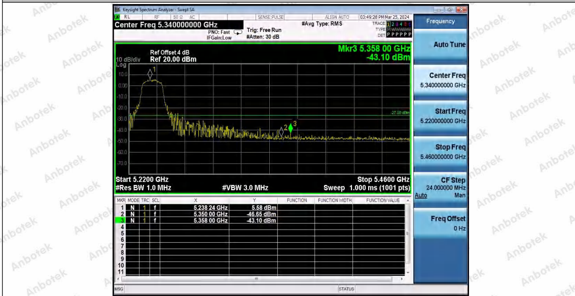
11AC20MIMO_Ant2_High_5240
