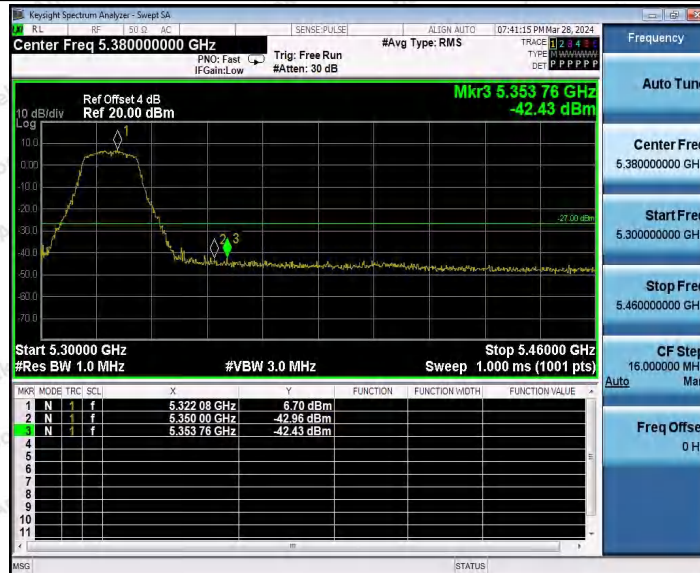
11A_Ant2_High_5320
