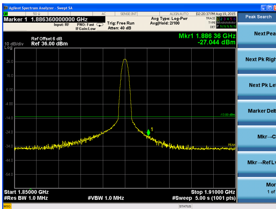
Channel 661, 1850MHz~1910MHz
