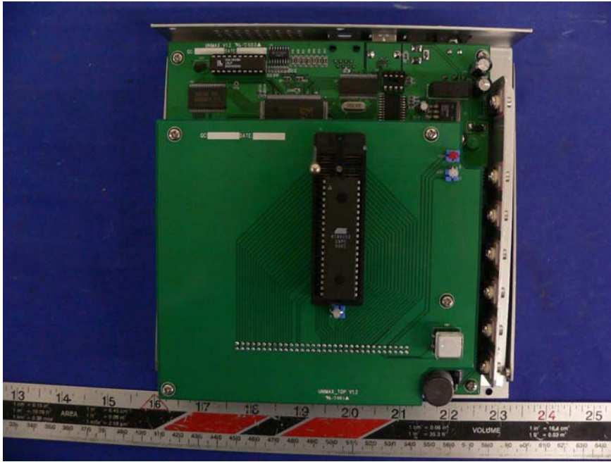
EUT – Chassis off View
