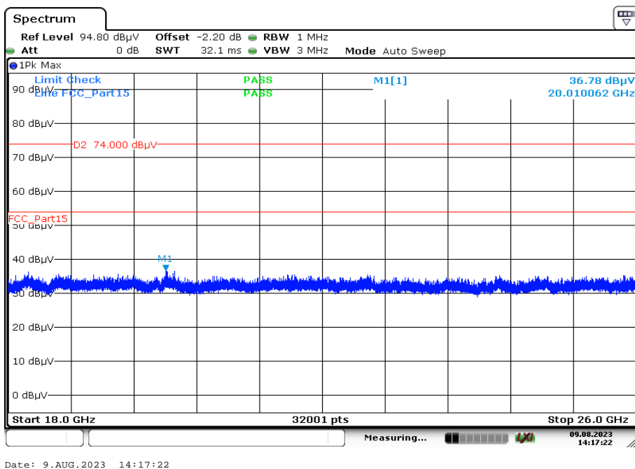
Plot 4: 18 GHz to 26 GHz, TX mode, 2440 MHz, vertical & horizontal polarization, 1 Msp
