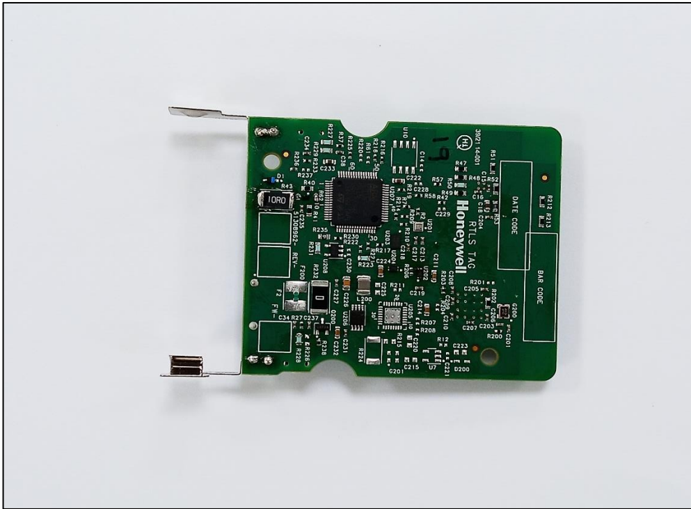
Figure 3: Front view of the PCB
