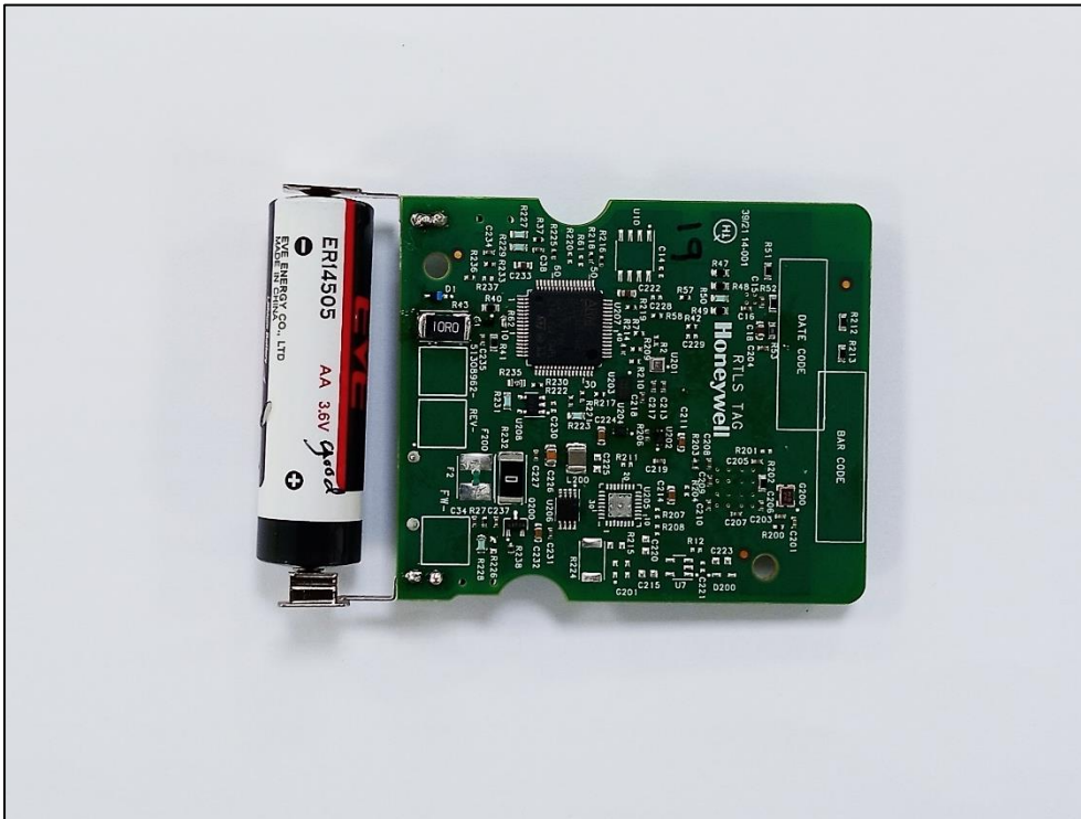
Figure 5: Front view of the PCB with 3.6V Battery
