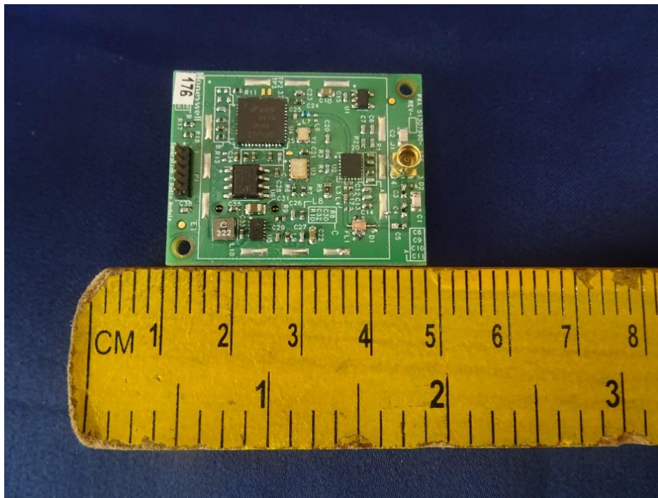
Photo 5: RF module dimensional view width)
