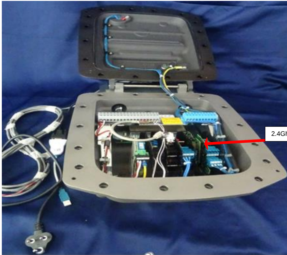
Photo 1: EUT with Top Encloser open
