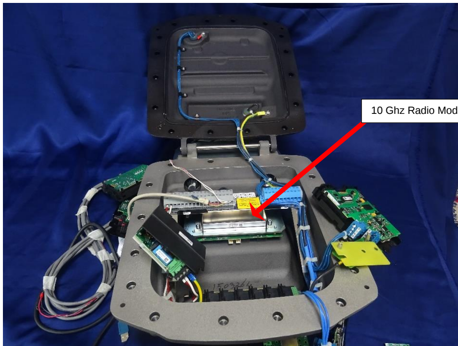
Photo 2: EUT showing with all PCB's removed
