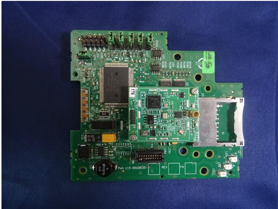
Photo 1: EUT PCB Front view
