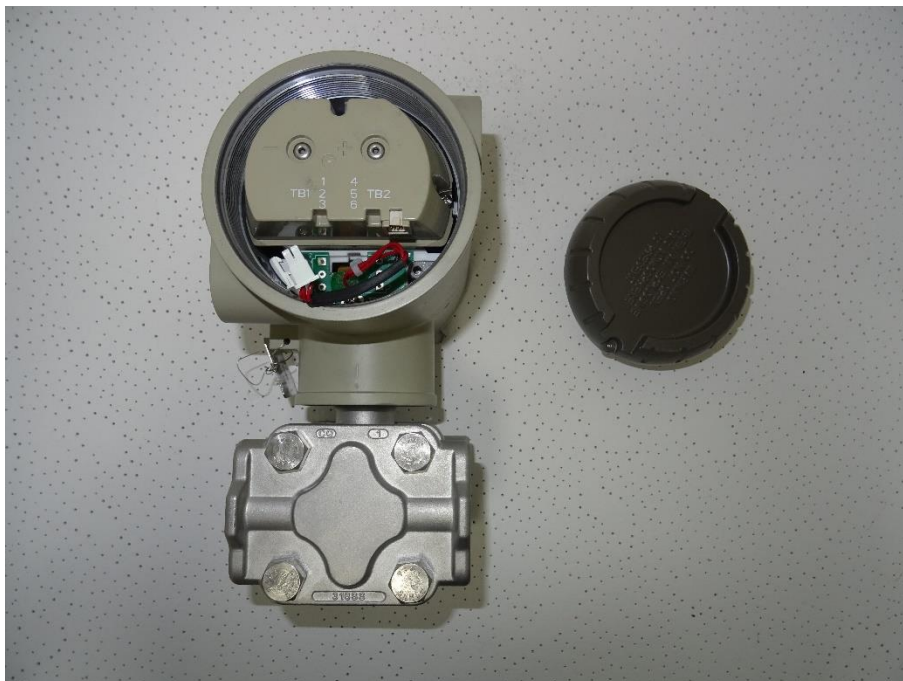
Photo 4: Rear panel removed from the host device
