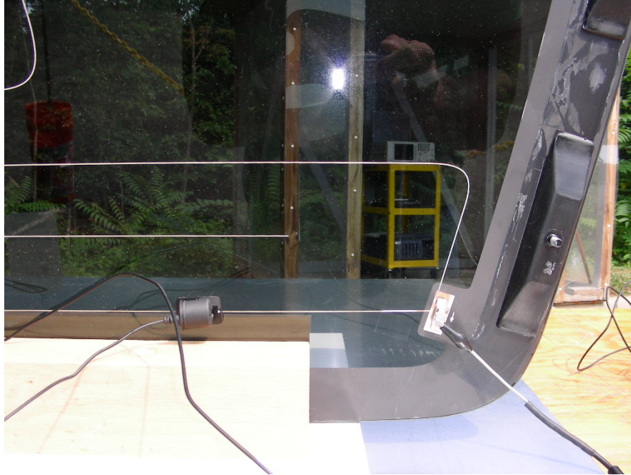
Figure 1-9. SureConnect with Glass Antenna Set-up – Test Configuration #7
