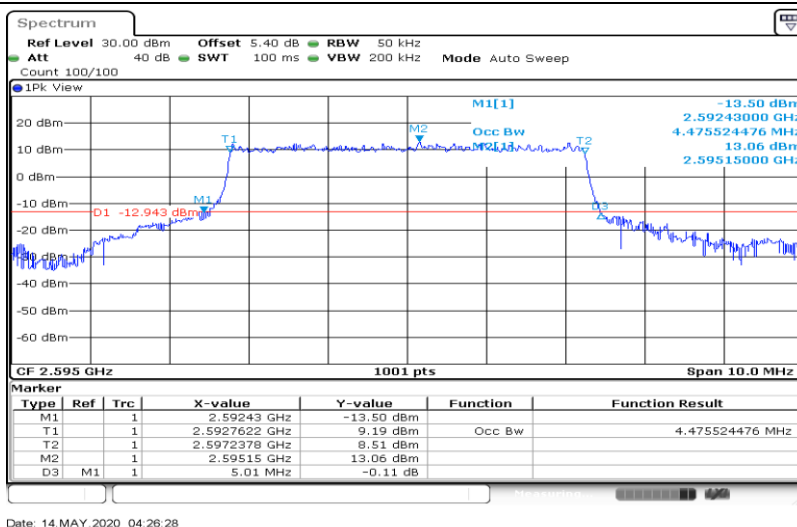
Band38-5MHz-16QAM-38225-25RB#0-4.476
