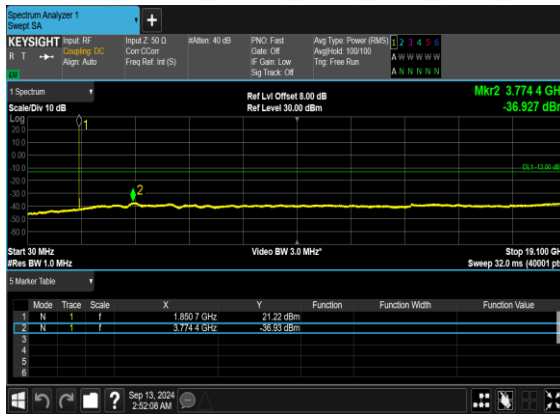
N2(10M)_DFT-s- OFDM_BPSK_Edge_1RB_Left_Low_CH
