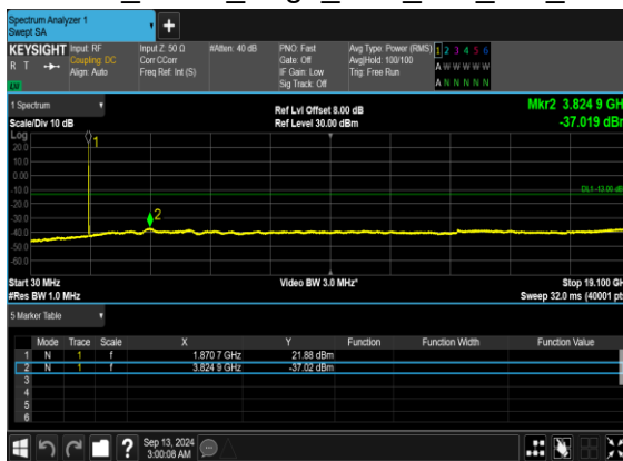
N2(20M)_DFT-s- OFDM_BPSK_Edge_1RB_Left_Mid_CH
