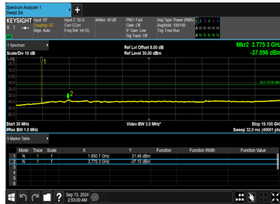
N2(10M)_DFT-s- OFDM_QPSK_Edge_1RB_Left_Low_CH
