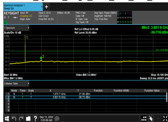
N2(20M)_DFT-s- OFDM_QPSK_Edge_1RB_Left_Mid_CH
