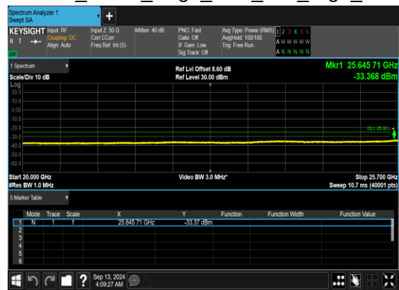
N7(20M)_DFT-s- OFDM_BPSK_Edge_1RB_Left_High_CH
