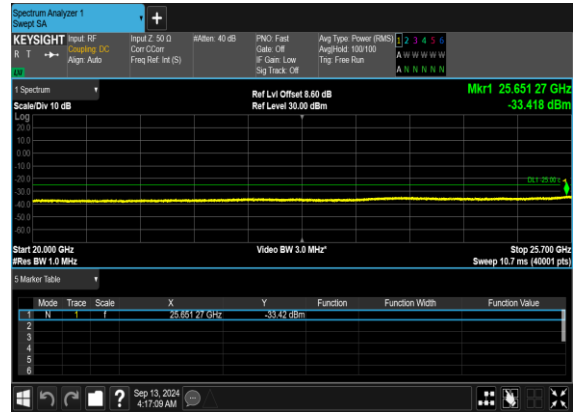
N7(40M)_DFT-s- OFDM_QPSK_Edge_1RB_Left_Mid_CH
