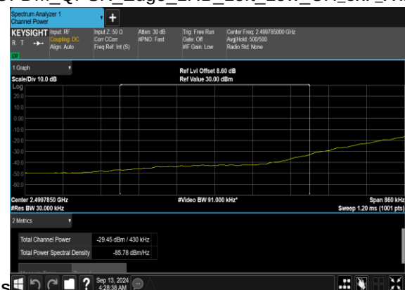
N7(20M)_DFT-s- OFDM_QPSK_Edge_1RB_Left_Low_CH_CHP_PAS
