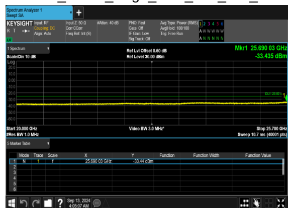
N7(20M)_DFT-s- OFDM_BPSK_Edge_1RB_Left_Mid_CH
